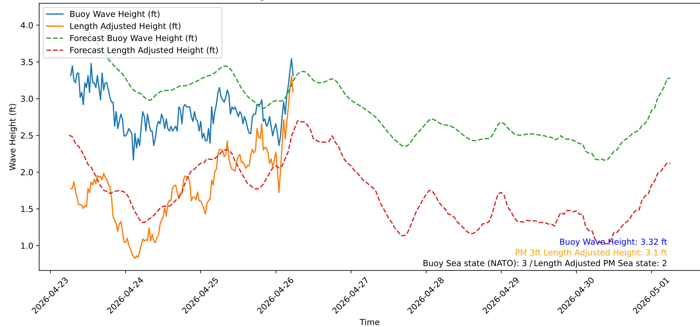
Wave Heights over Time for Red Beach at 2026-04-26 06:10:50
