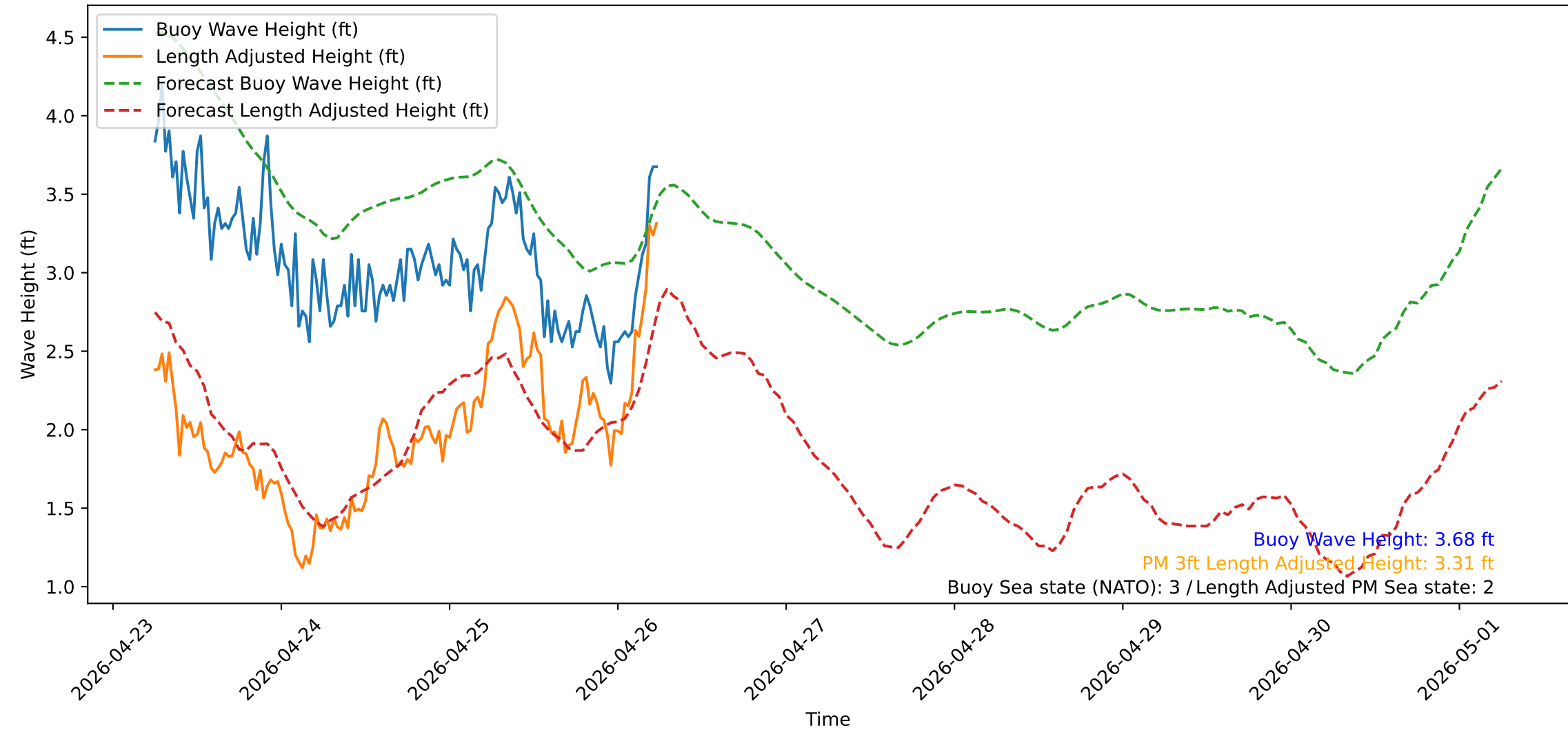
Wave Heights over Time for Oceanside Harbor at 2026-04-26 06:10:31
