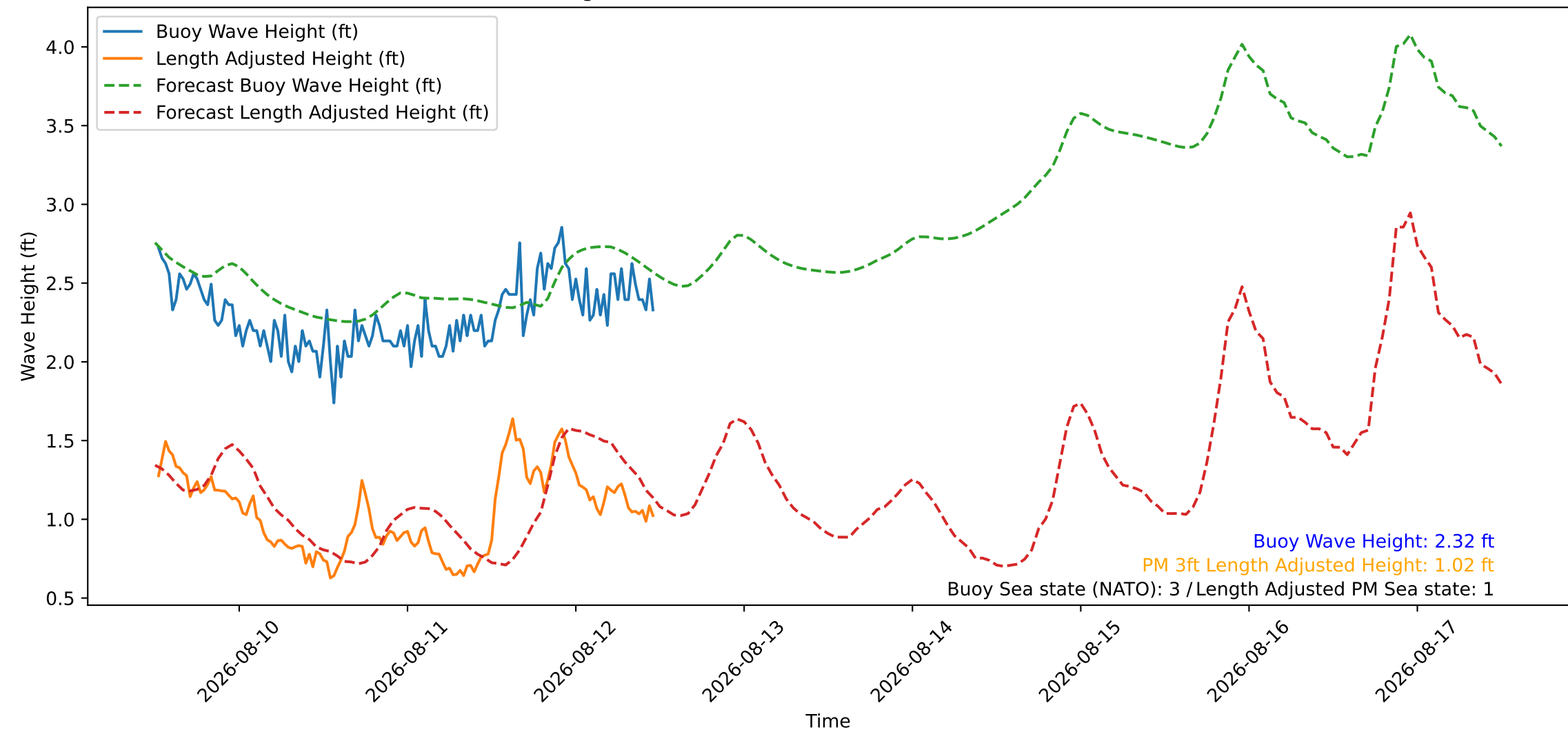
Wave Heights over Time for Red Beach at 2026-08-12 12:00:45
