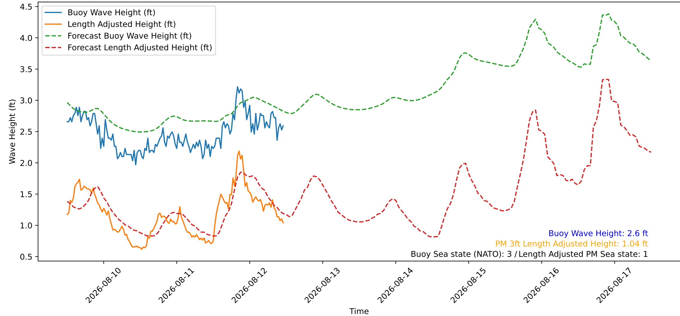
Wave Heights over Time for Green Beach at 2026-08-12 12:01:08
