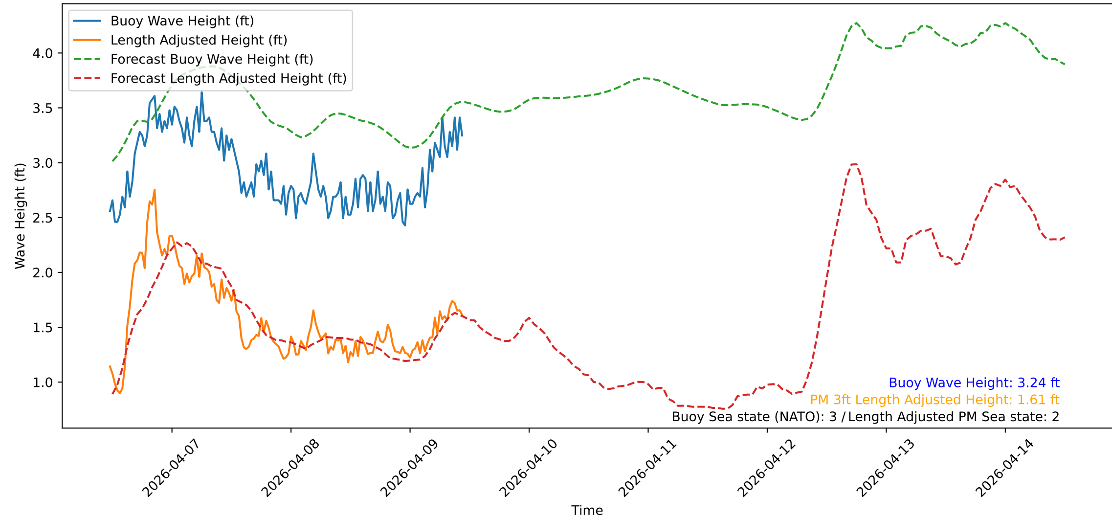
Wave Heights over Time for Oceanside Harbor at 2026-04-09 11:30:31
