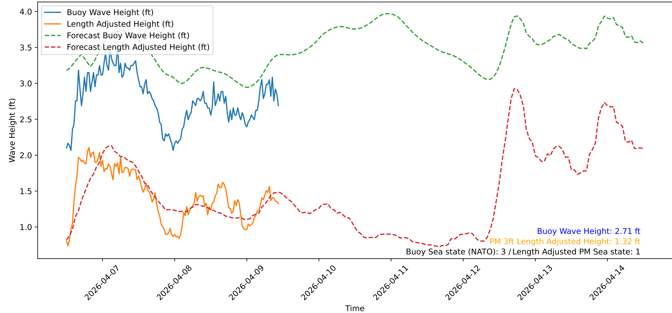
Wave Heights over Time for Red Beach at 2026-04-09 11:30:47
