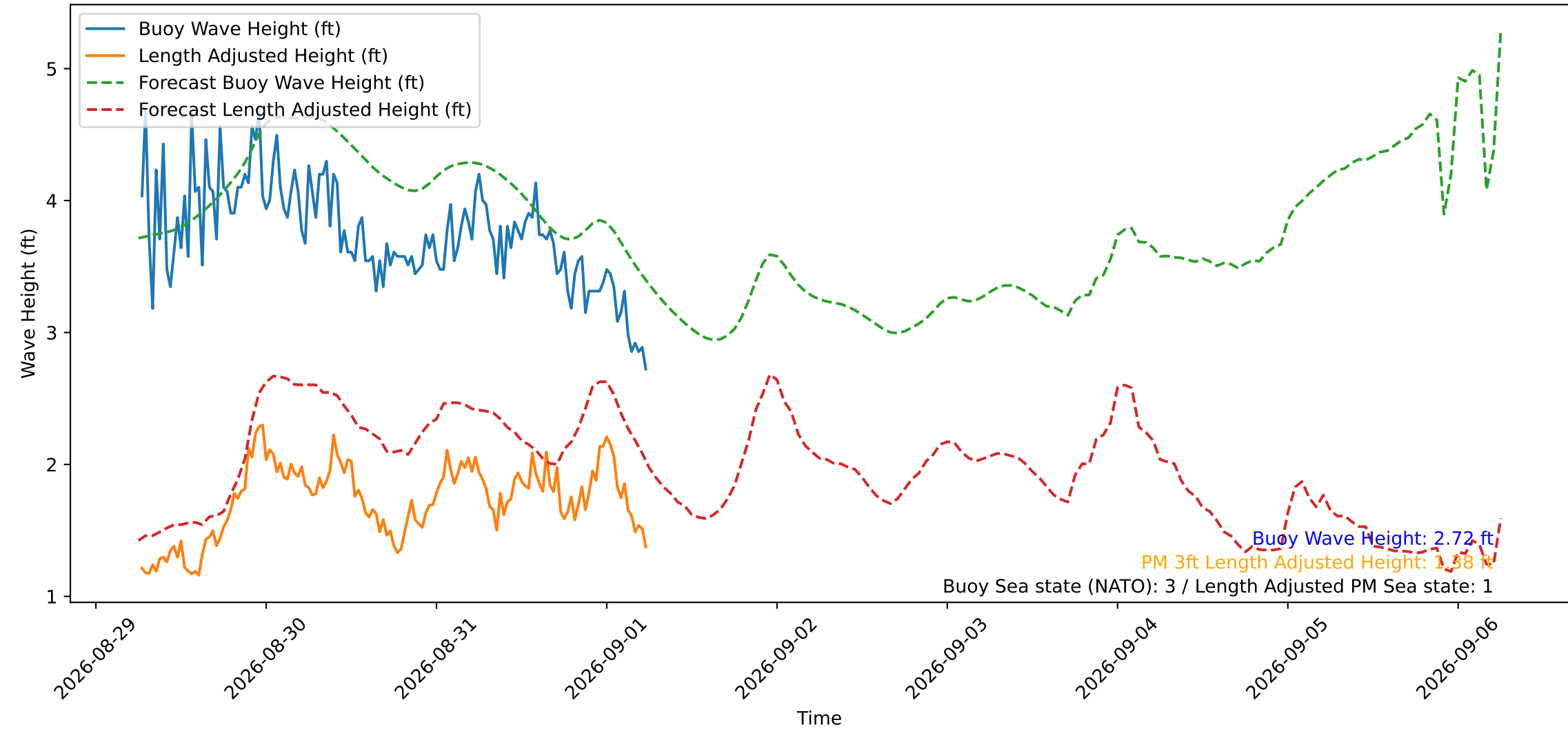
Wave Heights over Time for Red Beach at 2026-09-01 06:20:51
