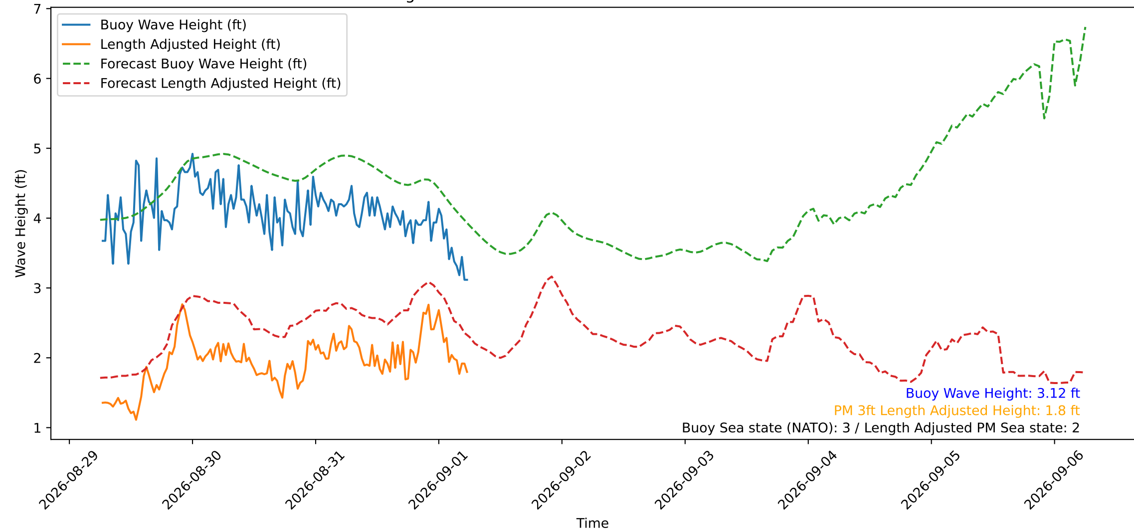
Wave Heights over Time for Green Beach at 2026-09-01 06:21:14
