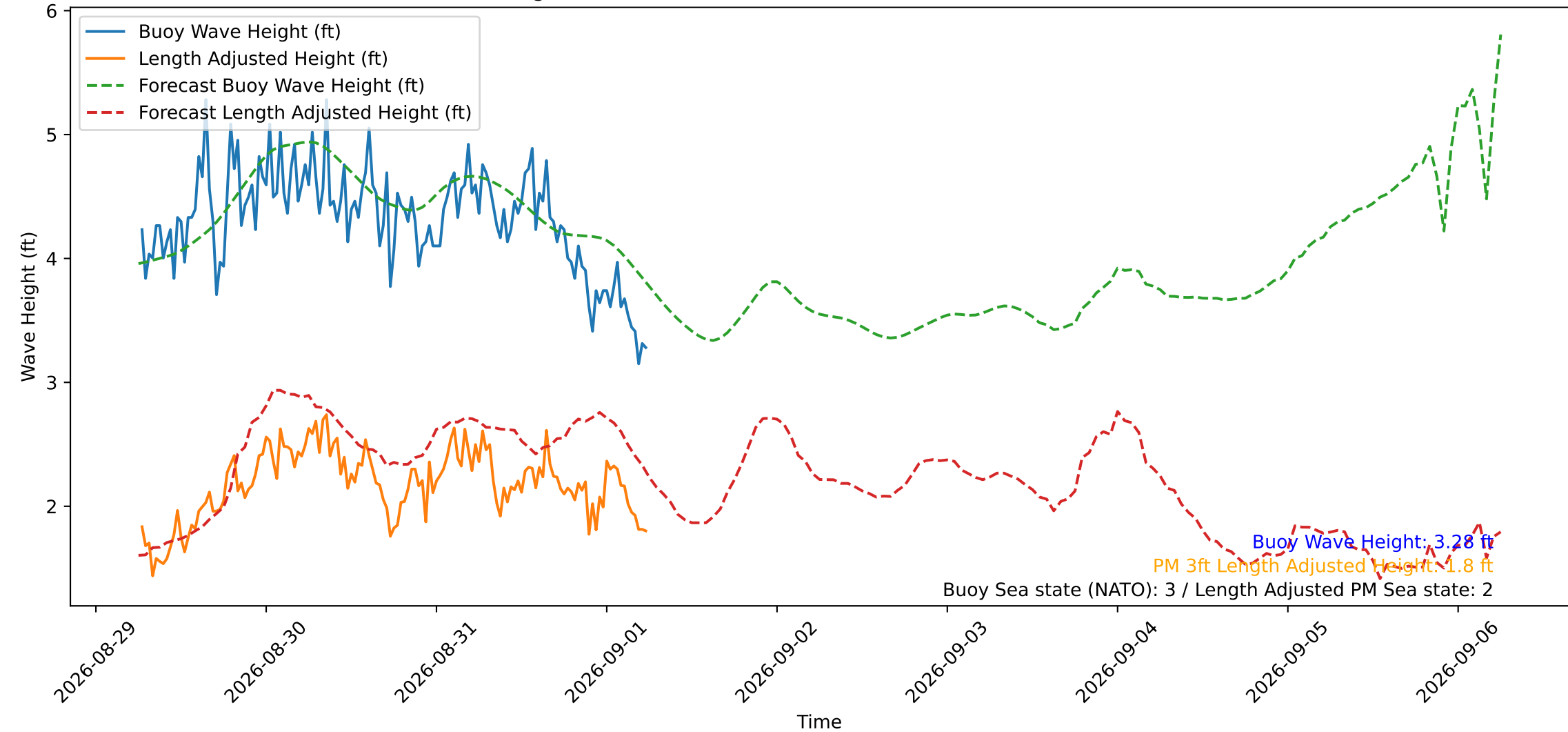
Wave Heights over Time for Oceanside Harbor at 2026-09-01 06:20:30
