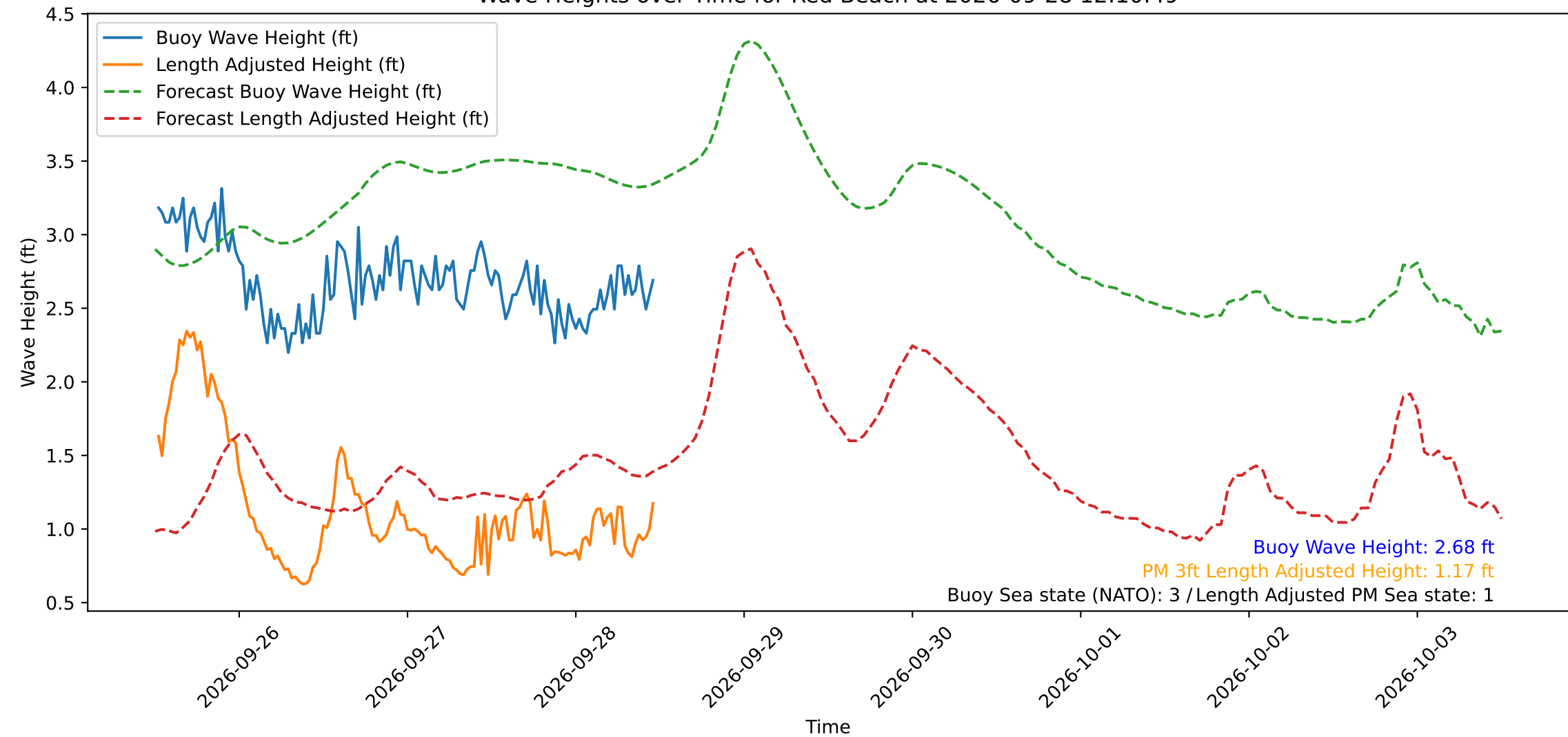
Wave Heights over Time for Red Beach at 2026-09-28 12:10:49
