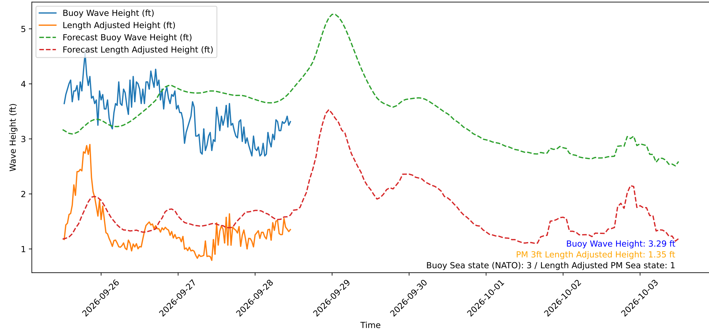
Wave Heights over Time for Green Beach at 2026-09-28 12:11:12
