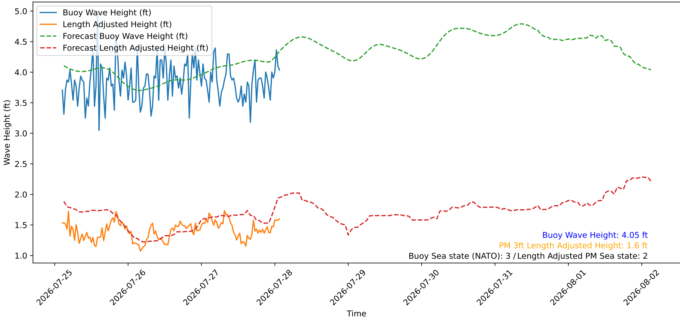
Wave Heights over Time for Oceanside Harbor at 2026-07-28 02:30:26
