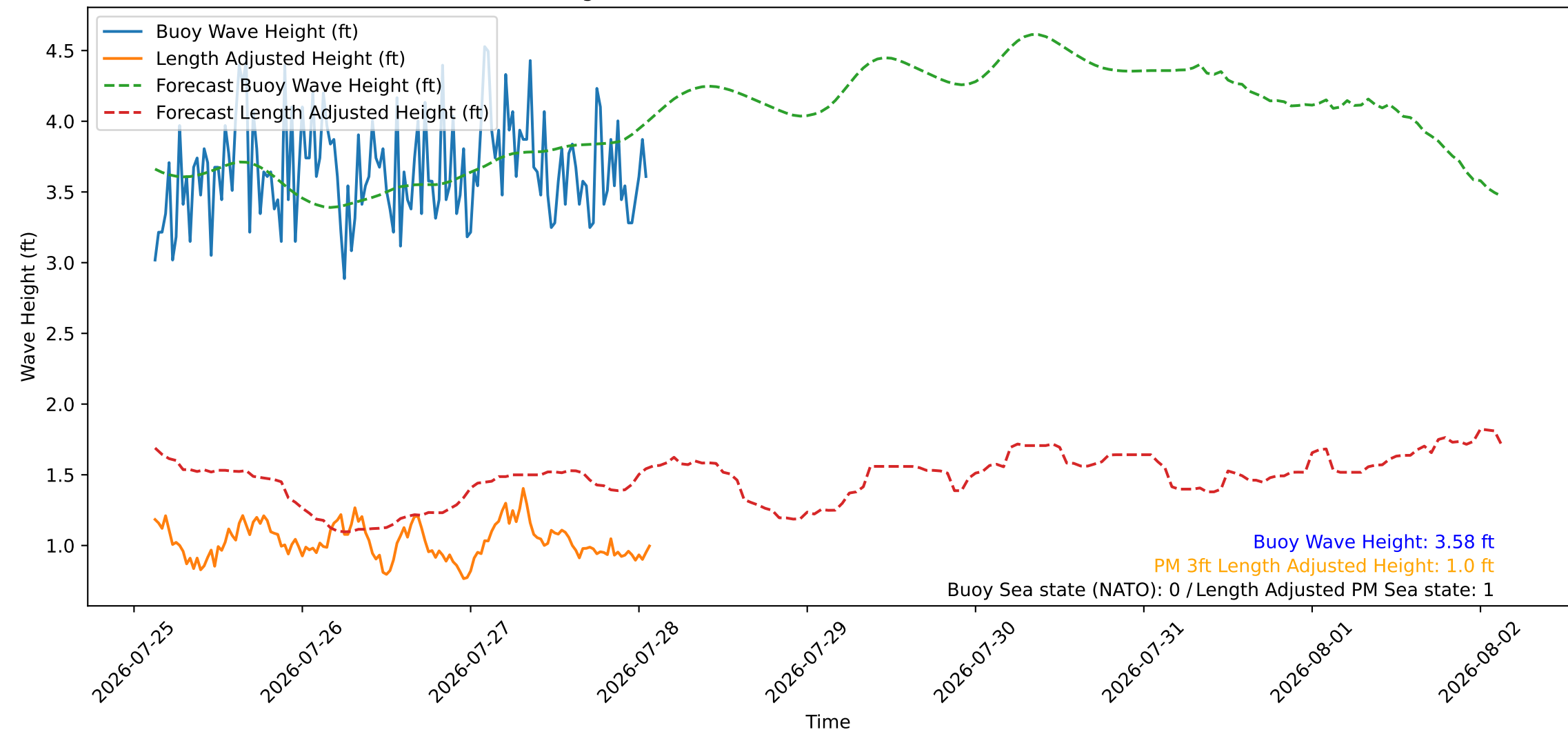
Wave Heights over Time for Red Beach at 2026-07-28 02:30:46
