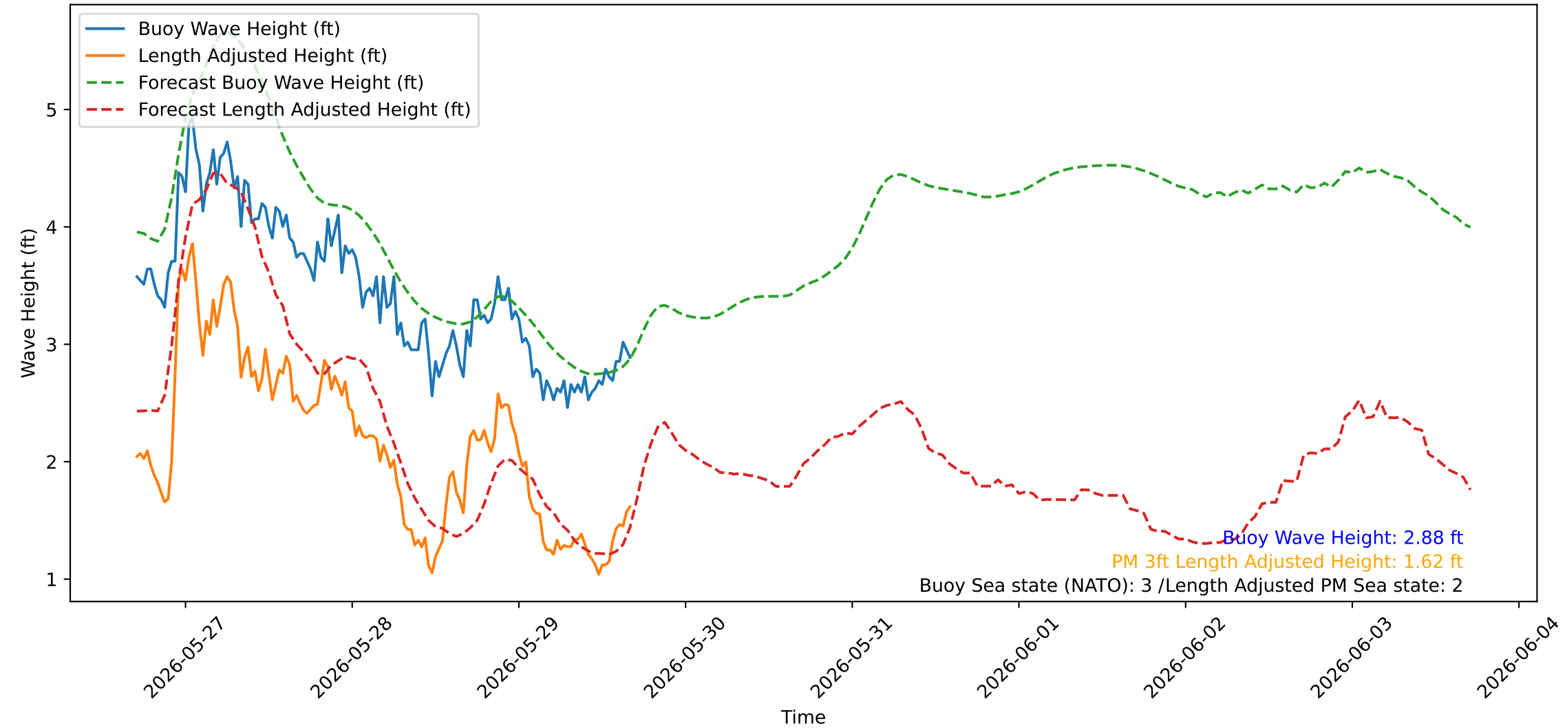
Wave Heights over Time for Green Beach at 2026-05-29 16:51:06
