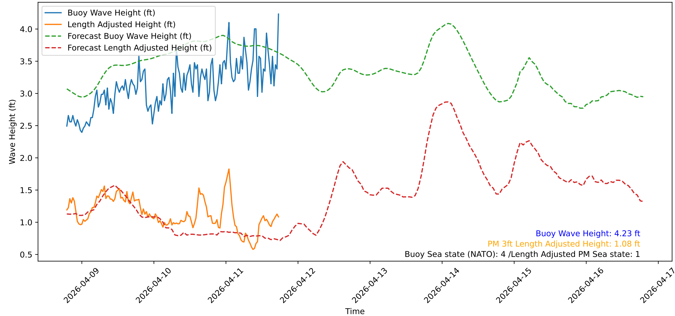
Wave Heights over Time for Red Beach at 2026-04-11 18:30:51
