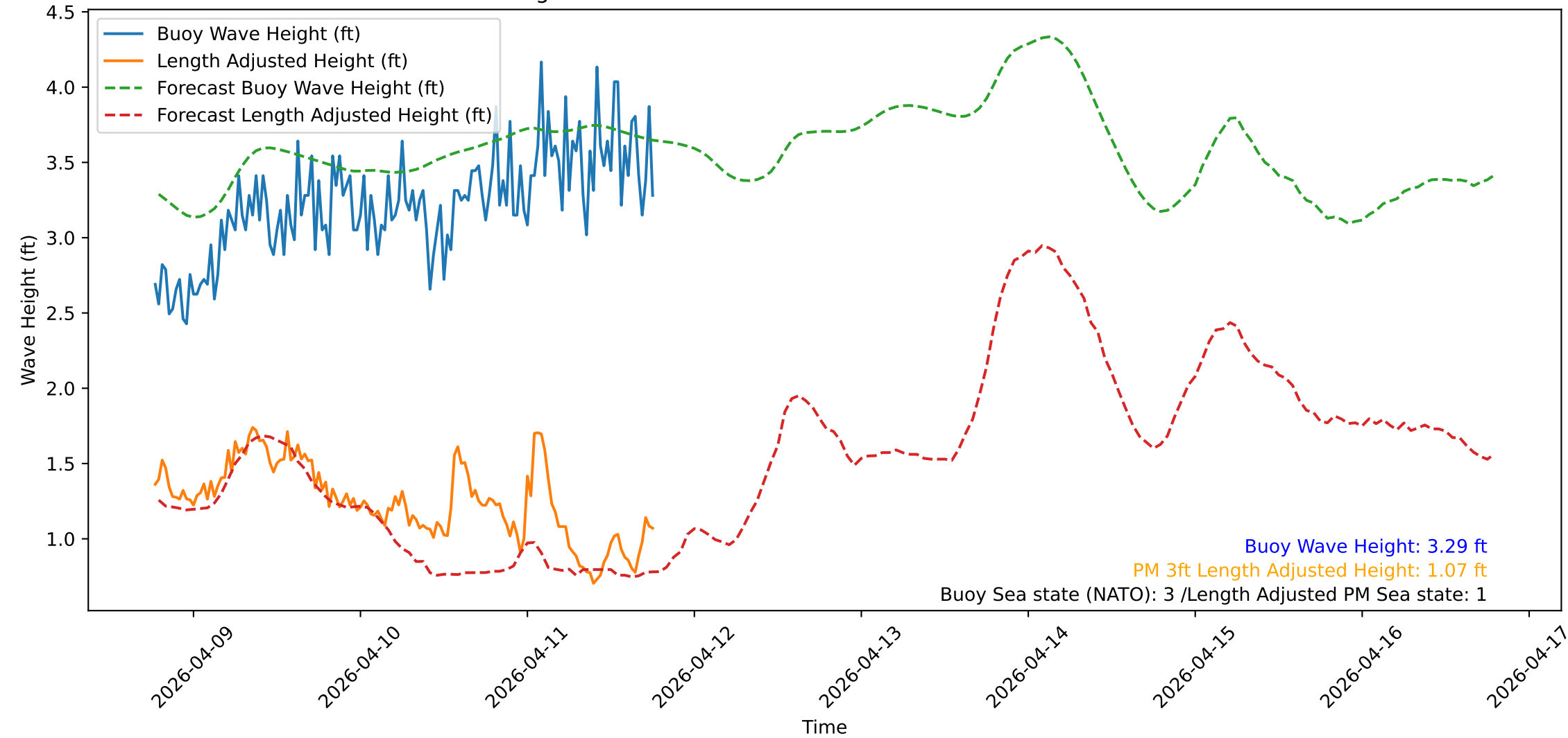
Wave Heights over Time for Oceanside Harbor at 2026-04-11 18:30:32
