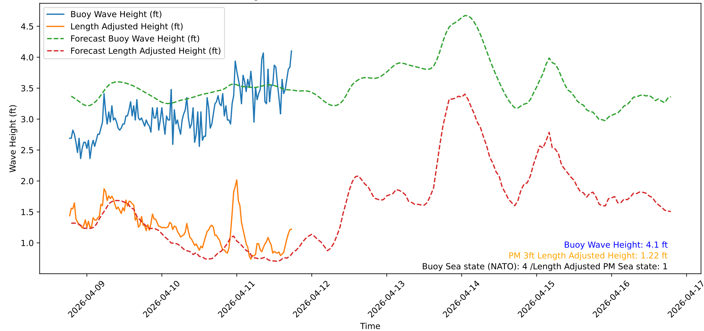
Wave Heights over Time for Green Beach at 2026-04-11 18:31:13
