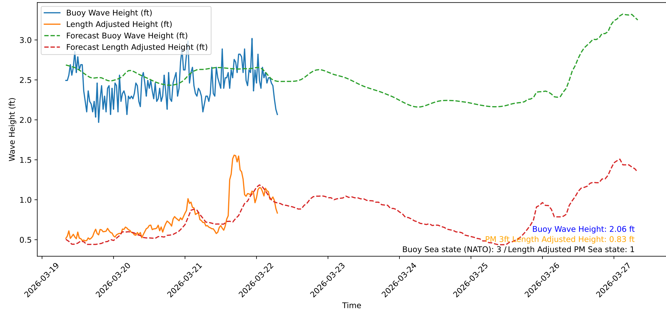
Wave Heights over Time for Oceanside Harbor at 2026-03-22 08:00:31
