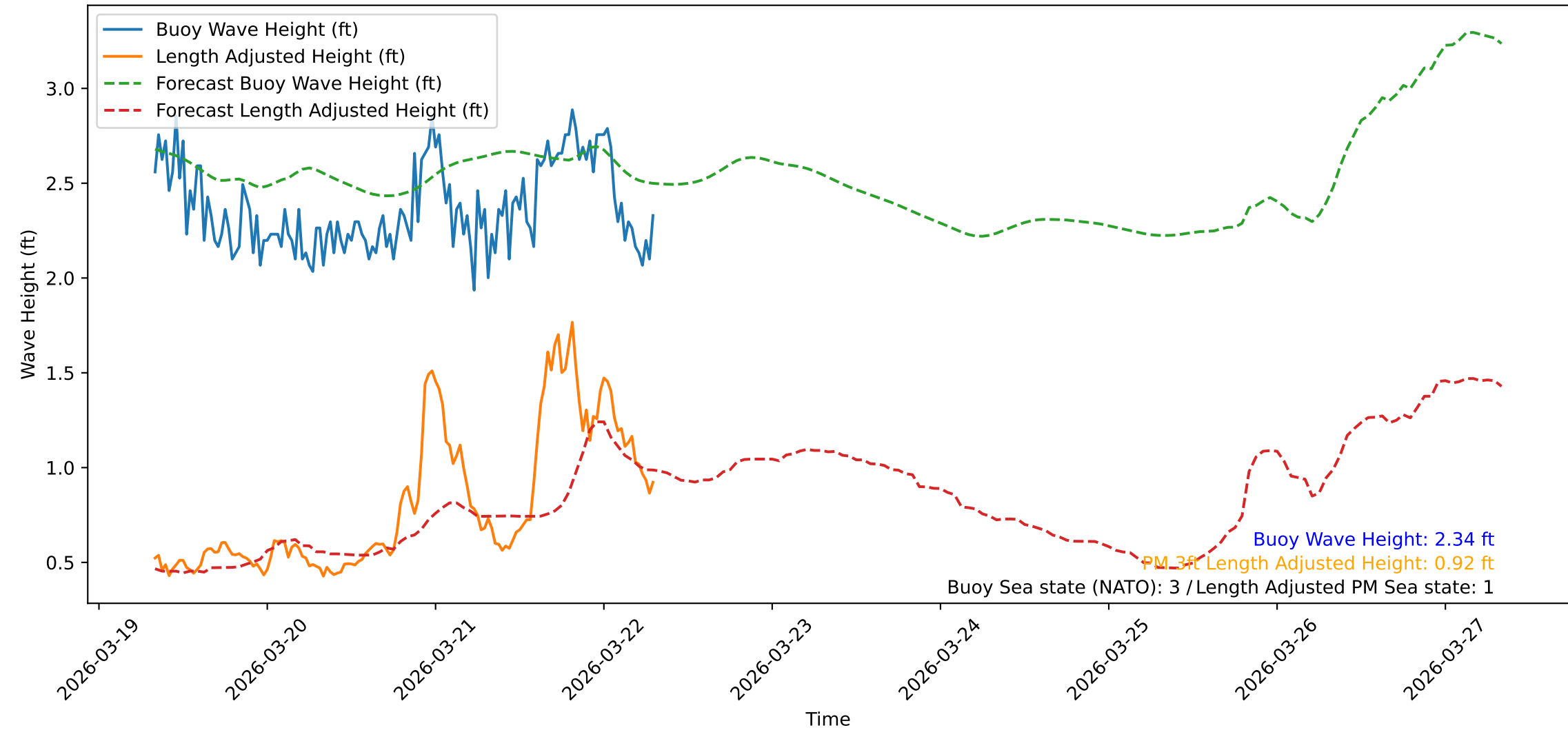
Wave Heights over Time for Green Beach at 2026-03-22 08:01:10
