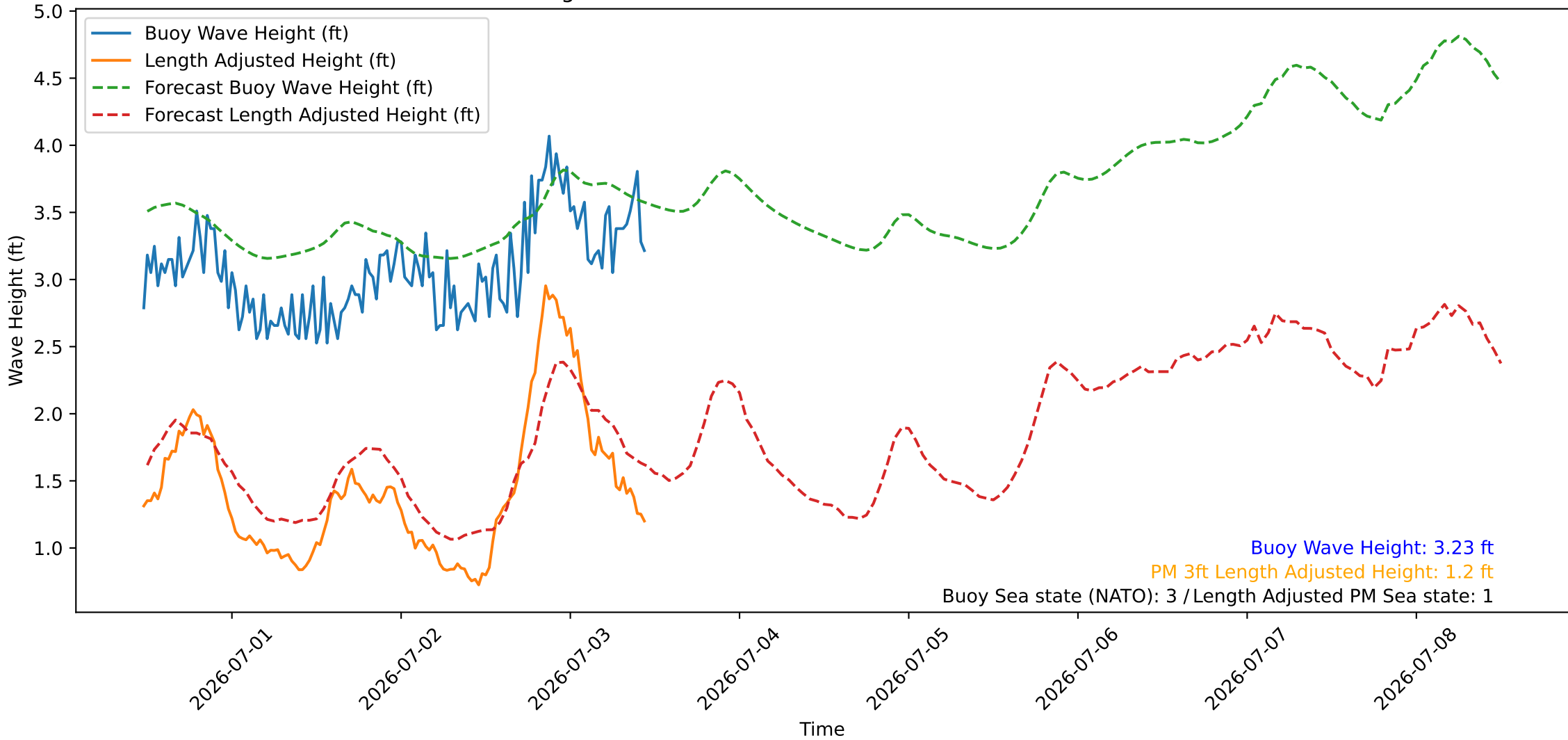
Wave Heights over Time for Green Beach at 2026-07-03 11:31:08
