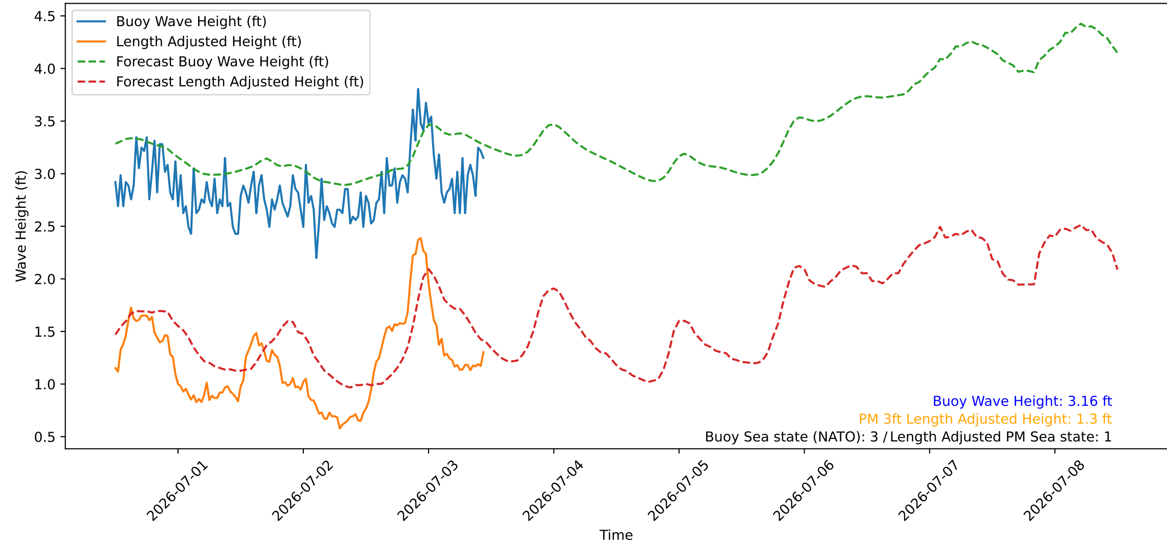
Wave Heights over Time for Red Beach at 2026-07-03 11:30:45
