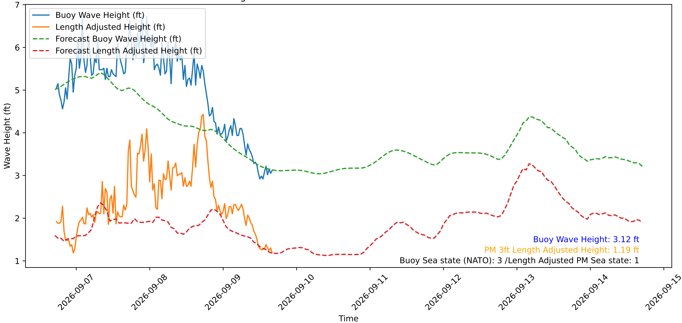
Wave Heights over Time for Red Beach at 2026-09-09 17:00:49
