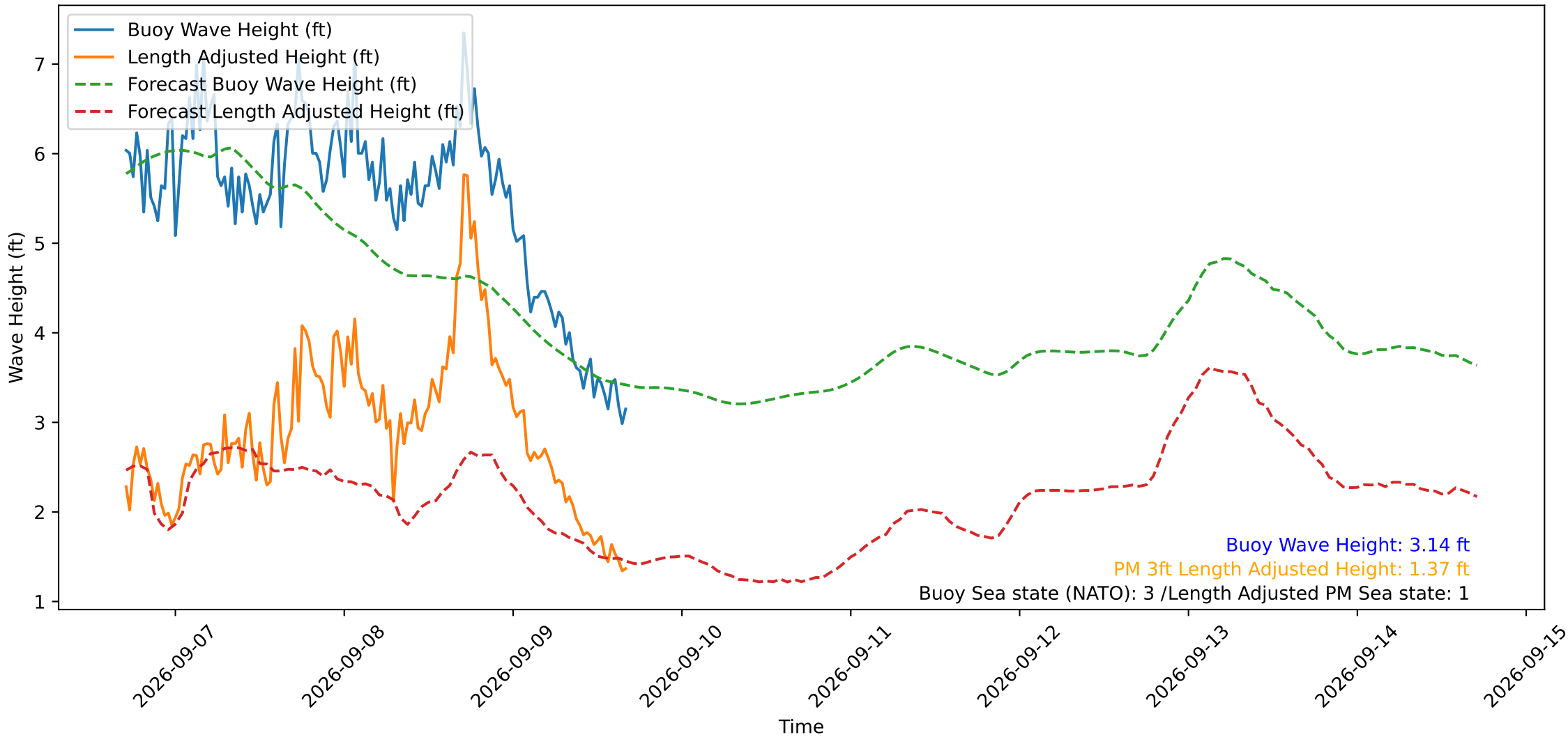
Wave Heights over Time for Oceanside Harbor at 2026-09-09 17:00:29
