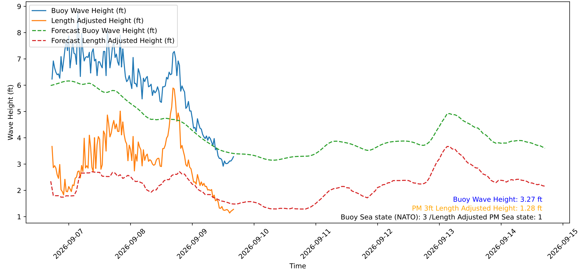
Wave Heights over Time for Green Beach at 2026-09-09 17:01:12
