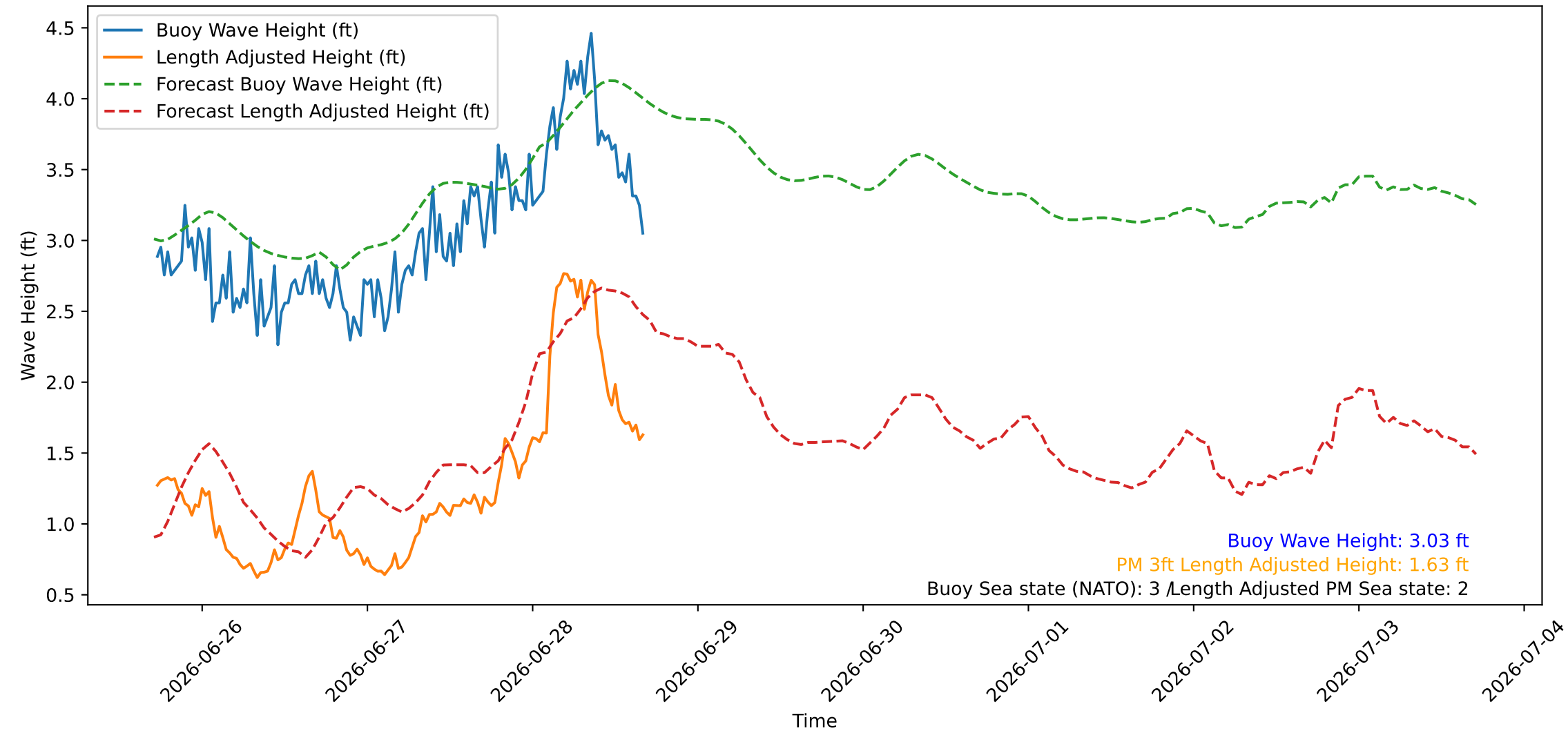
Wave Heights over Time for Red Beach at 2026-06-28 17:00:45
