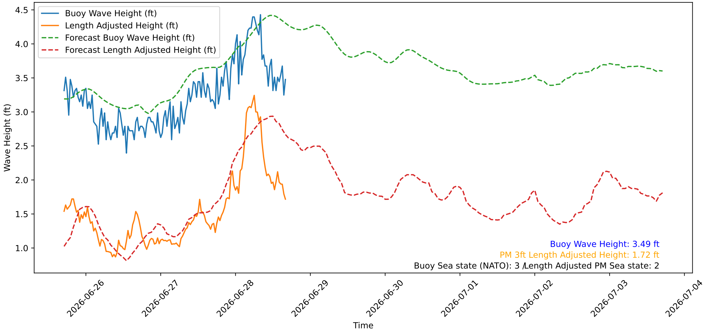
Wave Heights over Time for Oceanside Harbor at 2026-06-28 17:00:26
