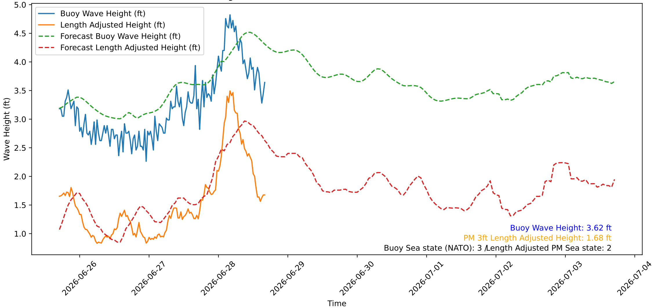
Wave Heights over Time for Green Beach at 2026-06-28 17:01:07
