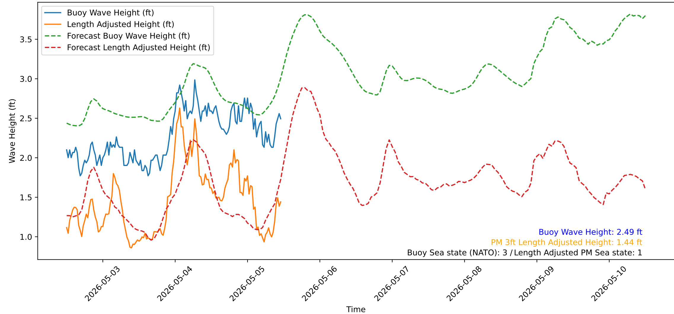
Wave Heights over Time for Green Beach at 2026-05-05 11:51:18
