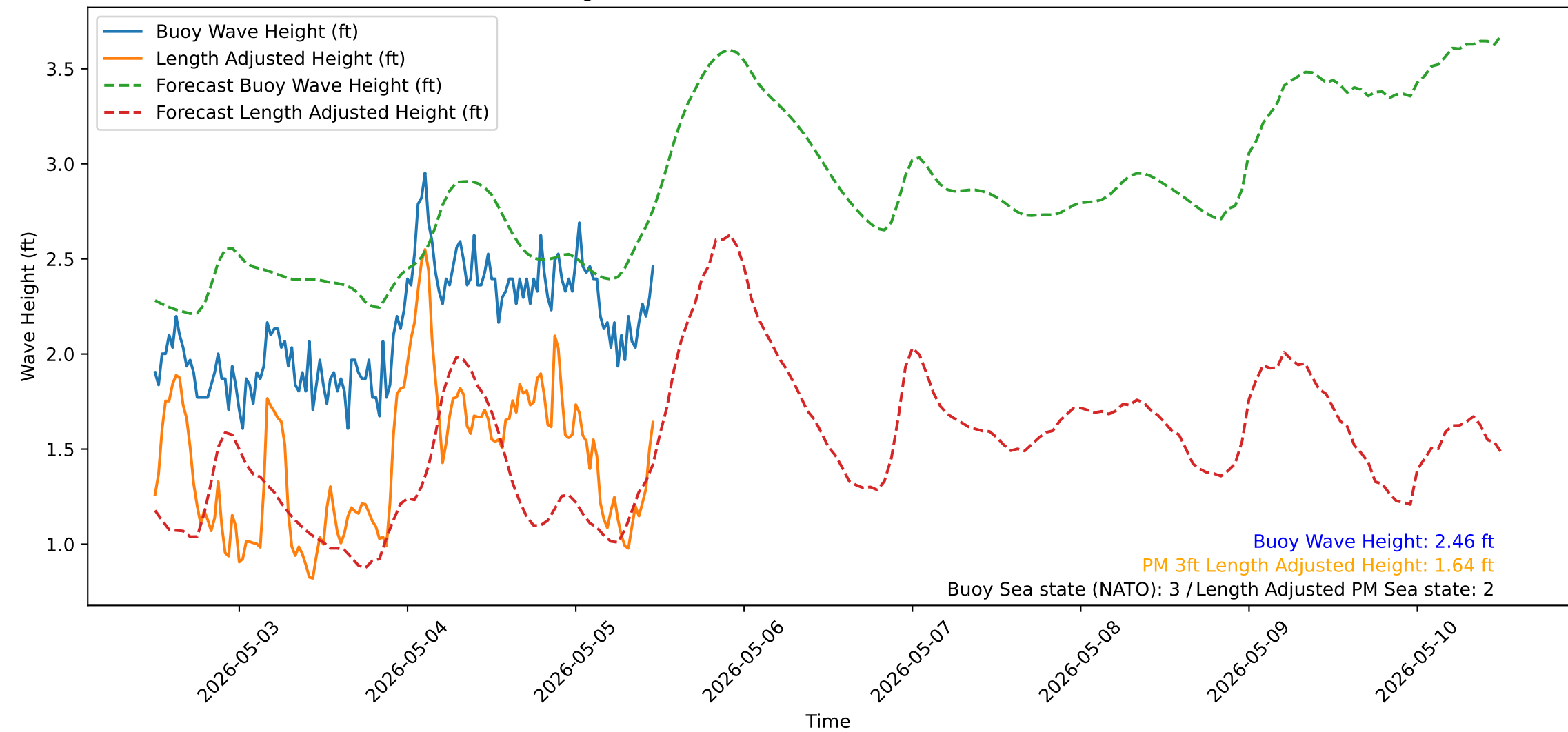
Wave Heights over Time for Red Beach at 2026-05-05 11:50:55
