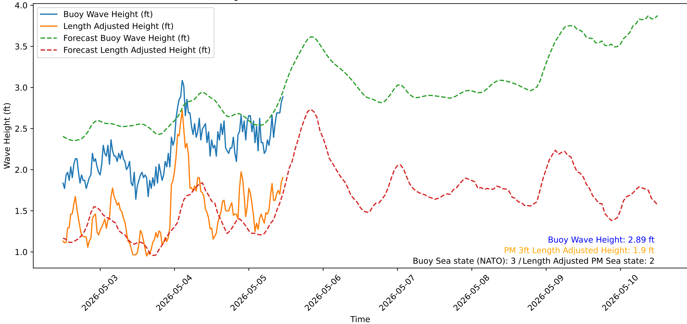
Wave Heights over Time for Oceanside Harbor at 2026-05-05 11:50:35
