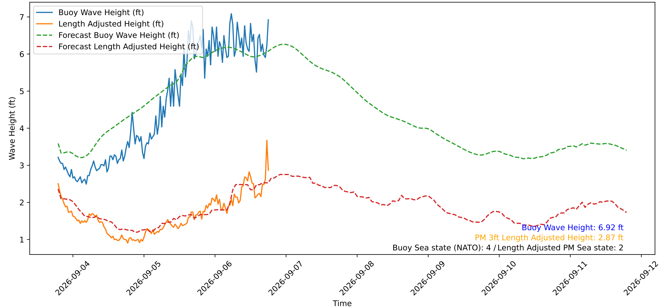
Wave Heights over Time for Green Beach at 2026-09-06 18:41:12
