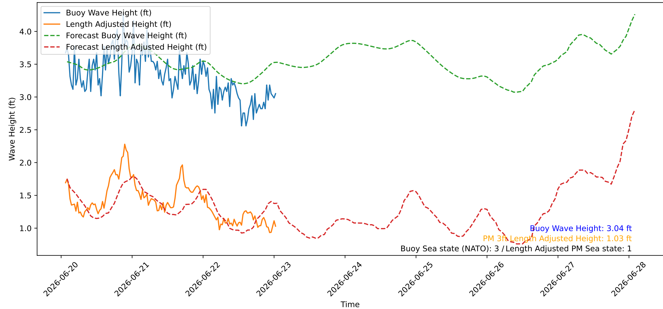
Wave Heights over Time for Oceanside Harbor at 2026-06-23 01:40:26
