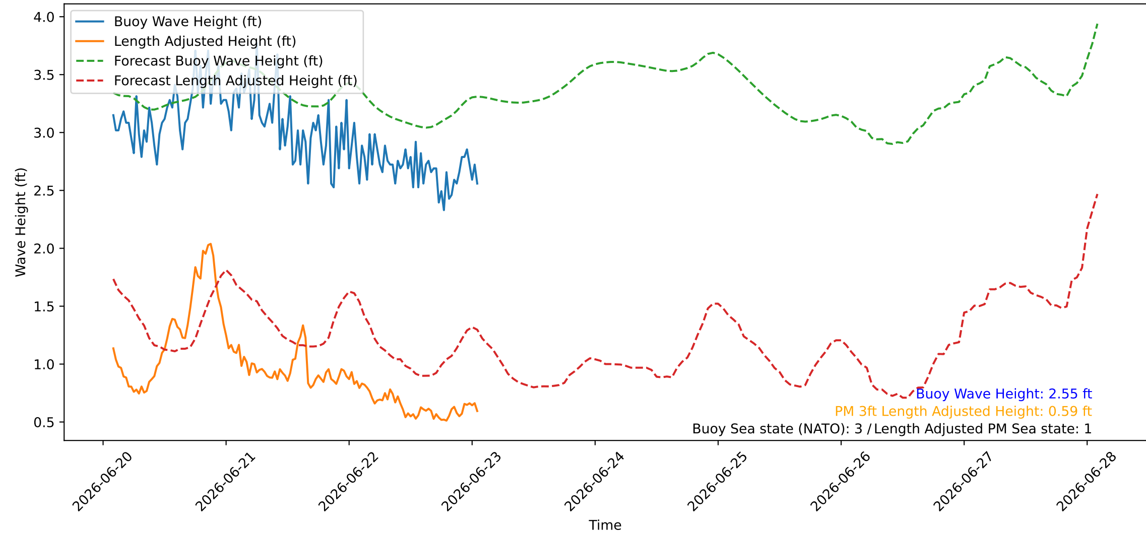
Wave Heights over Time for Red Beach at 2026-06-23 01:40:45
