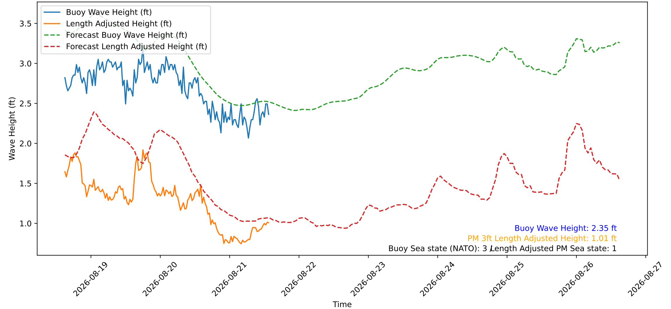
Wave Heights over Time for Red Beach at 2026-08-21 14:30:46
