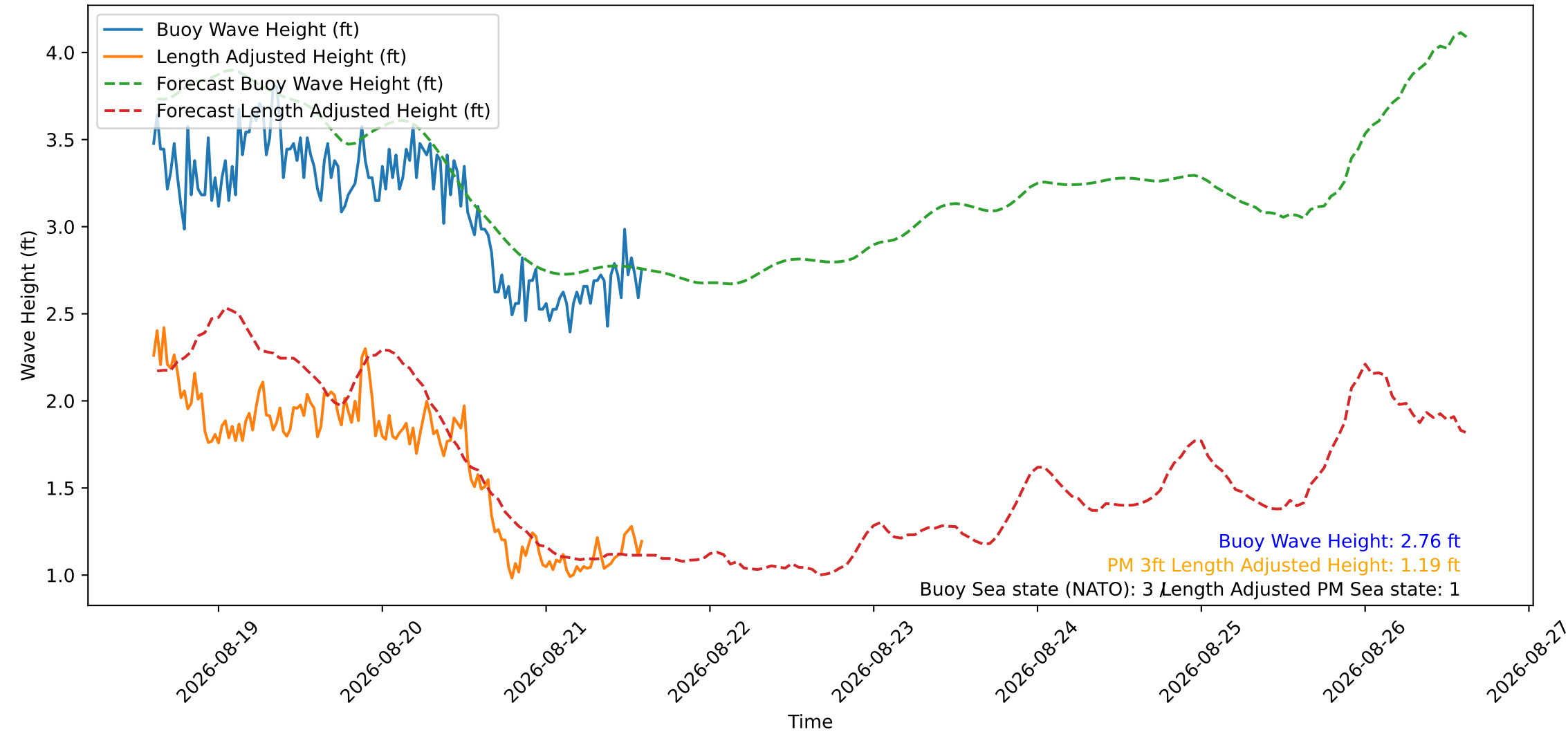
Wave Heights over Time for Oceanside Harbor at 2026-08-21 14:30:26
