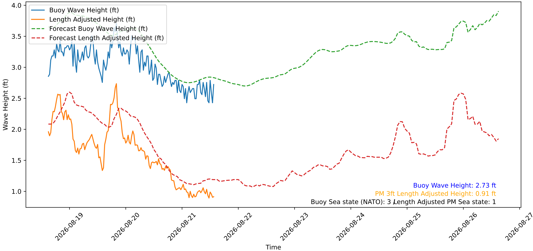
Wave Heights over Time for Green Beach at 2026-08-21 14:31:08
