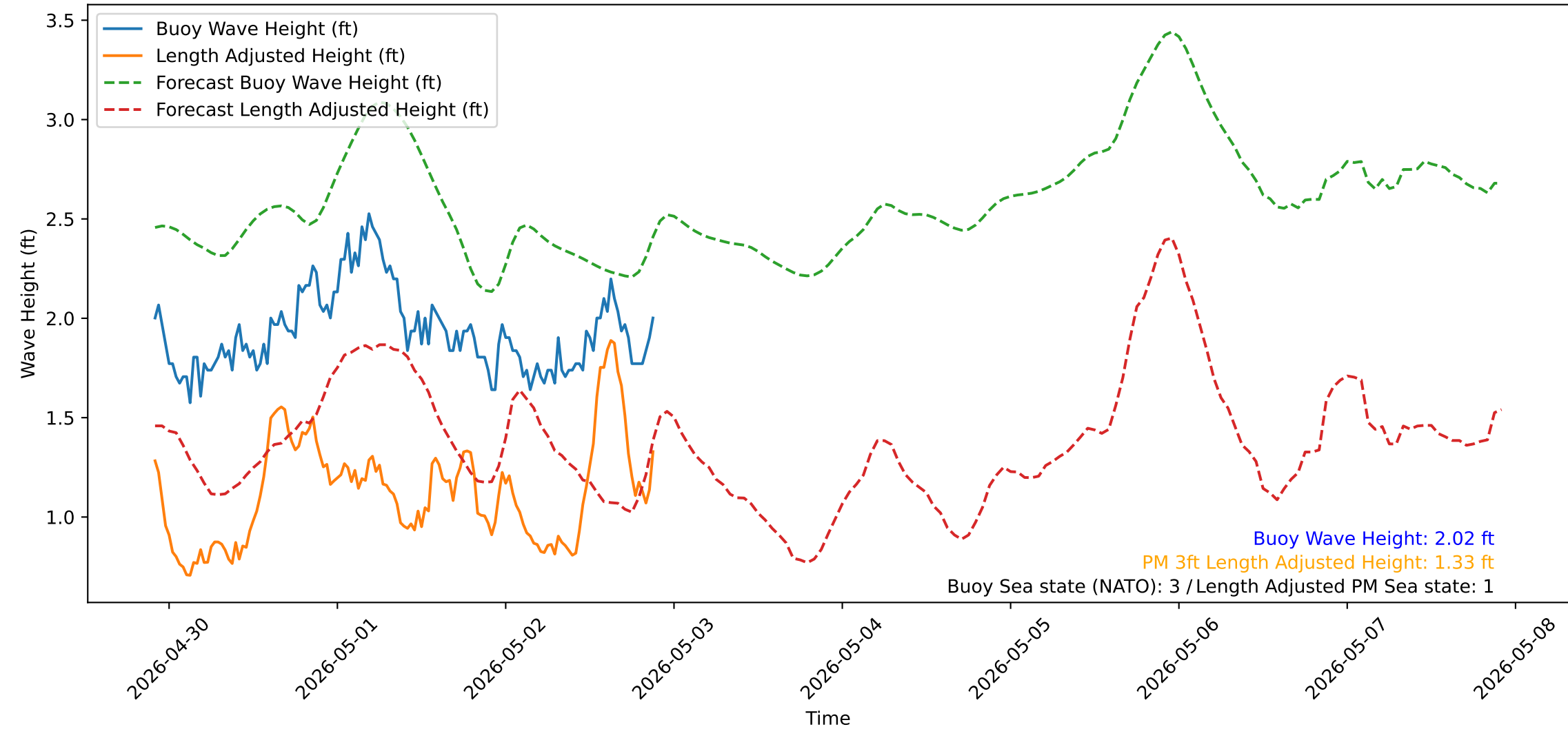
Wave Heights over Time for Red Beach at 2026-05-02 21:50:52
