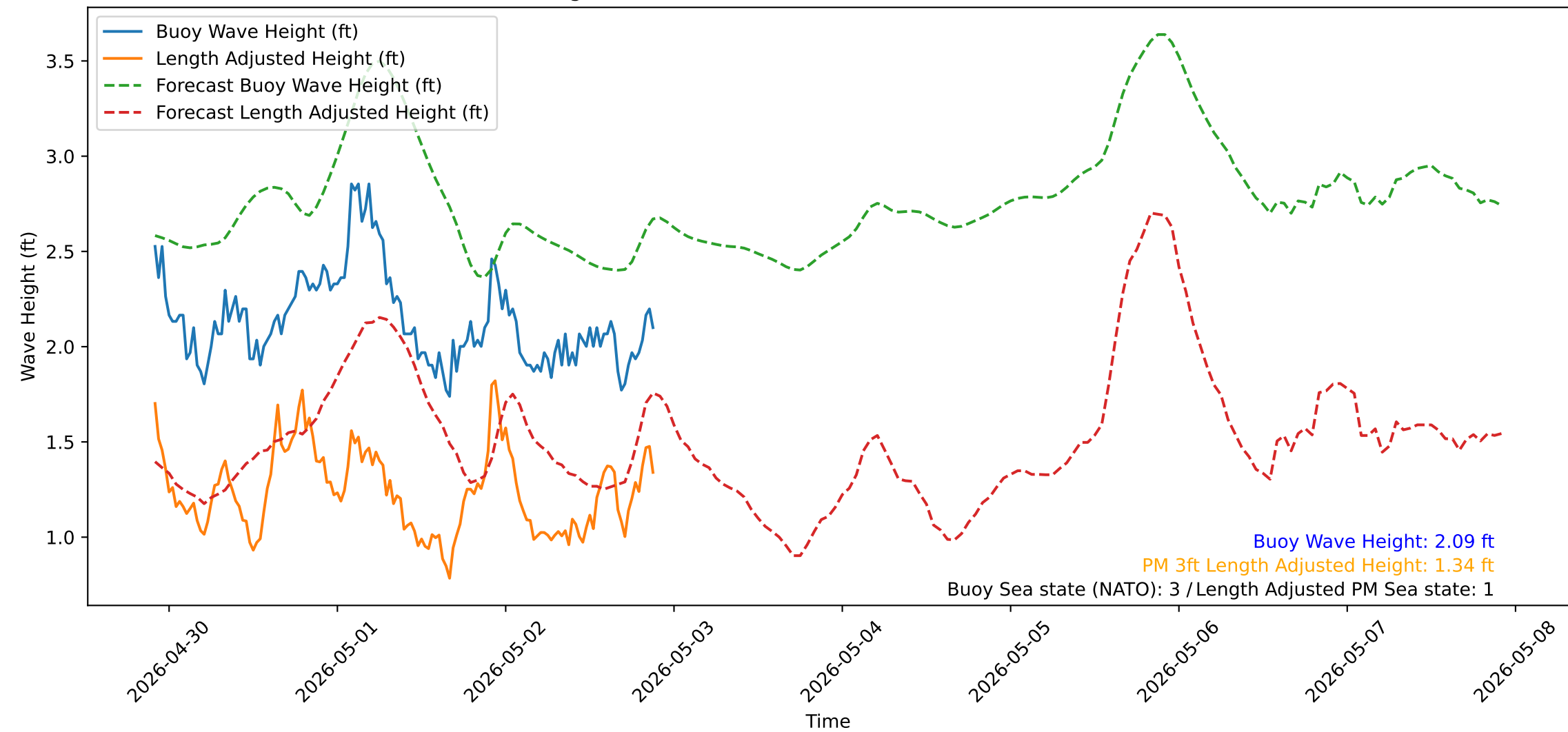
Wave Heights over Time for Green Beach at 2026-05-02 21:51:15
