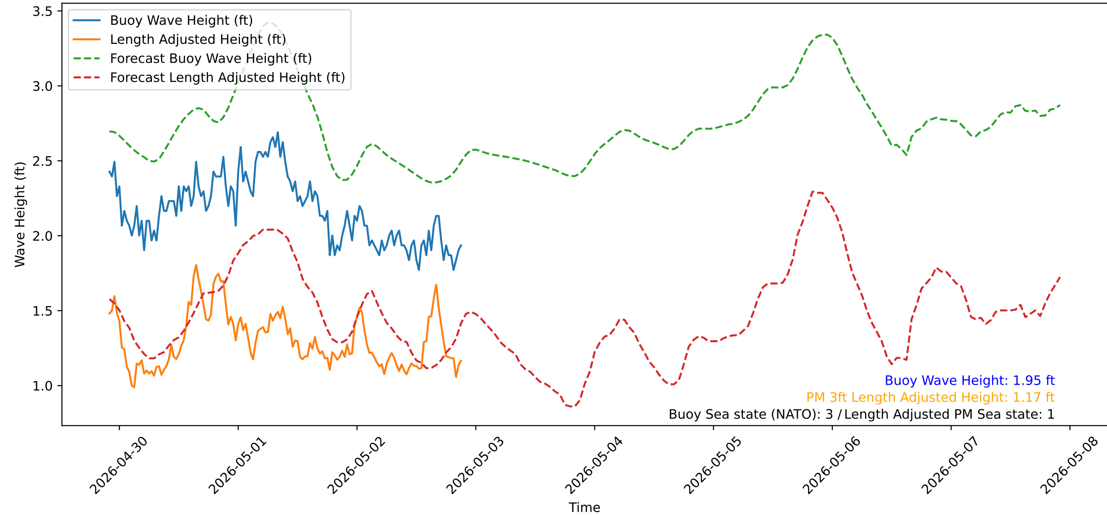
Wave Heights over Time for Oceanside Harbor at 2026-05-02 21:50:32
