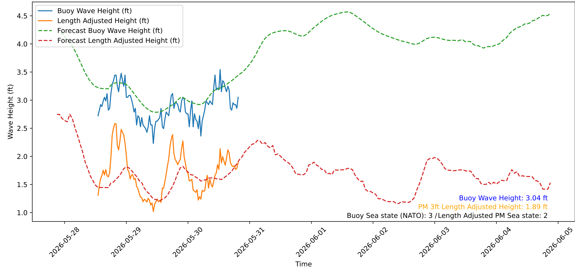
Wave Heights over Time for Oceanside Harbor at 2026-05-30 20:30:25
