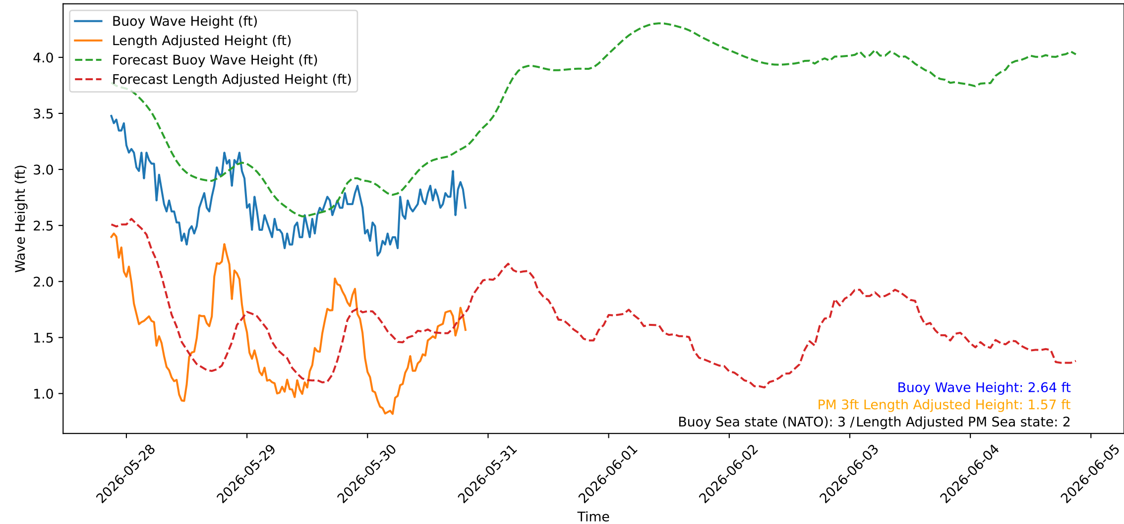
Wave Heights over Time for Red Beach at 2026-05-30 20:30:44
