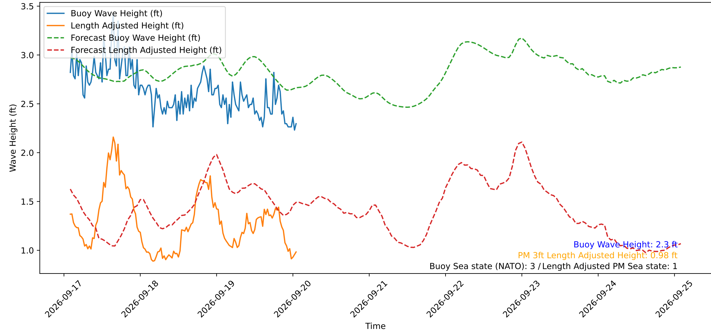
Wave Heights over Time for Red Beach at 2026-09-20 01:50:50
