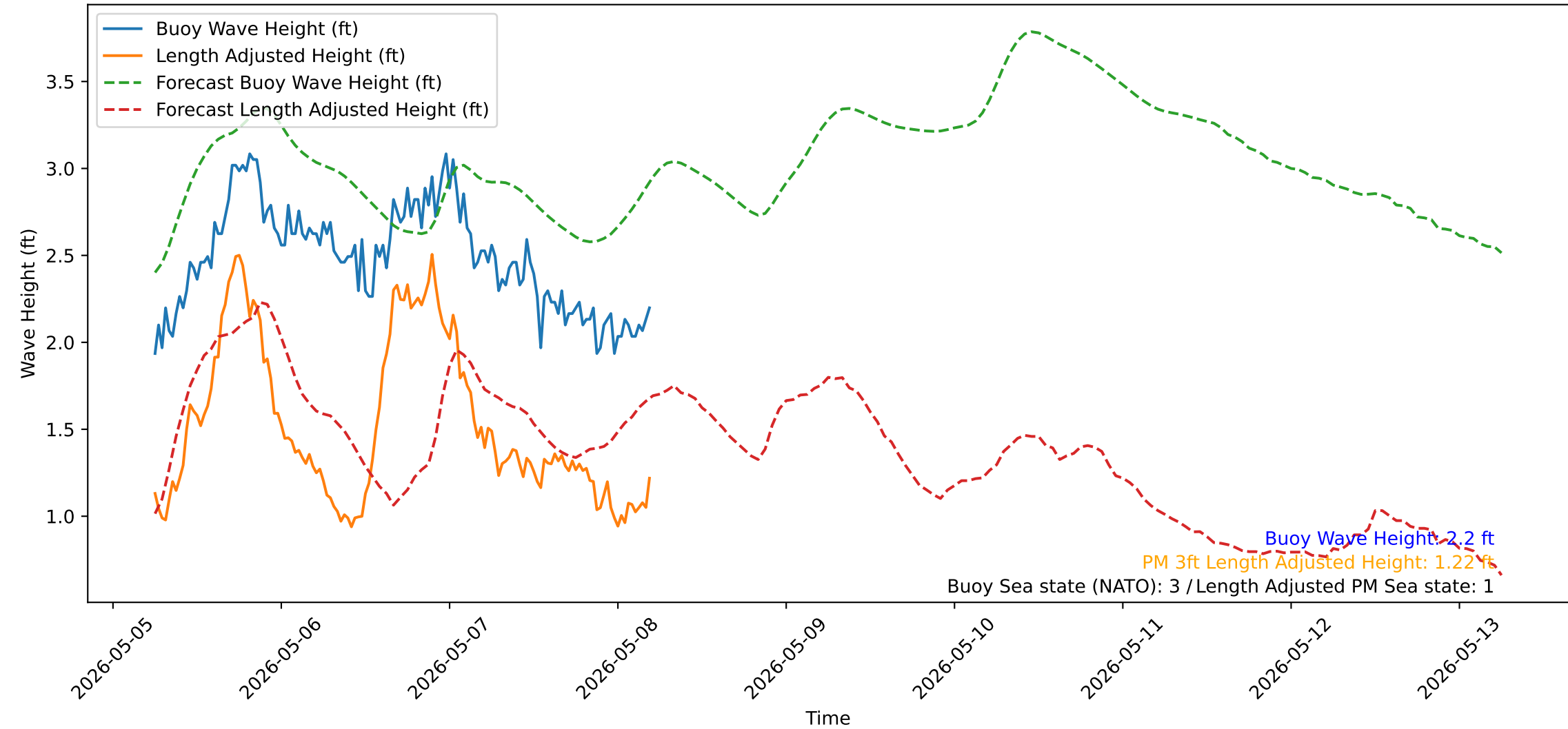
Wave Heights over Time for Red Beach at 2026-05-08 05:30:50
