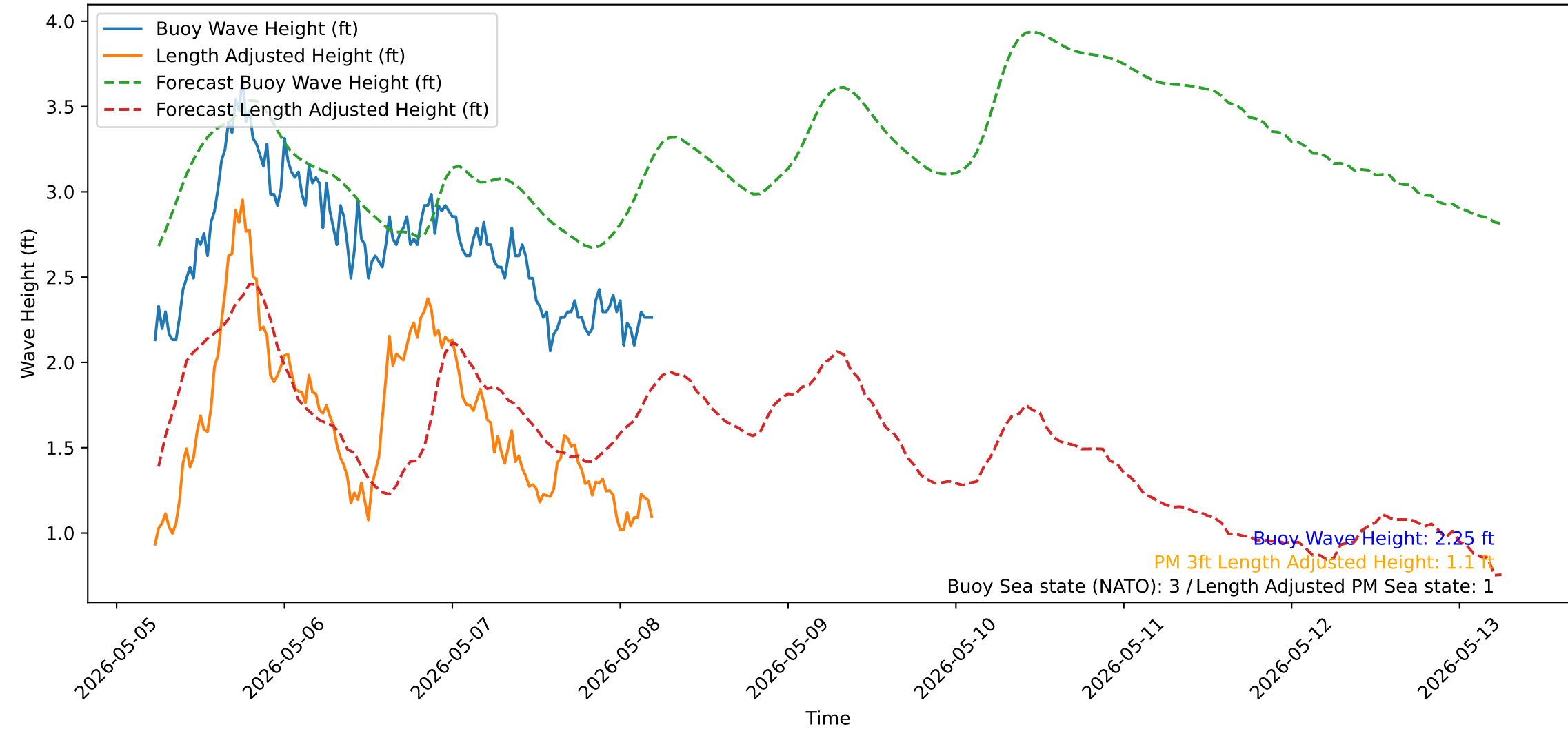
Wave Heights over Time for Green Beach at 2026-05-08 05:31:12
