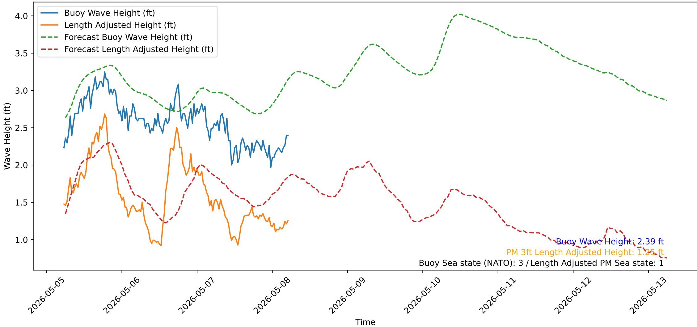
Wave Heights over Time for Oceanside Harbor at 2026-05-08 05:30:31
