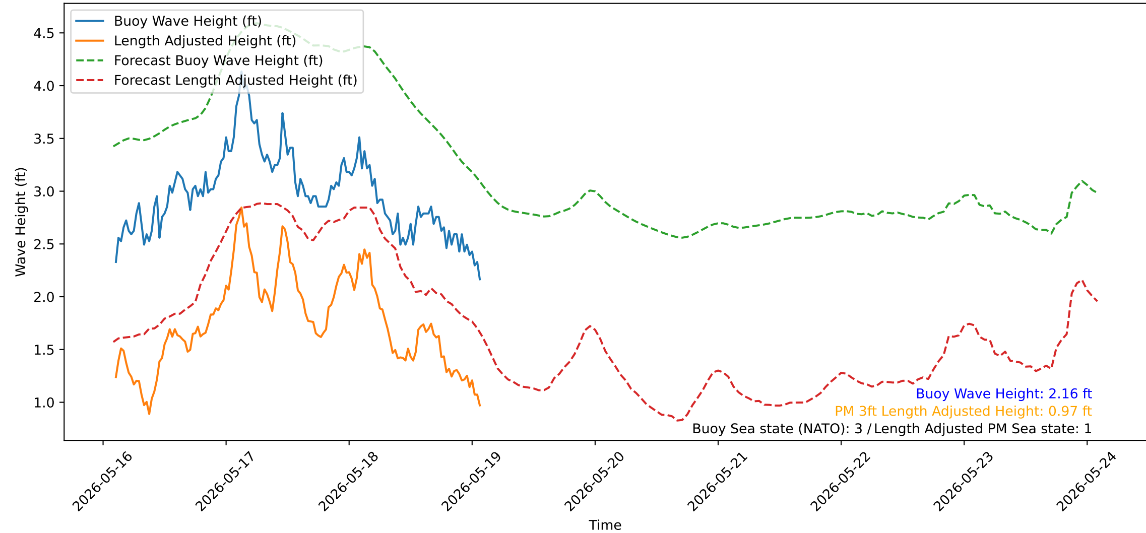
Wave Heights over Time for Red Beach at 2026-05-19 02:20:52
