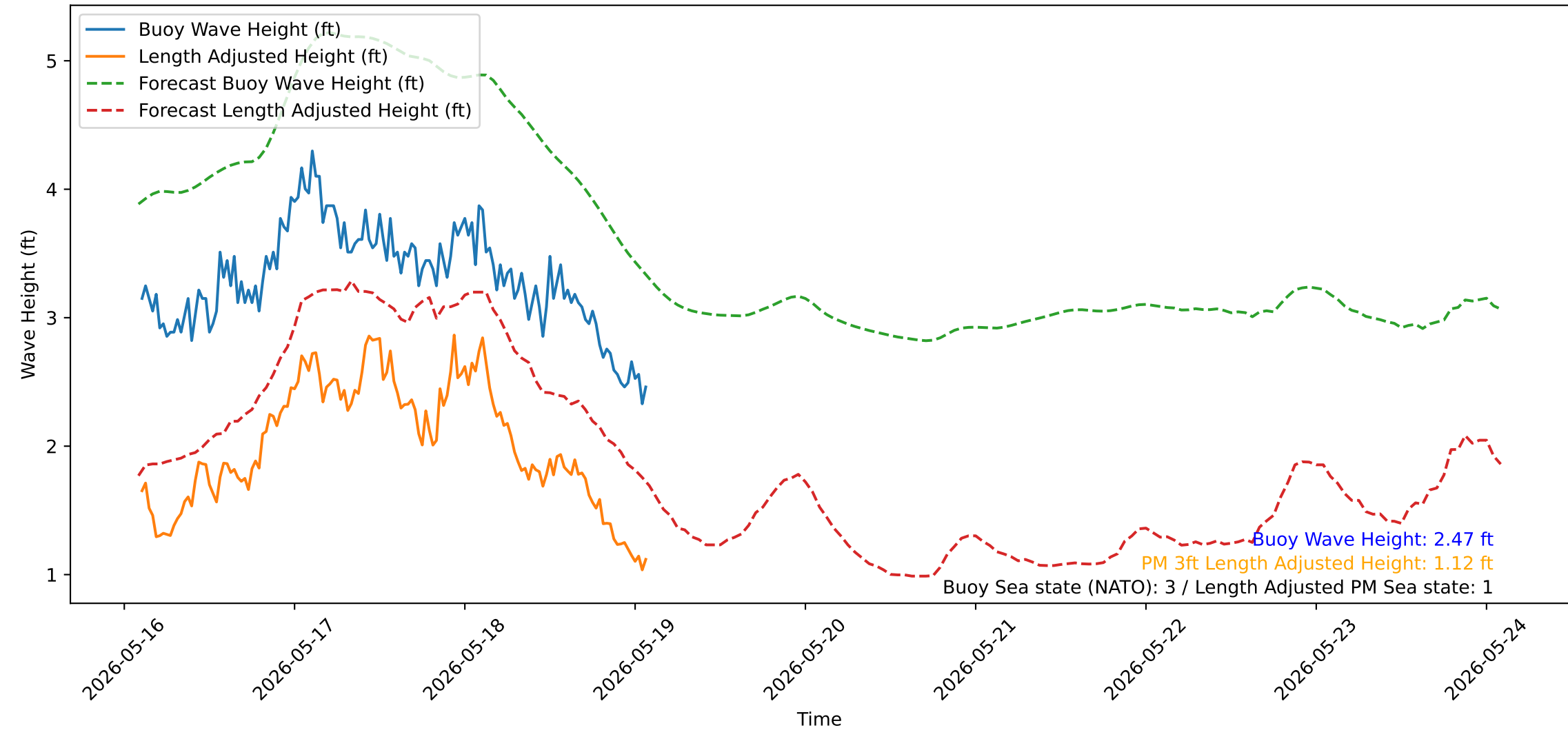
Wave Heights over Time for Oceanside Harbor at 2026-05-19 02:20:31
