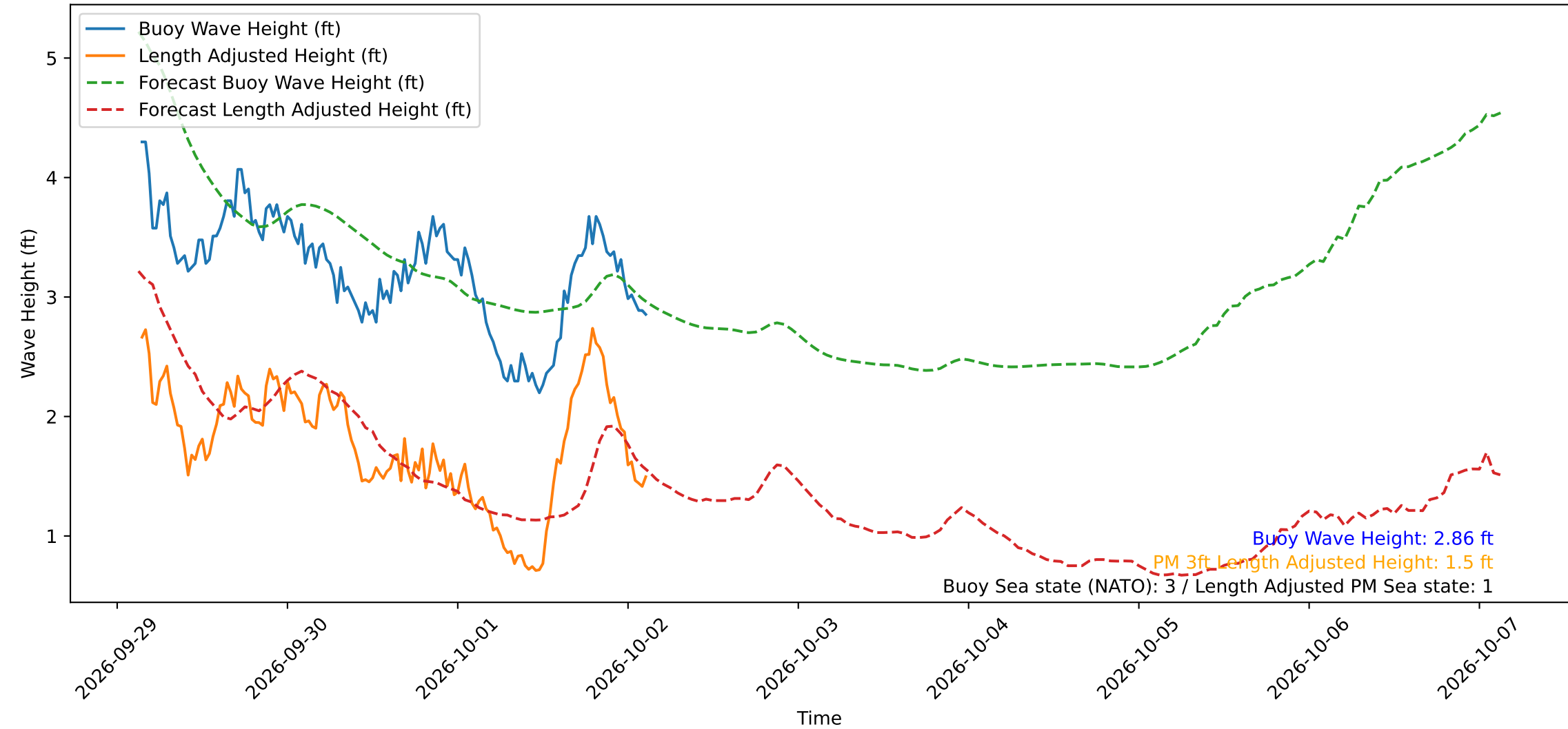
Wave Heights over Time for Green Beach at 2026-10-02 03:21:15
