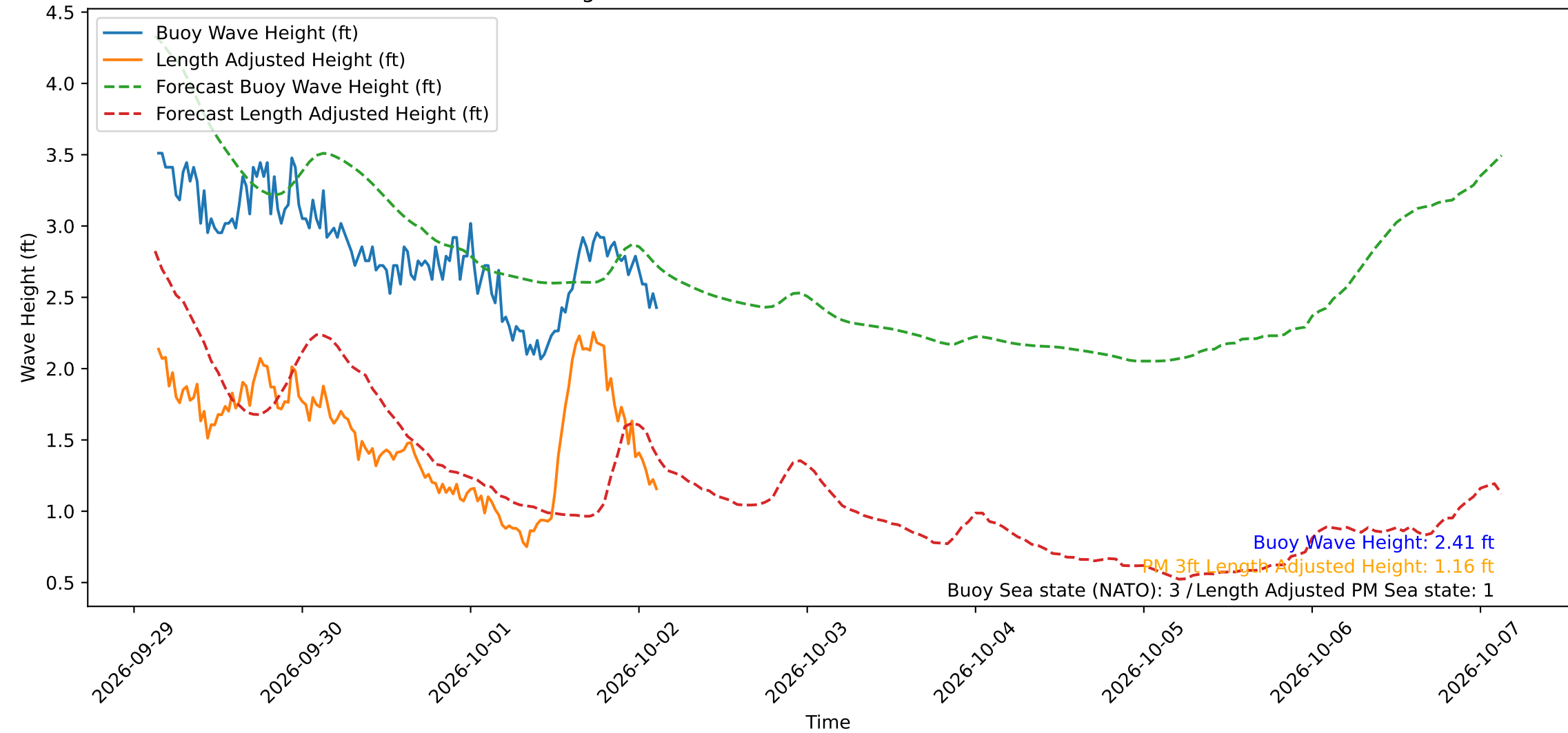
Wave Heights over Time for Red Beach at 2026-10-02 03:20:51
