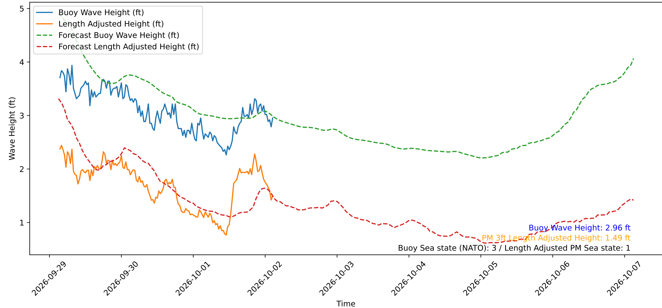
Wave Heights over Time for Oceanside Harbor at 2026-10-02 03:20:30
