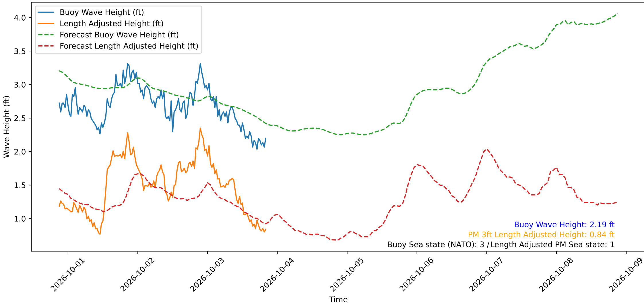
Wave Heights over Time for Oceanside Harbor at 2026-10-03 20:50:29
