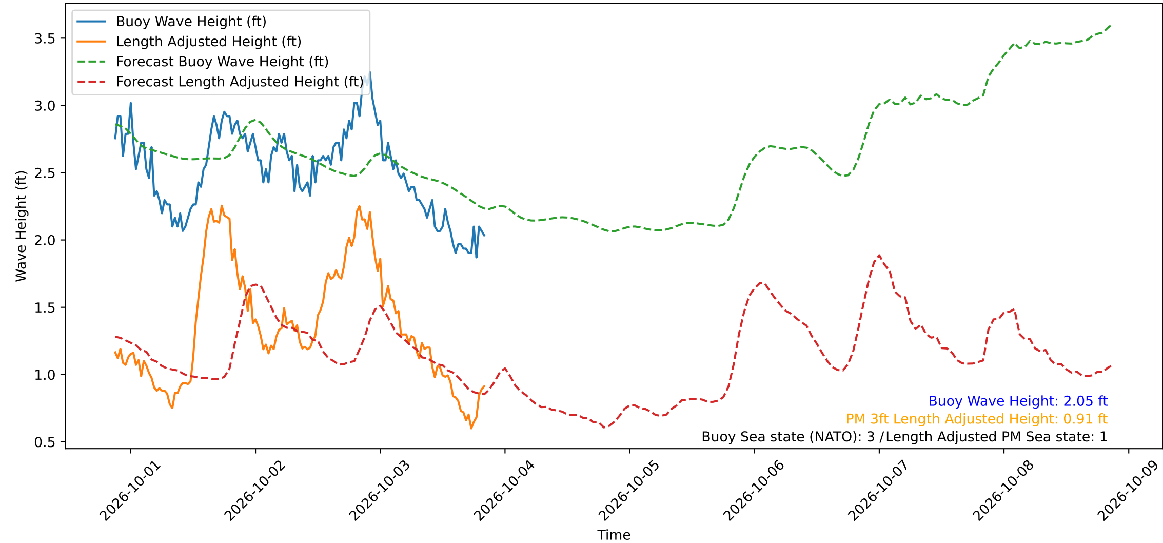
Wave Heights over Time for Red Beach at 2026-10-03 20:50:50
