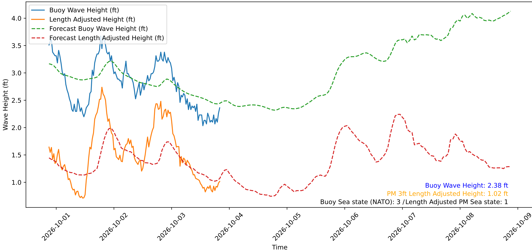
Wave Heights over Time for Green Beach at 2026-10-03 20:51:15
