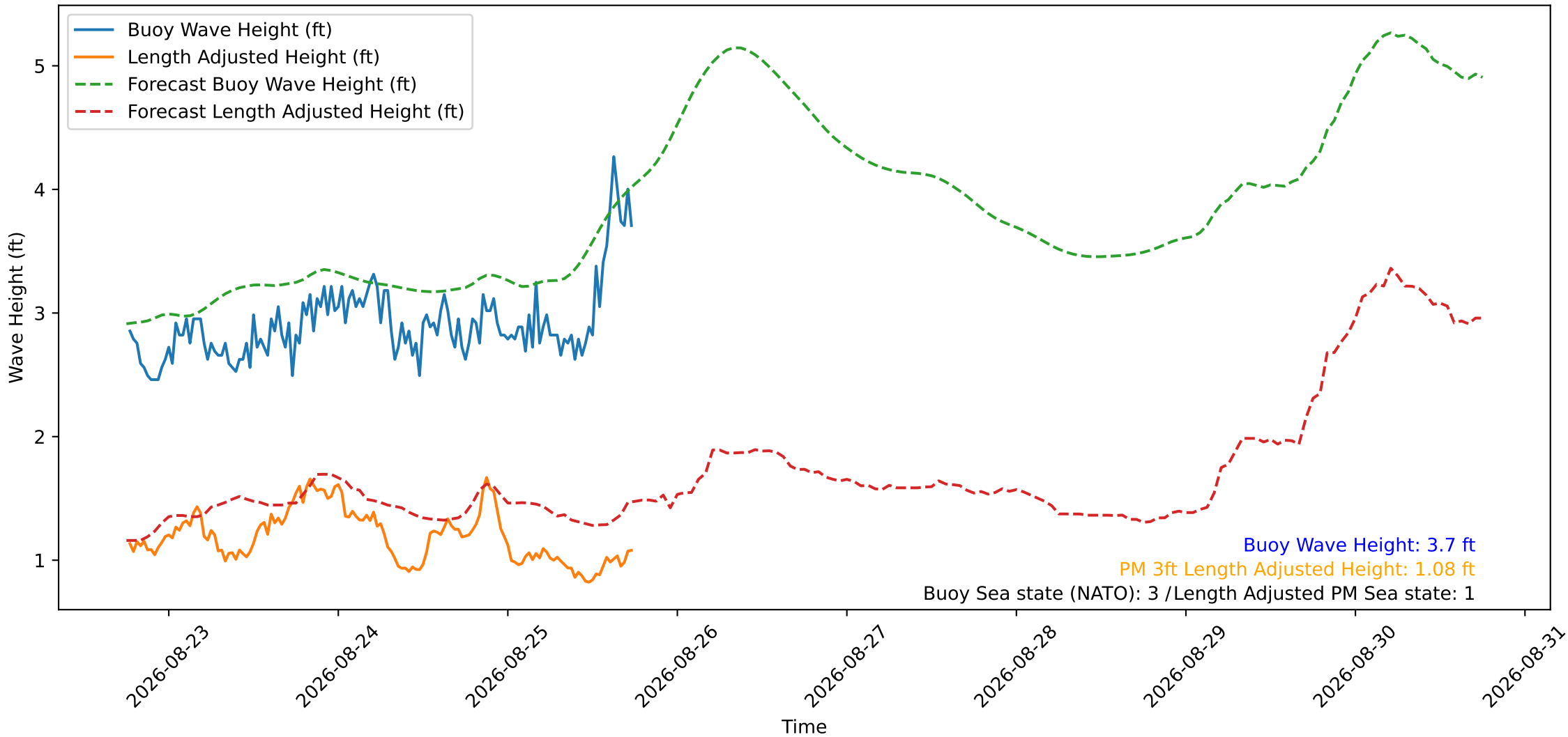
Wave Heights over Time for Green Beach at 2026-08-25 18:21:14
