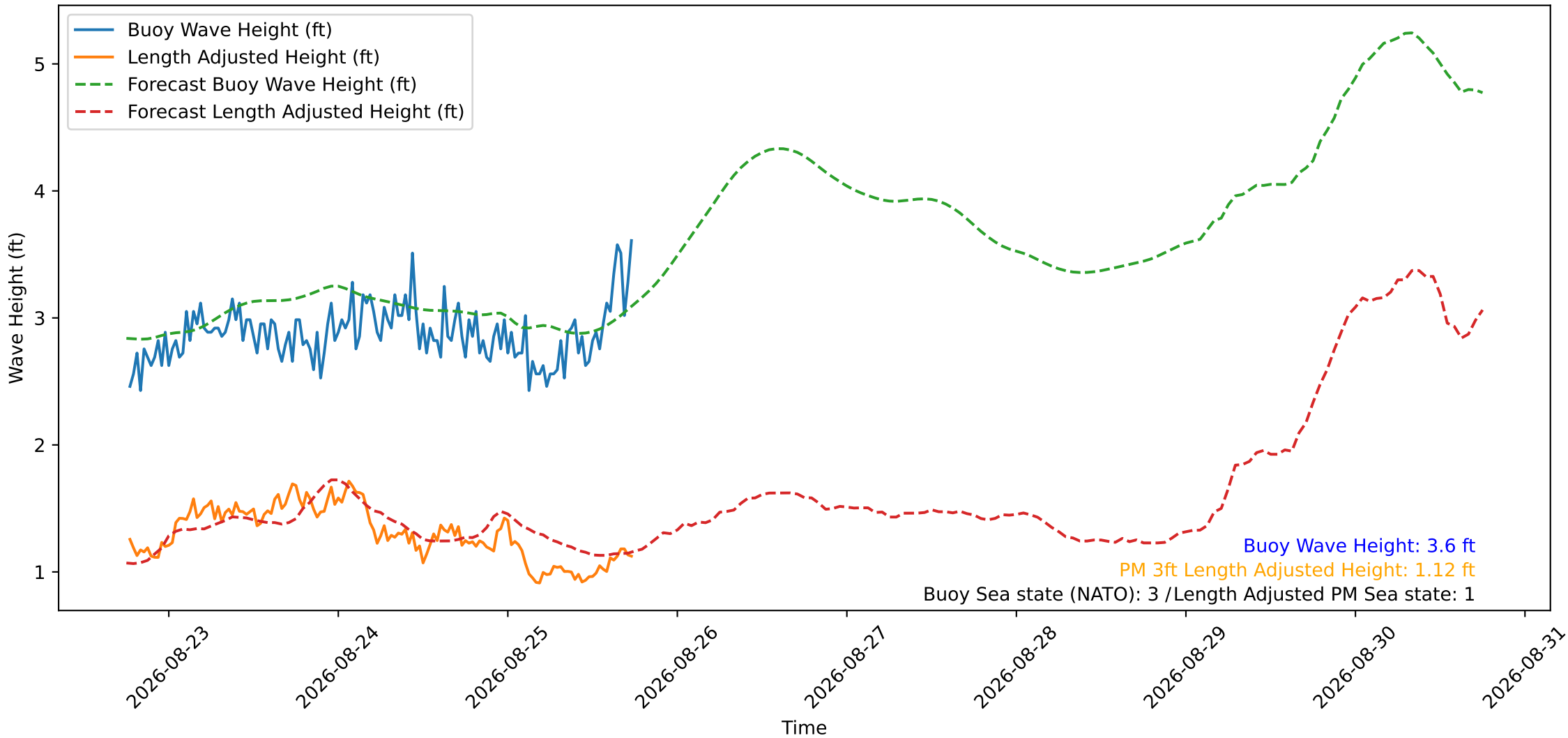
Wave Heights over Time for Oceanside Harbor at 2026-08-25 18:20:29
