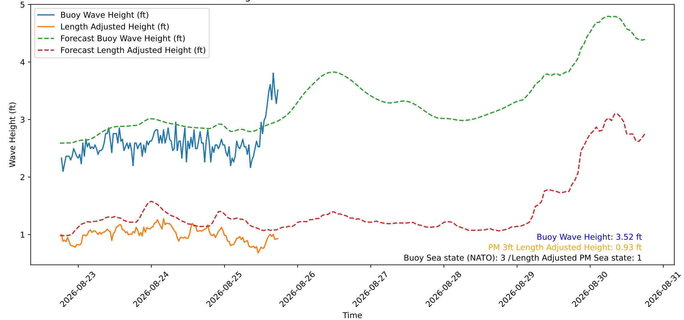
Wave Heights over Time for Red Beach at 2026-08-25 18:20:50
