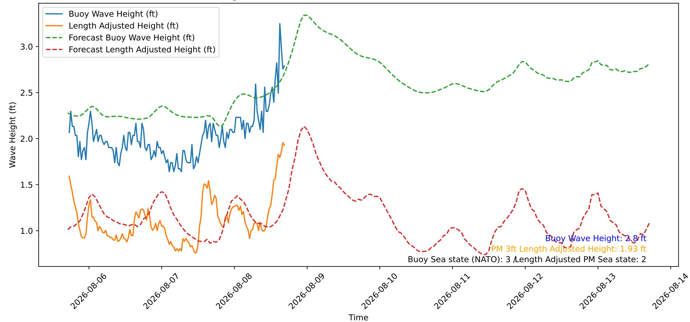
Wave Heights over Time for Oceanside Harbor at 2026-08-08 17:20:26
