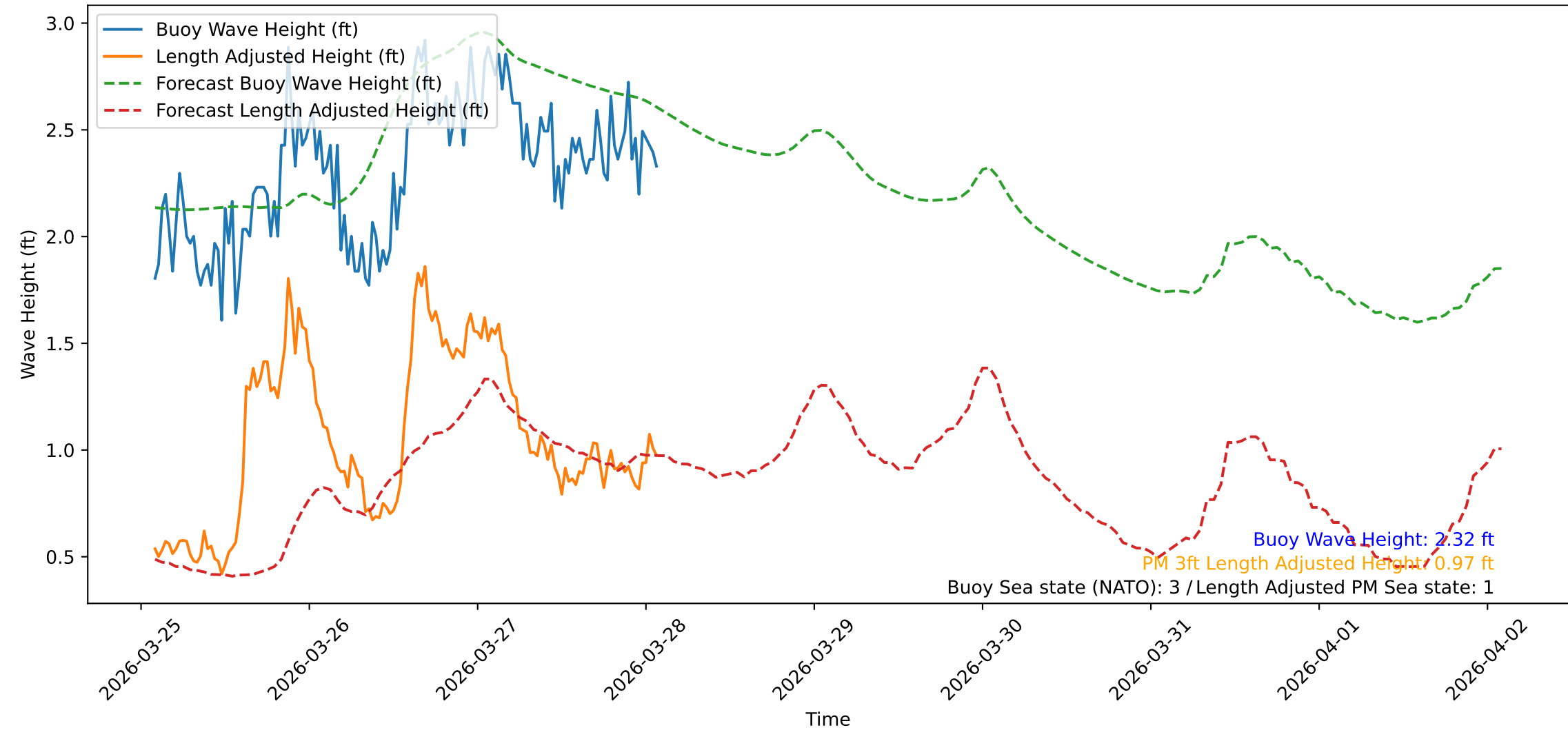
Wave Heights over Time for Oceanside Harbor at 2026-03-28 02:10:32
