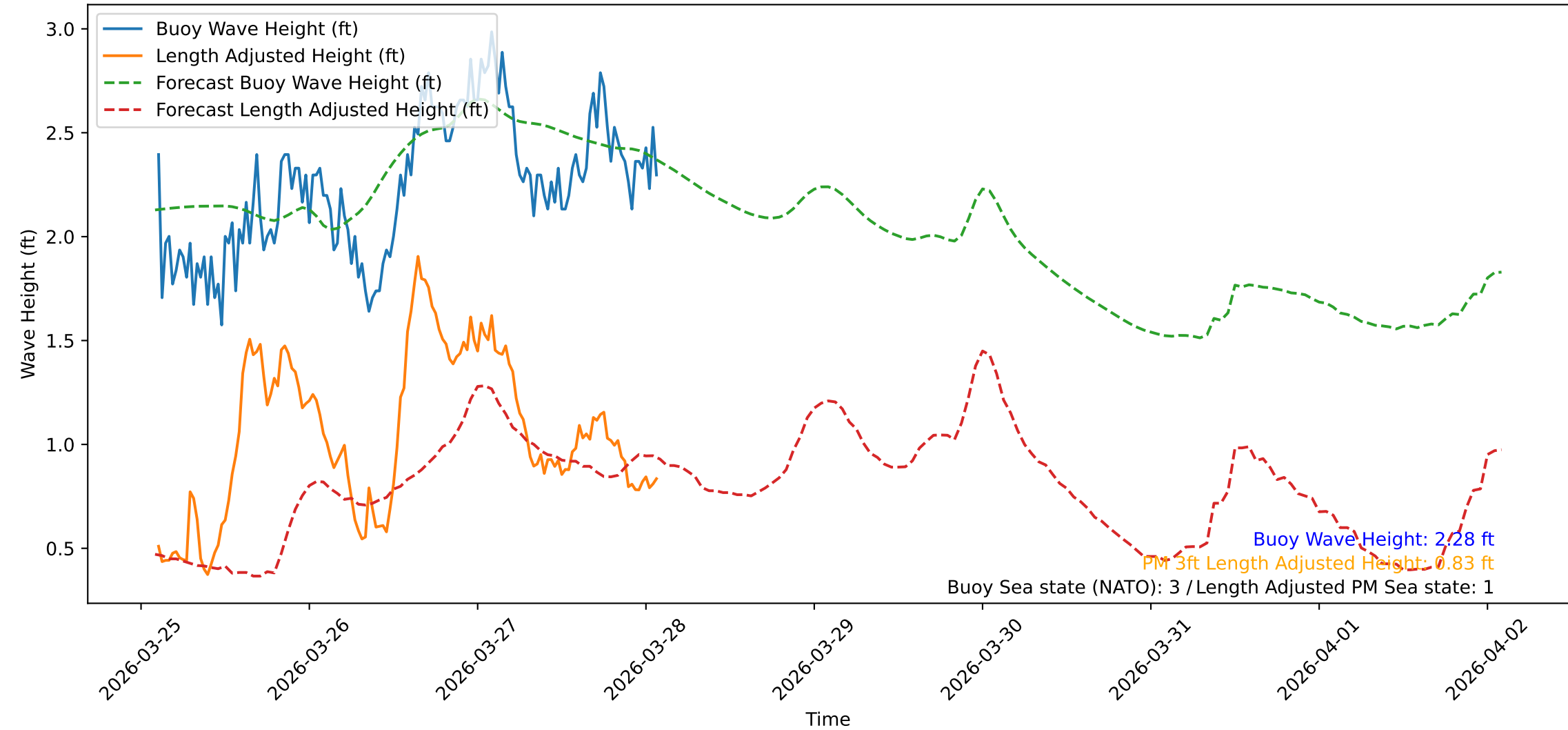
Wave Heights over Time for Red Beach at 2026-03-28 02:10:48
