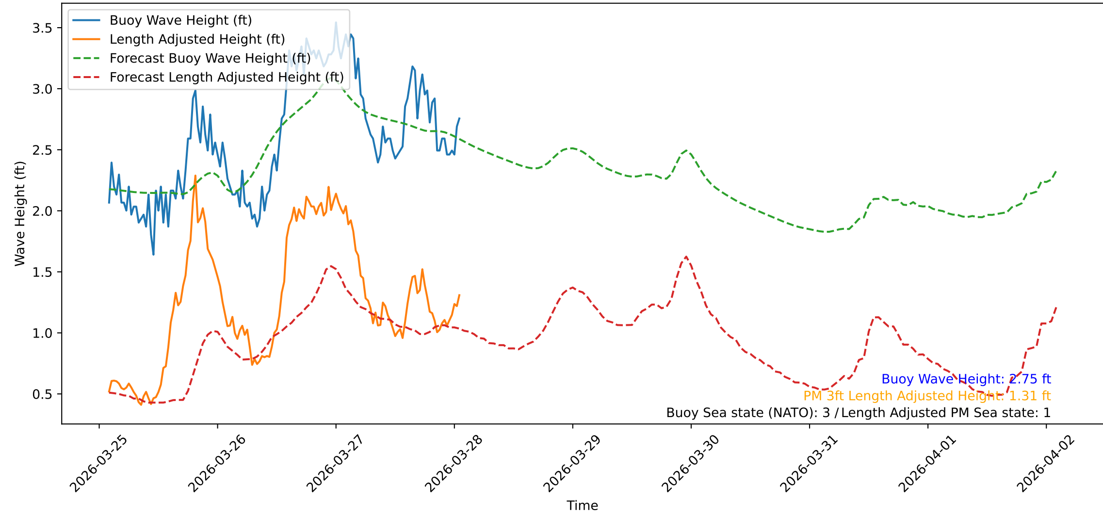
Wave Heights over Time for Green Beach at 2026-03-28 02:11:10
