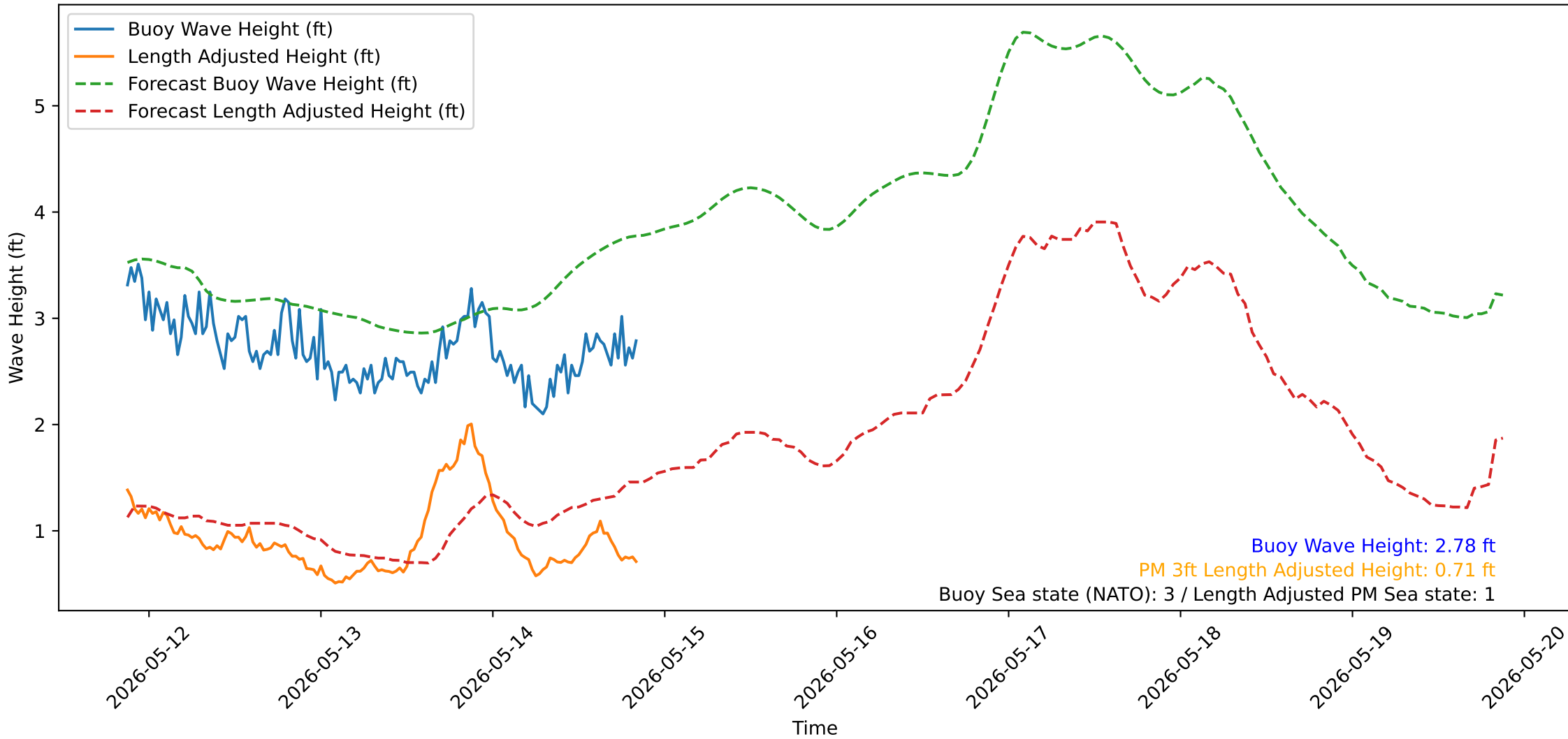
Wave Heights over Time for Green Beach at 2026-05-14 20:51:16
