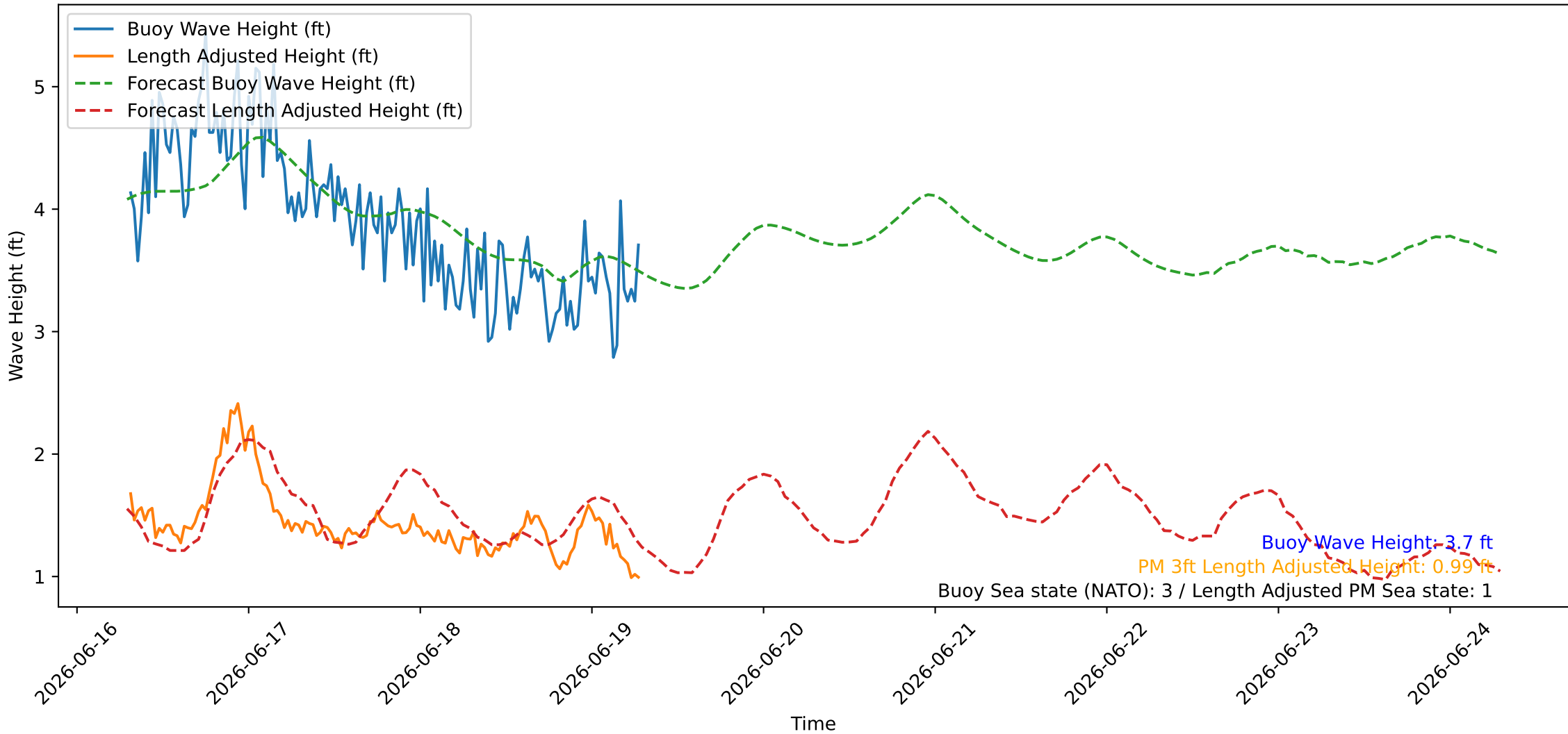
Wave Heights over Time for Oceanside Harbor at 2026-06-19 07:20:26
