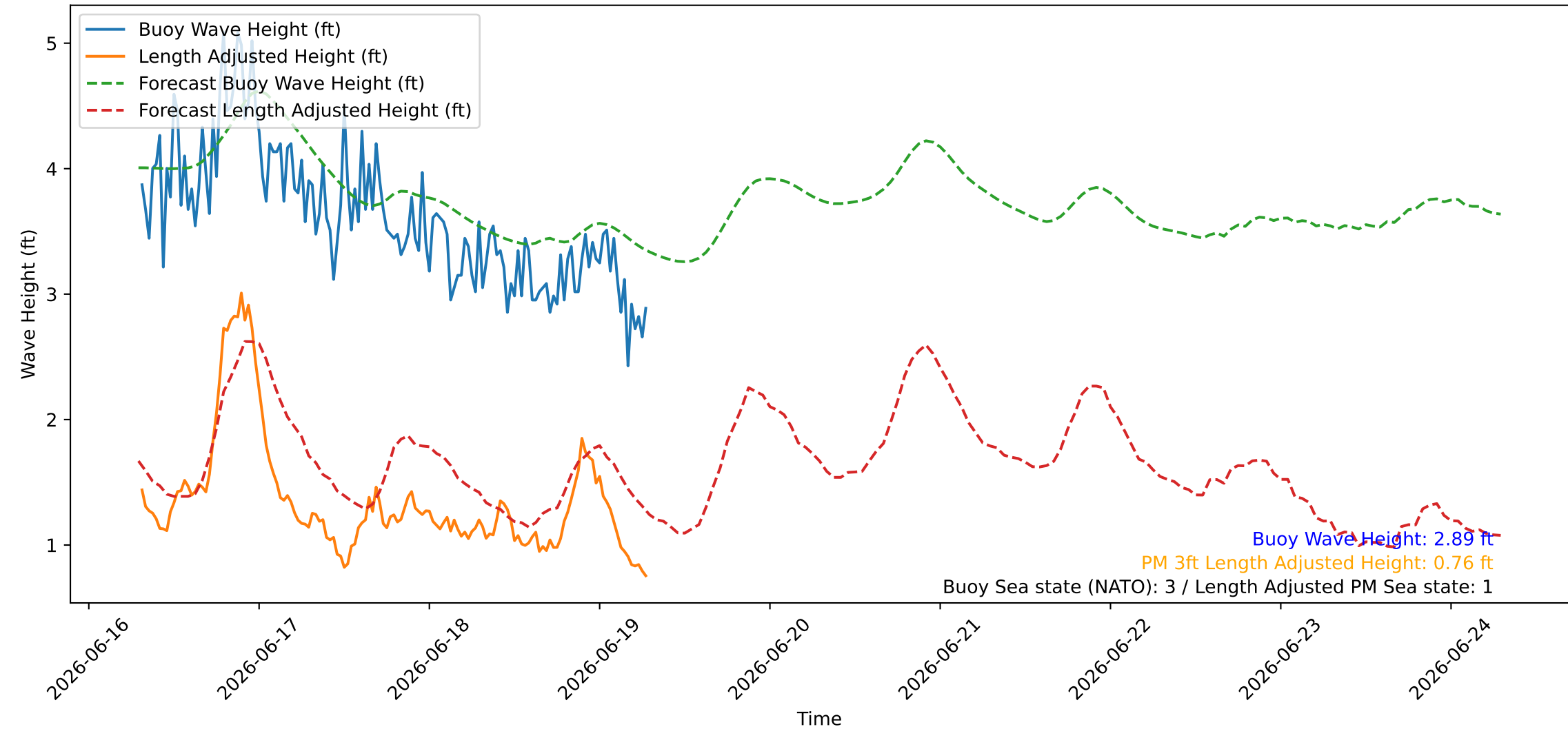
Wave Heights over Time for Green Beach at 2026-06-19 07:21:08
