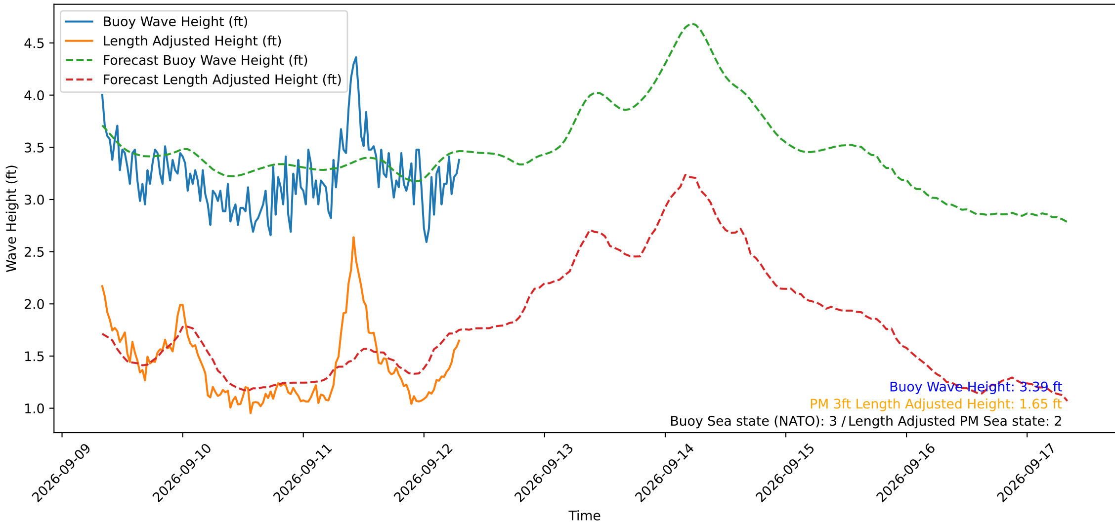
Wave Heights over Time for Oceanside Harbor at 2026-09-12 08:00:29
