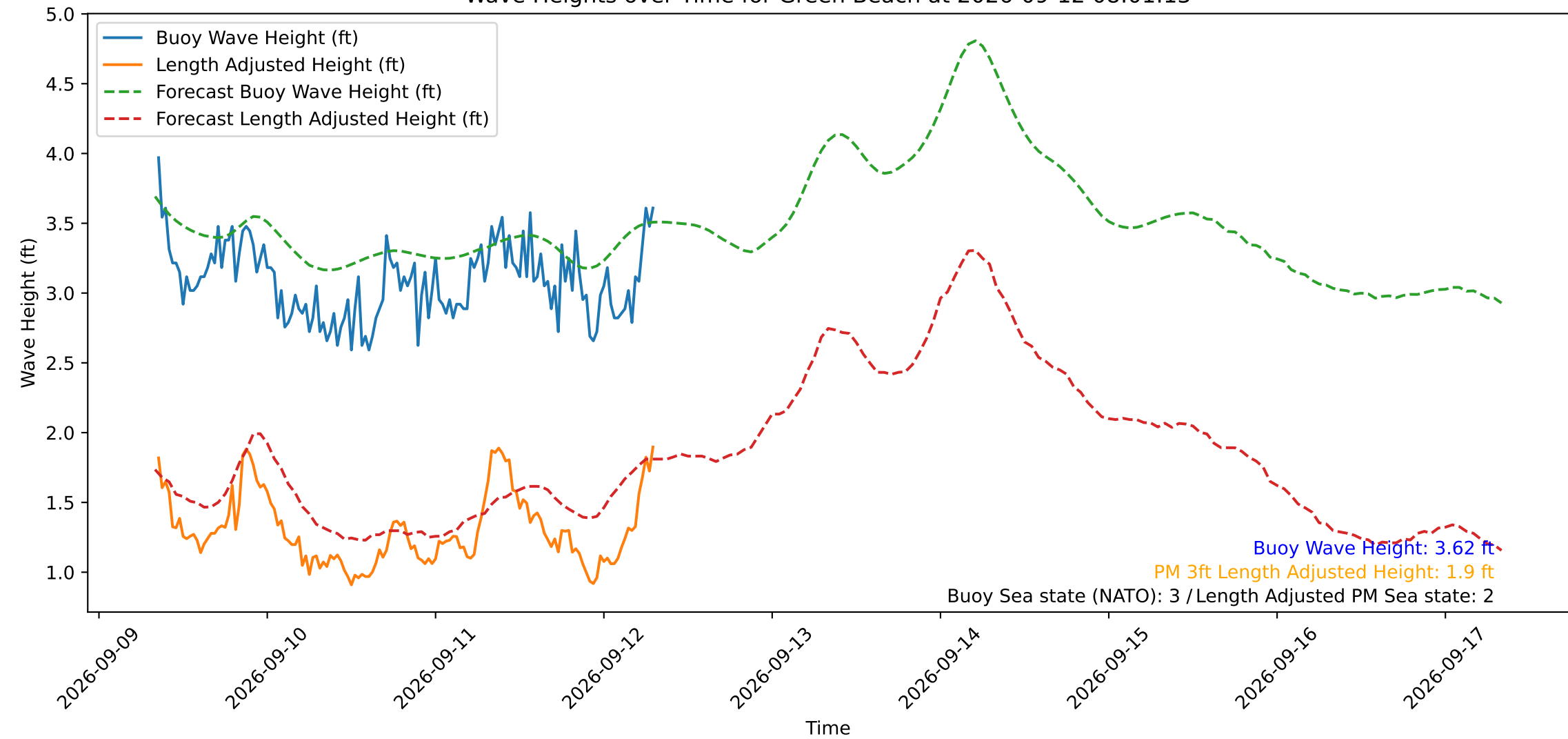
Wave Heights over Time for Green Beach at 2026-09-12 08:01:13
