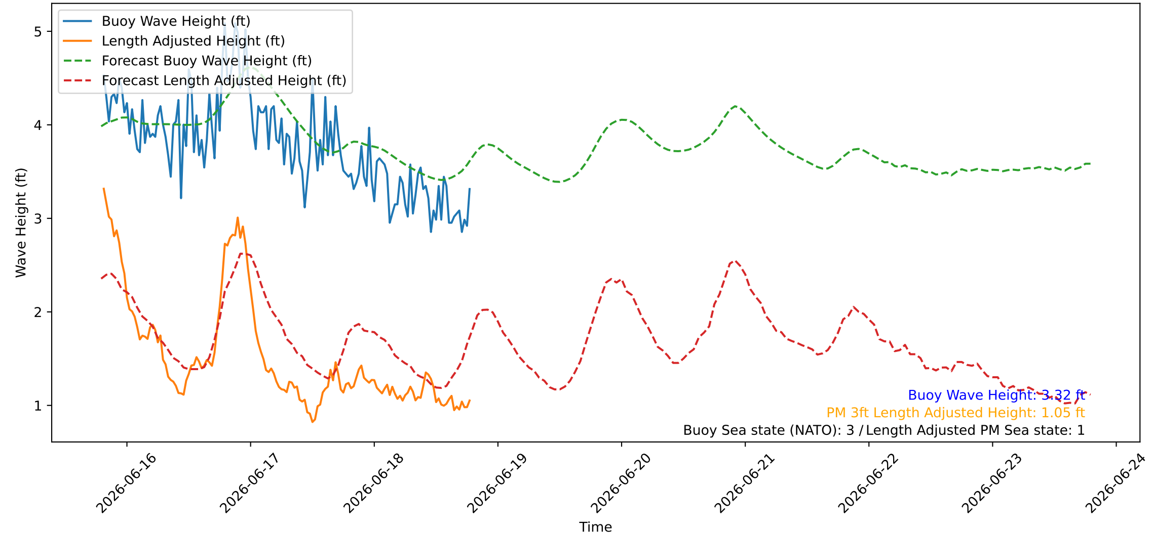
Wave Heights over Time for Green Beach at 2026-06-18 19:21:08
