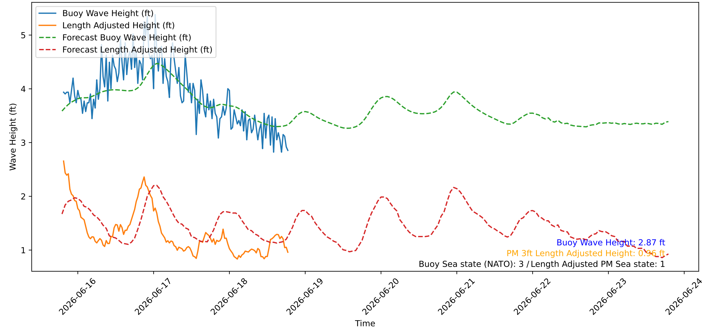
Wave Heights over Time for Red Beach at 2026-06-18 19:20:46
