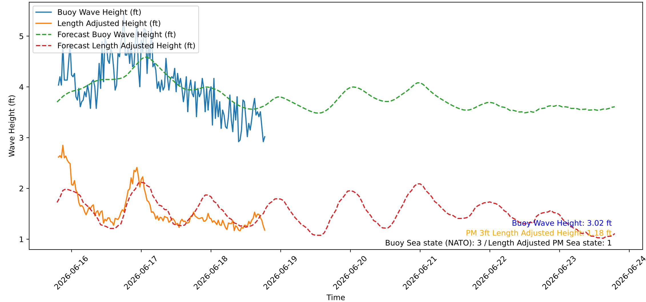
Wave Heights over Time for Oceanside Harbor at 2026-06-18 19:20:26
