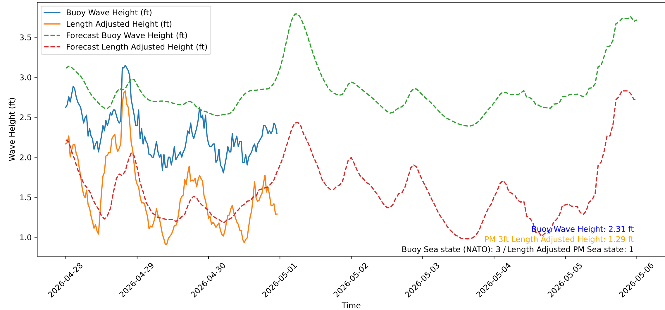
Wave Heights over Time for Green Beach at 2026-04-30 23:51:15
