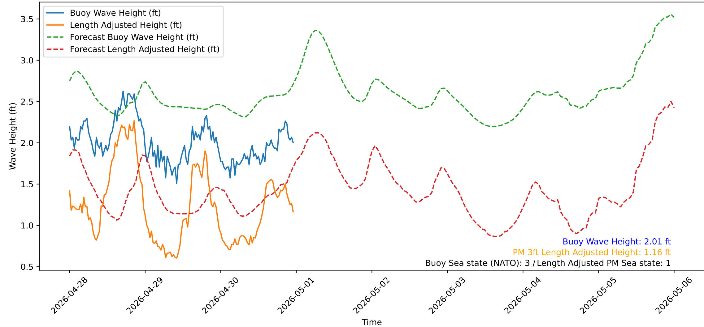
Wave Heights over Time for Red Beach at 2026-04-30 23:50:52
