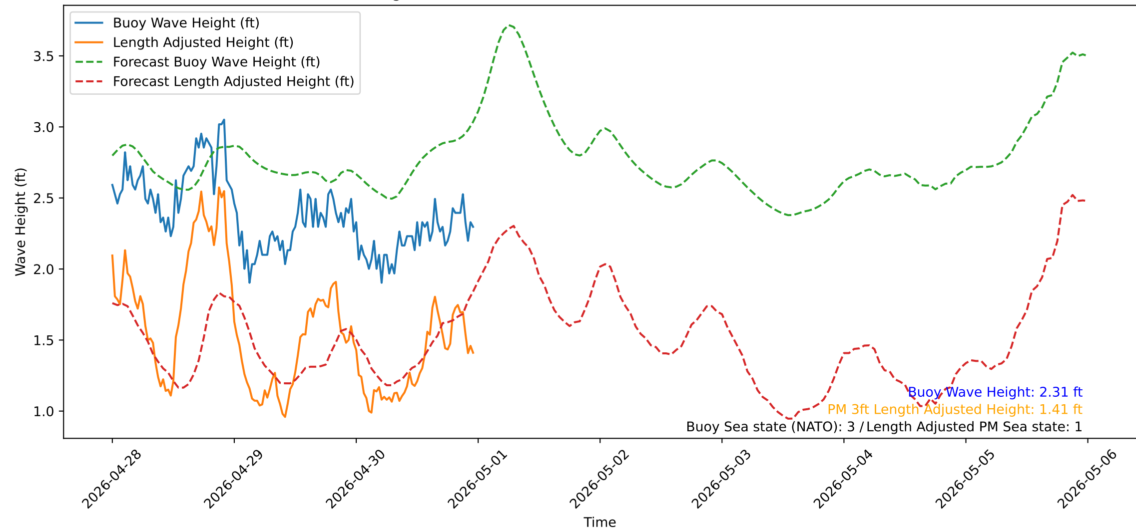
Wave Heights over Time for Oceanside Harbor at 2026-04-30 23:50:32
