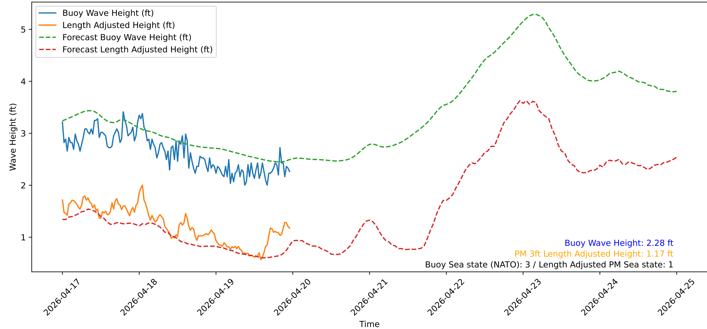
Wave Heights over Time for Oceanside Harbor at 2026-04-19 23:50:32
