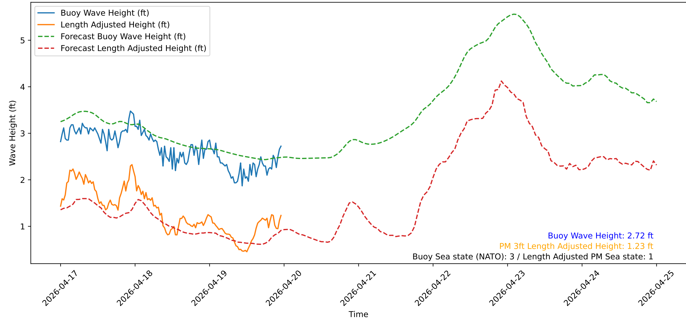
Wave Heights over Time for Green Beach at 2026-04-19 23:51:15
