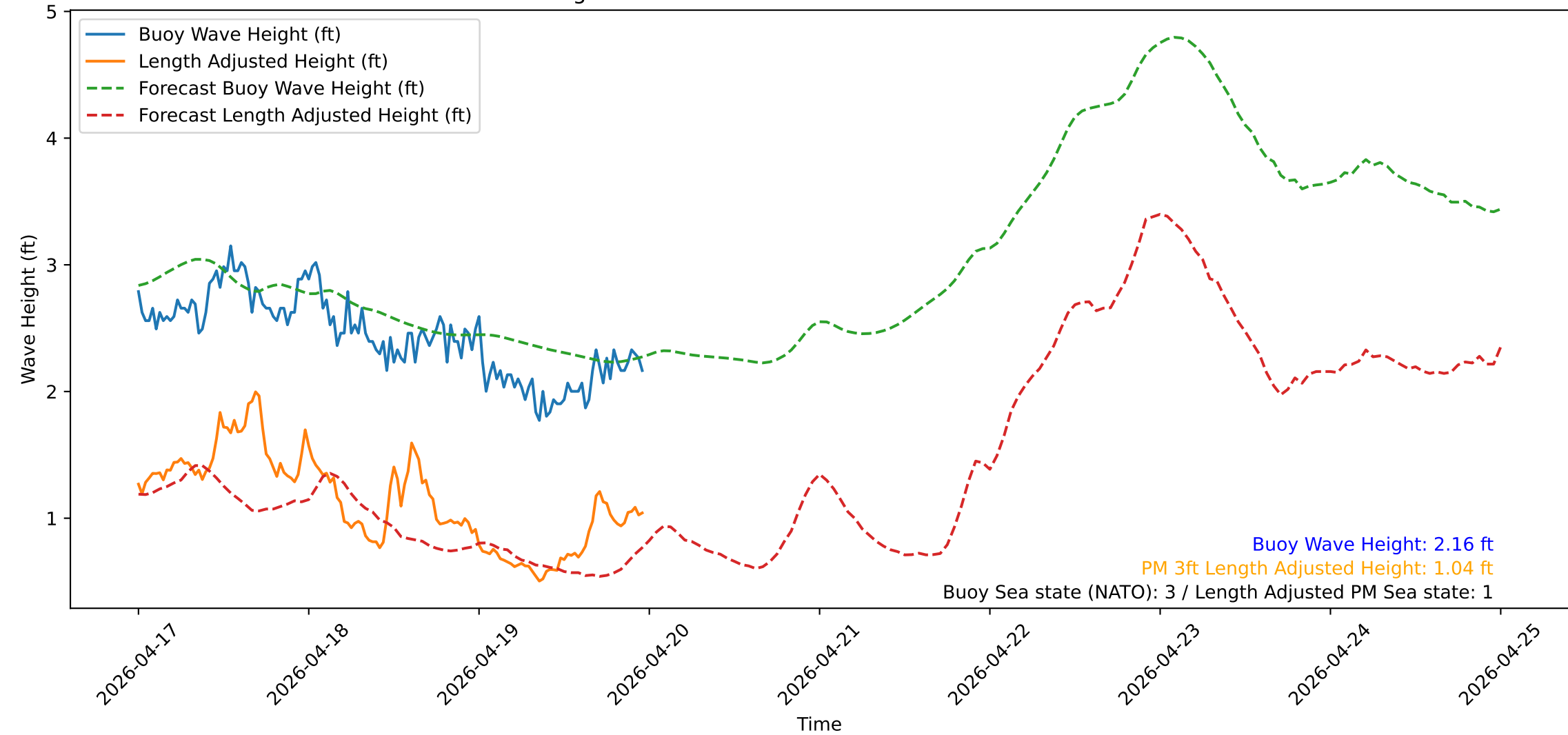
Wave Heights over Time for Red Beach at 2026-04-19 23:50:52
