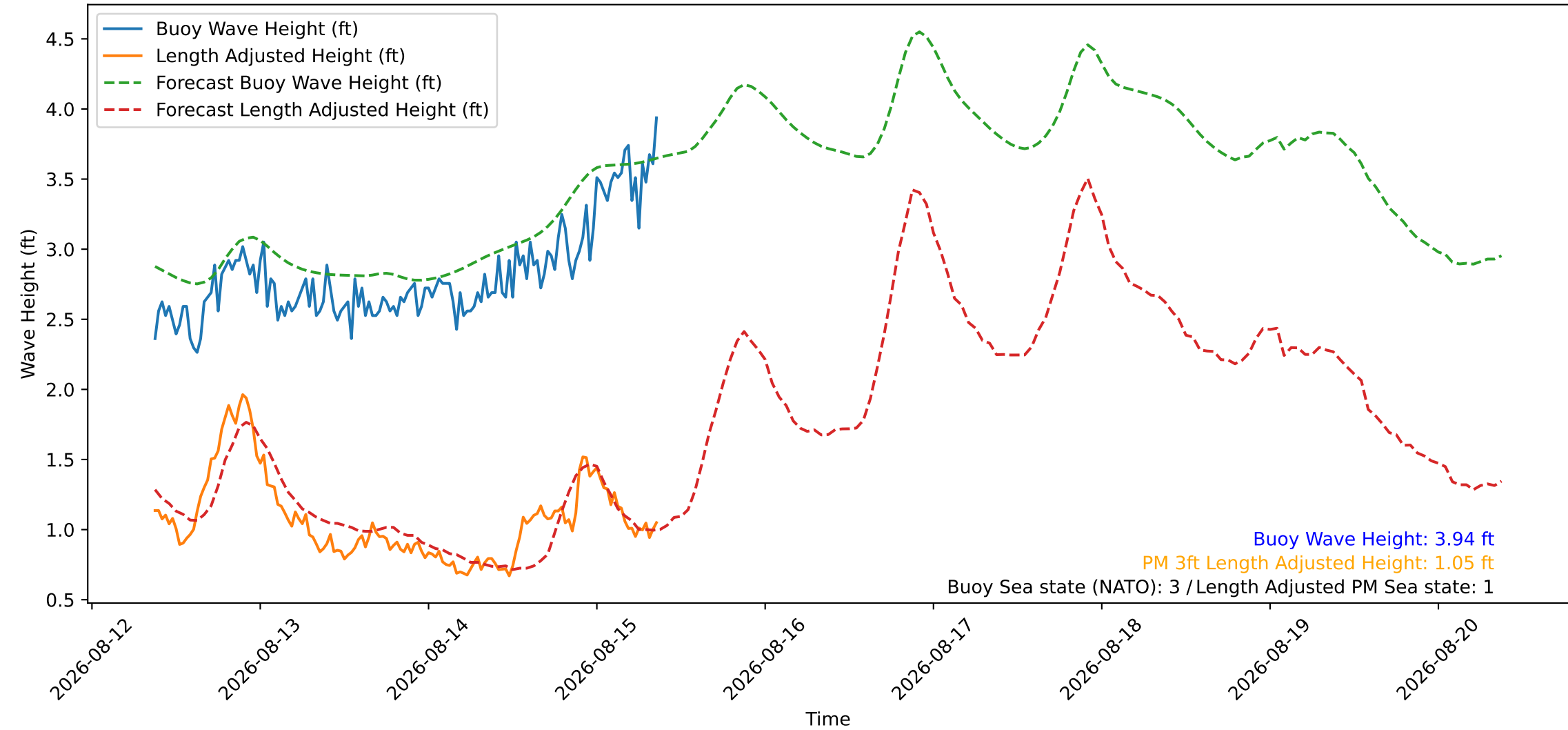
Wave Heights over Time for Green Beach at 2026-08-15 09:11:09
