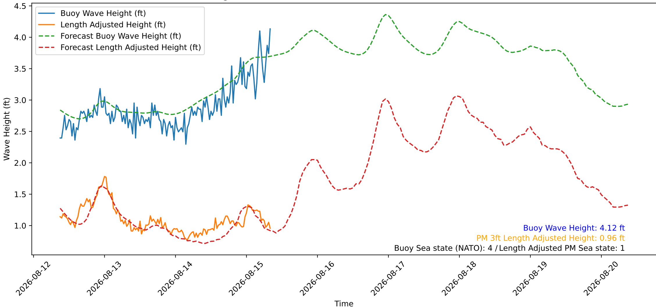
Wave Heights over Time for Oceanside Harbor at 2026-08-15 09:10:26
