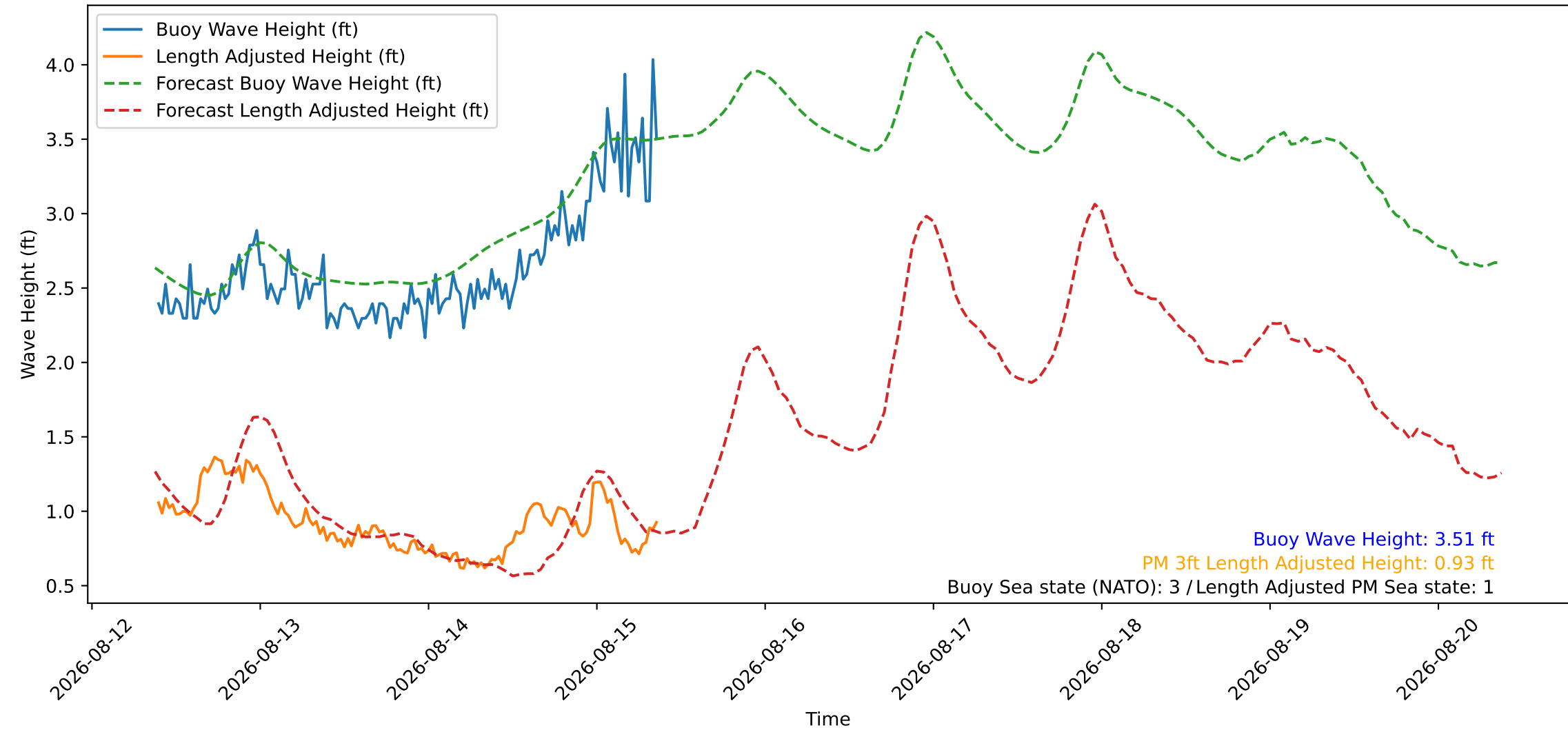
Wave Heights over Time for Red Beach at 2026-08-15 09:10:46
