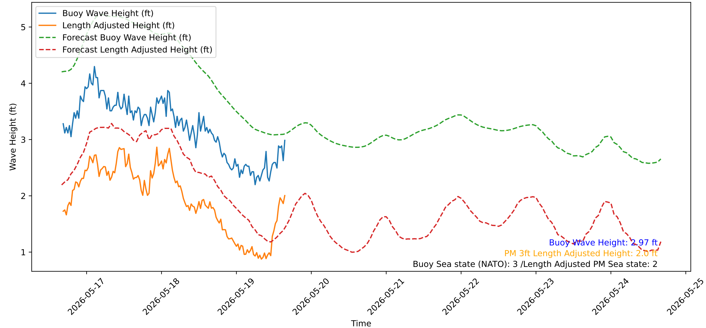
Wave Heights over Time for Oceanside Harbor at 2026-05-19 16:20:31
