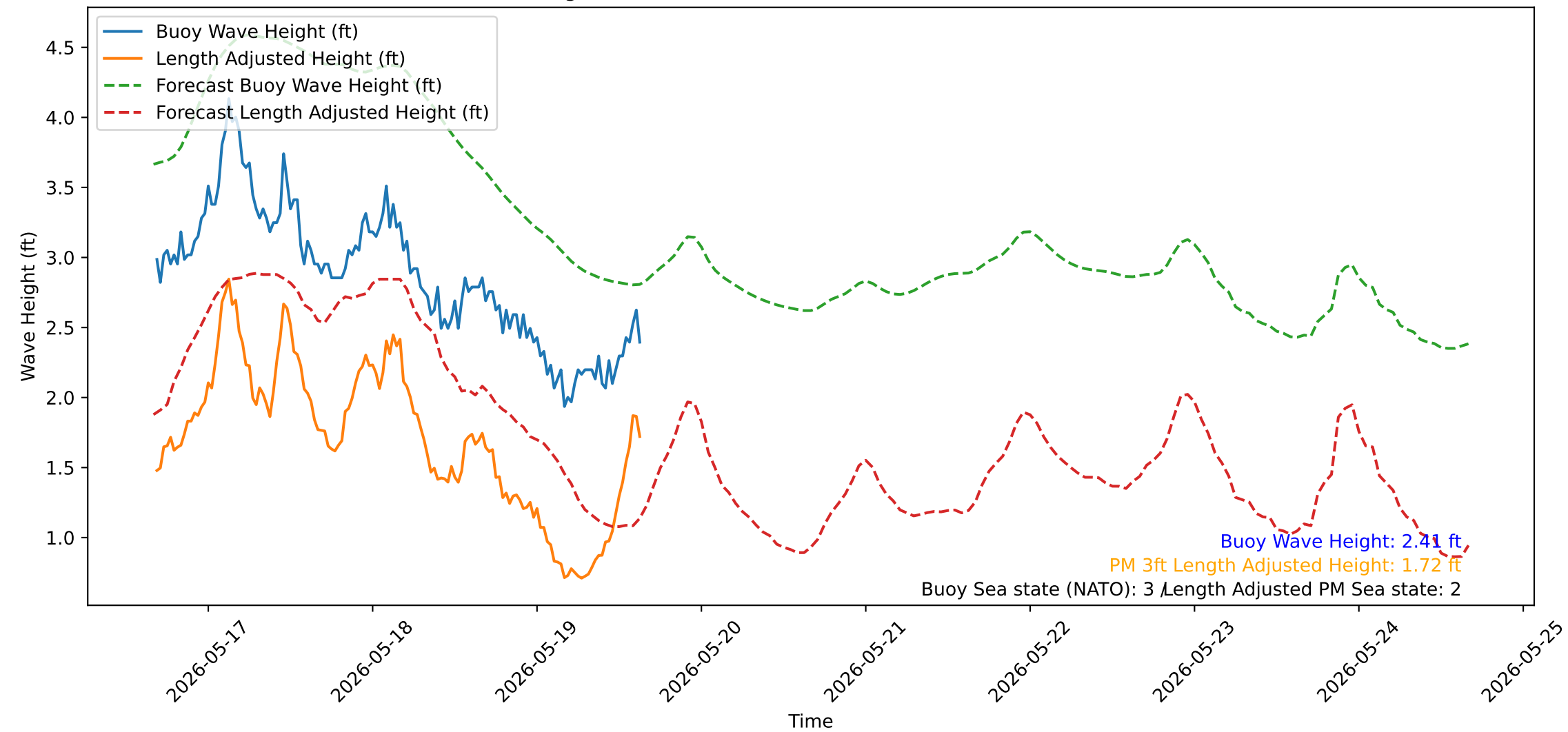
Wave Heights over Time for Red Beach at 2026-05-19 16:20:51
