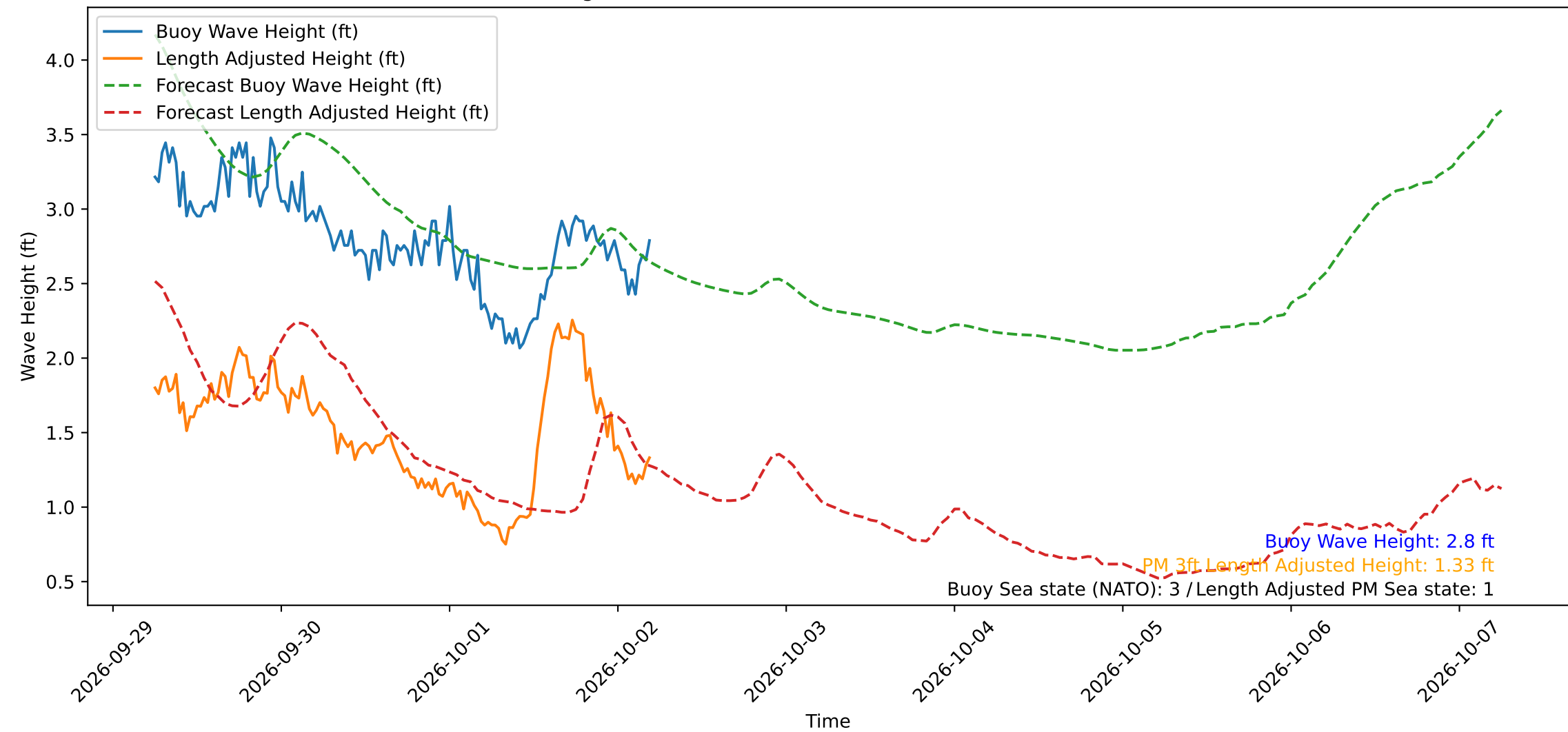
Wave Heights over Time for Red Beach at 2026-10-02 05:30:49
