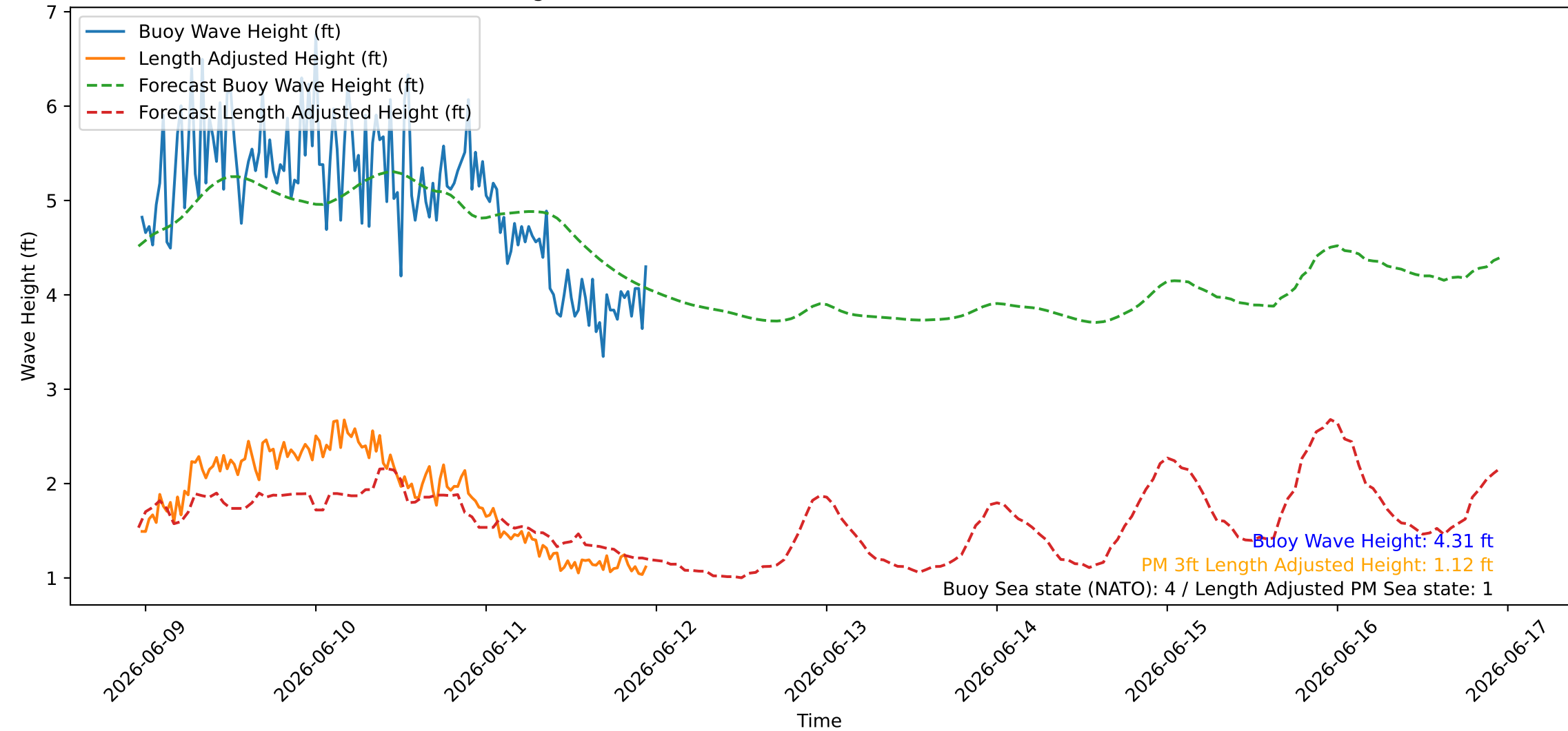
Wave Heights over Time for Oceanside Harbor at 2026-06-11 23:20:26
