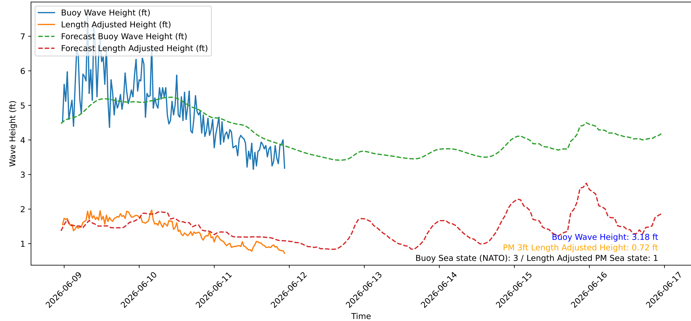
Wave Heights over Time for Red Beach at 2026-06-11 23:20:47
