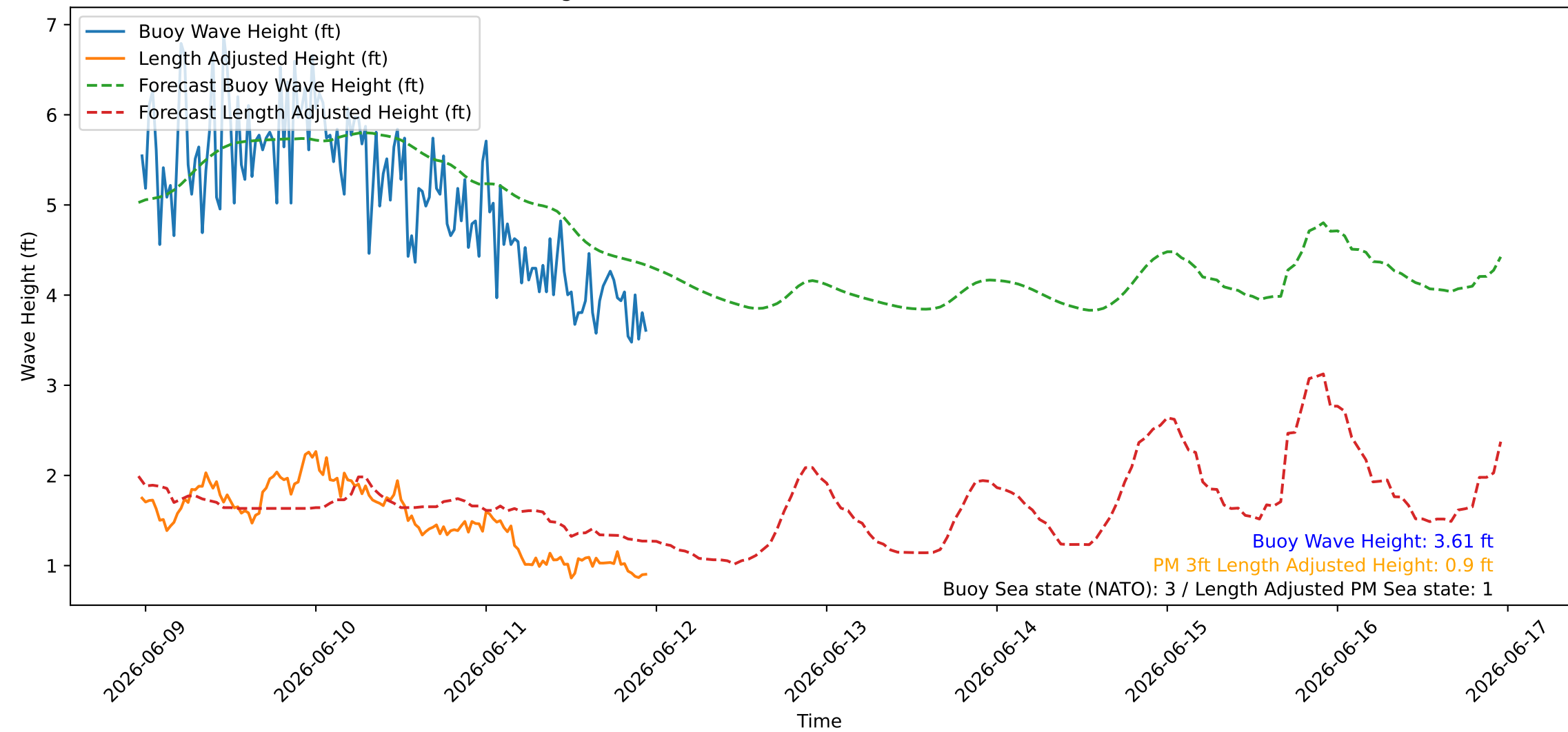
Wave Heights over Time for Green Beach at 2026-06-11 23:21:09
