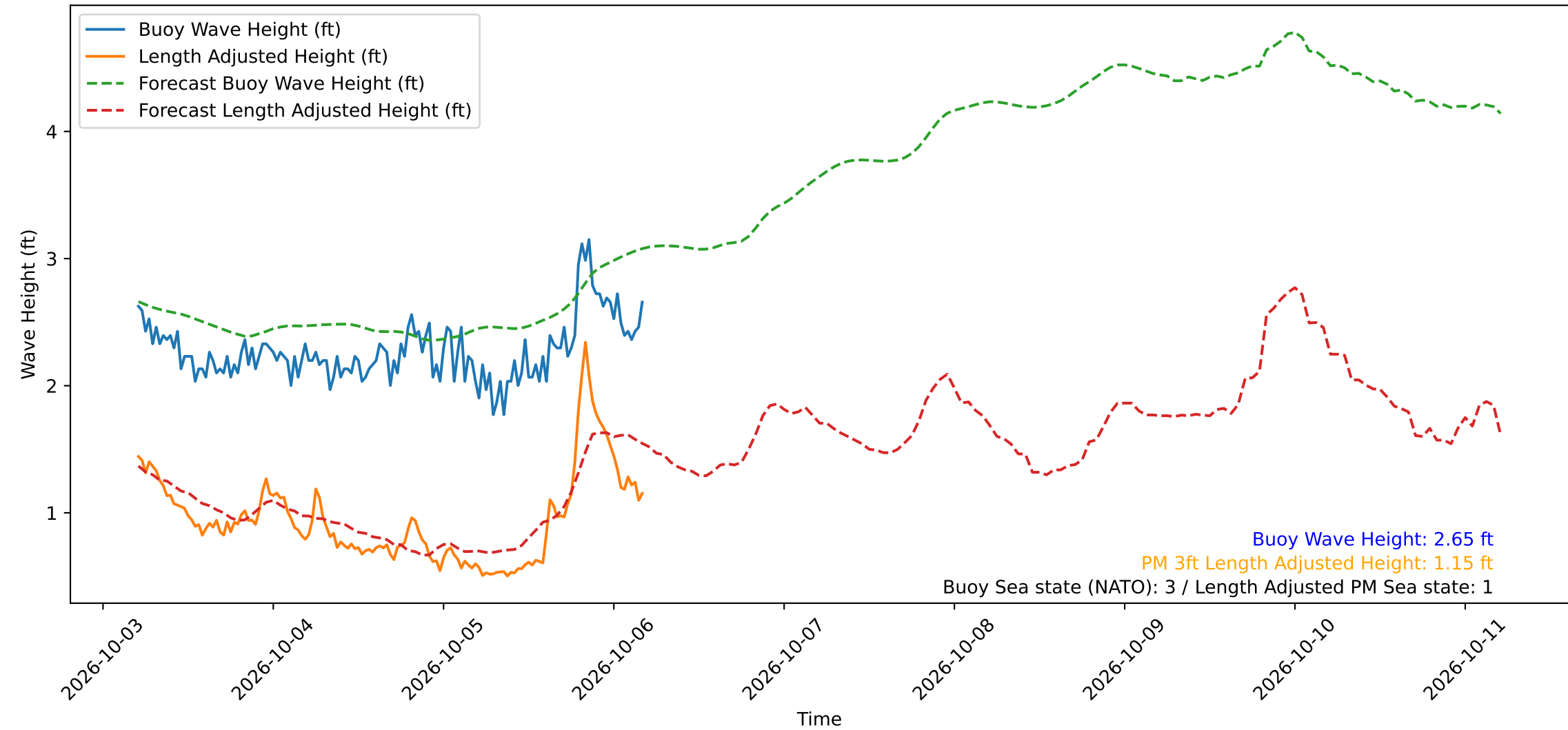
Wave Heights over Time for Green Beach at 2026-10-06 04:51:13
