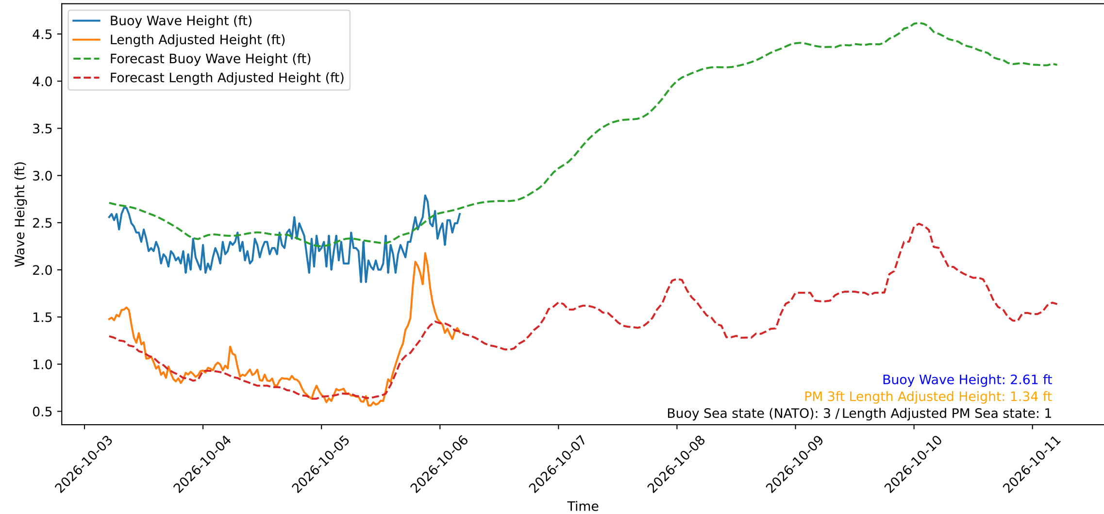
Wave Heights over Time for Oceanside Harbor at 2026-10-06 04:50:29
