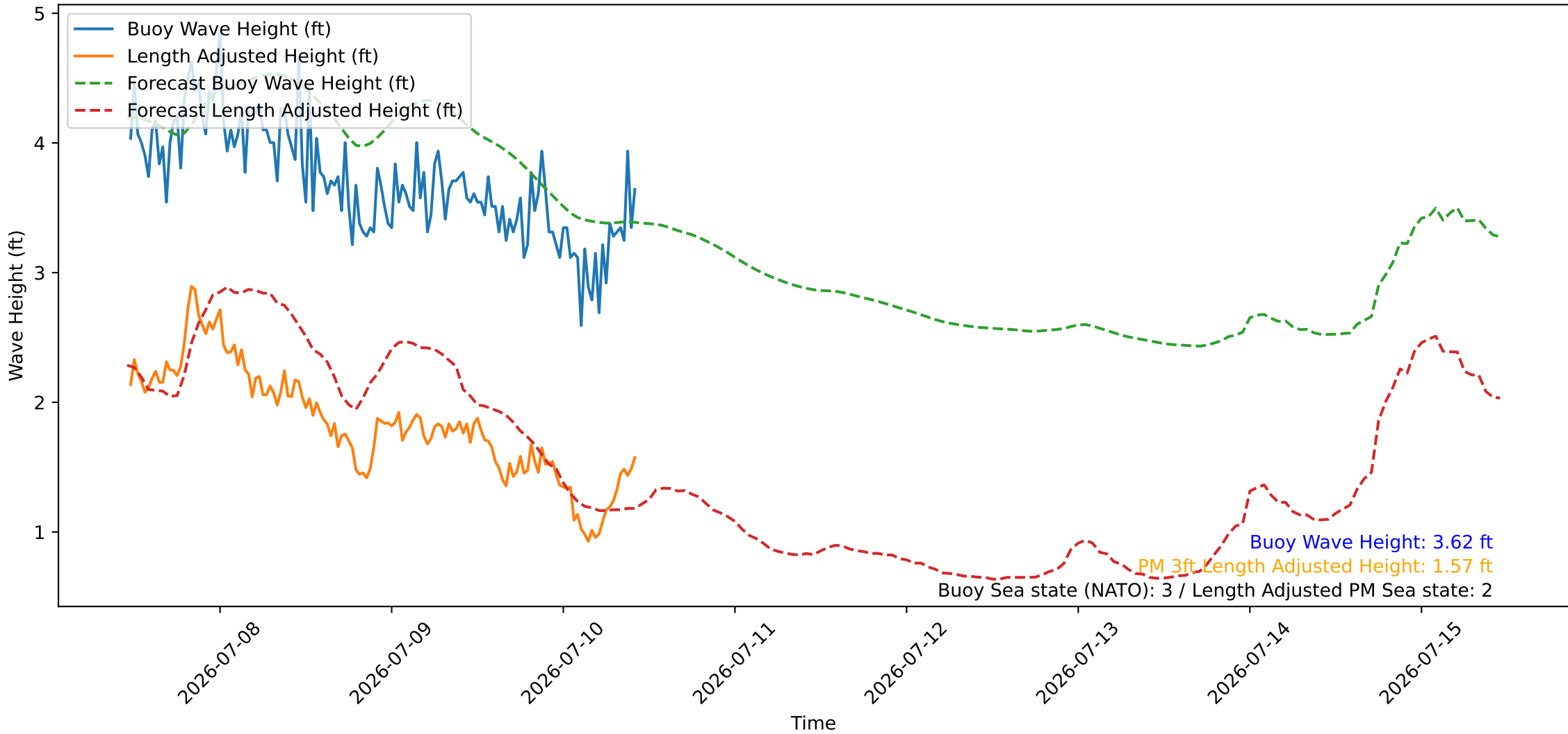
Wave Heights over Time for Red Beach at 2026-07-10 11:00:46
