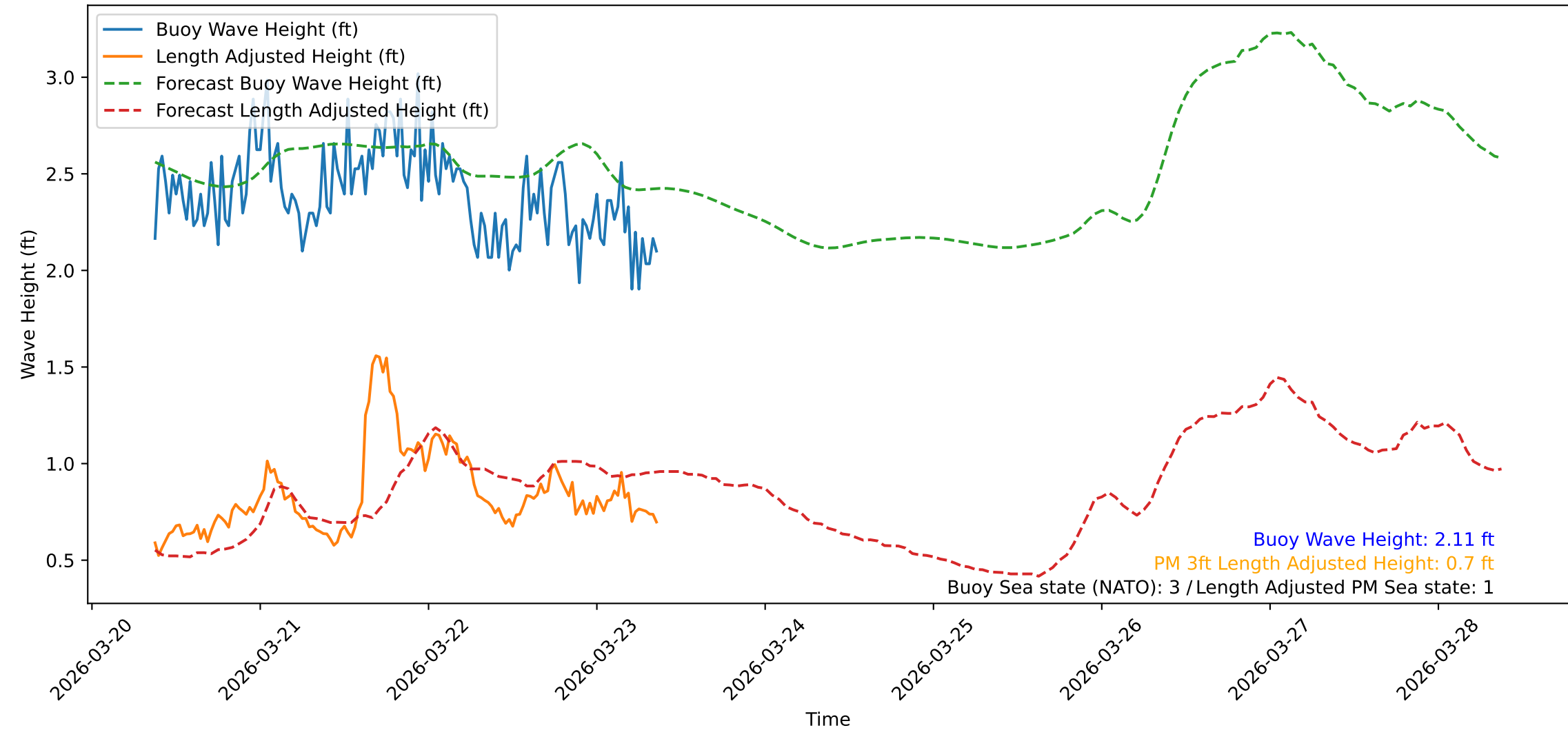
Wave Heights over Time for Oceanside Harbor at 2026-03-23 09:10:32
