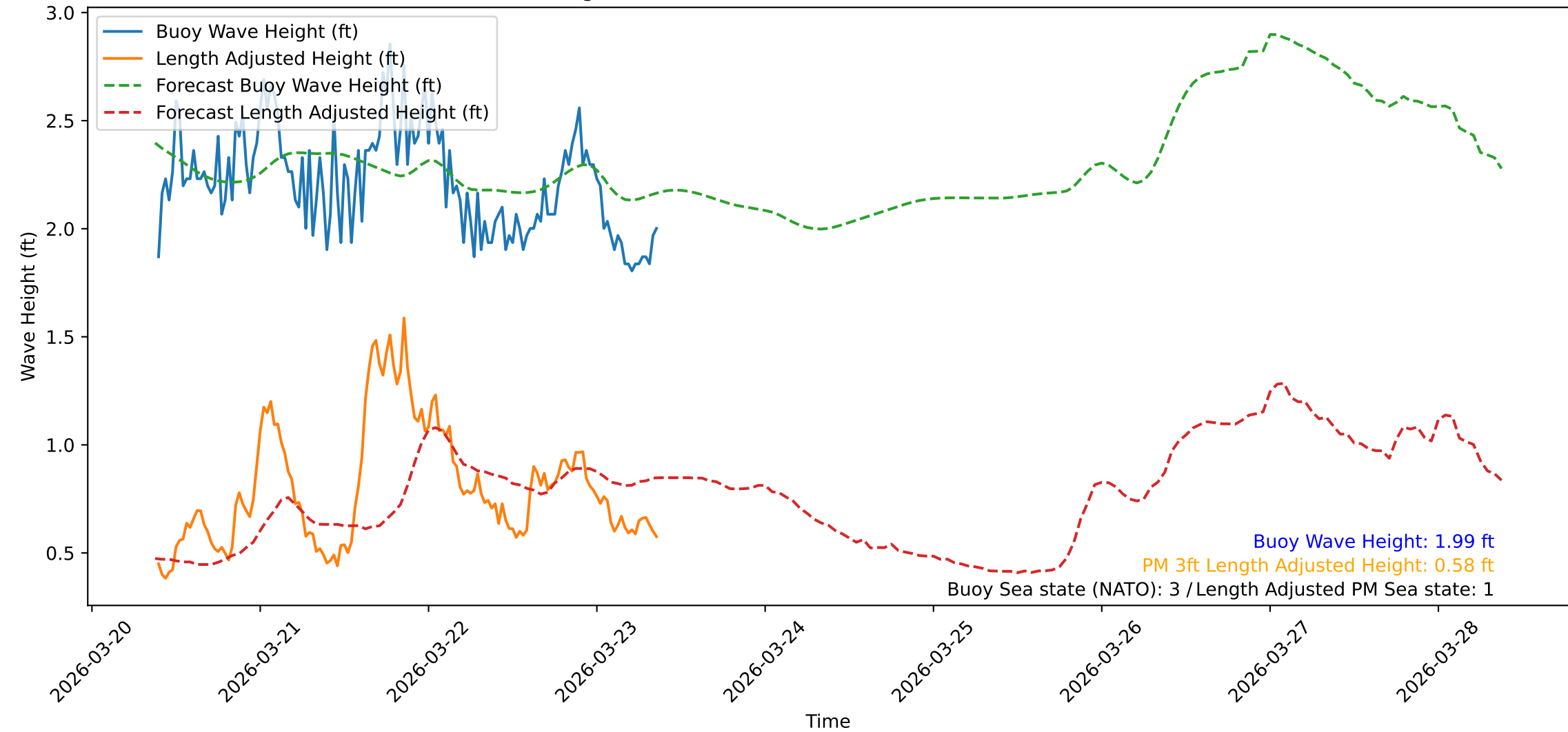
Wave Heights over Time for Red Beach at 2026-03-23 09:10:48
