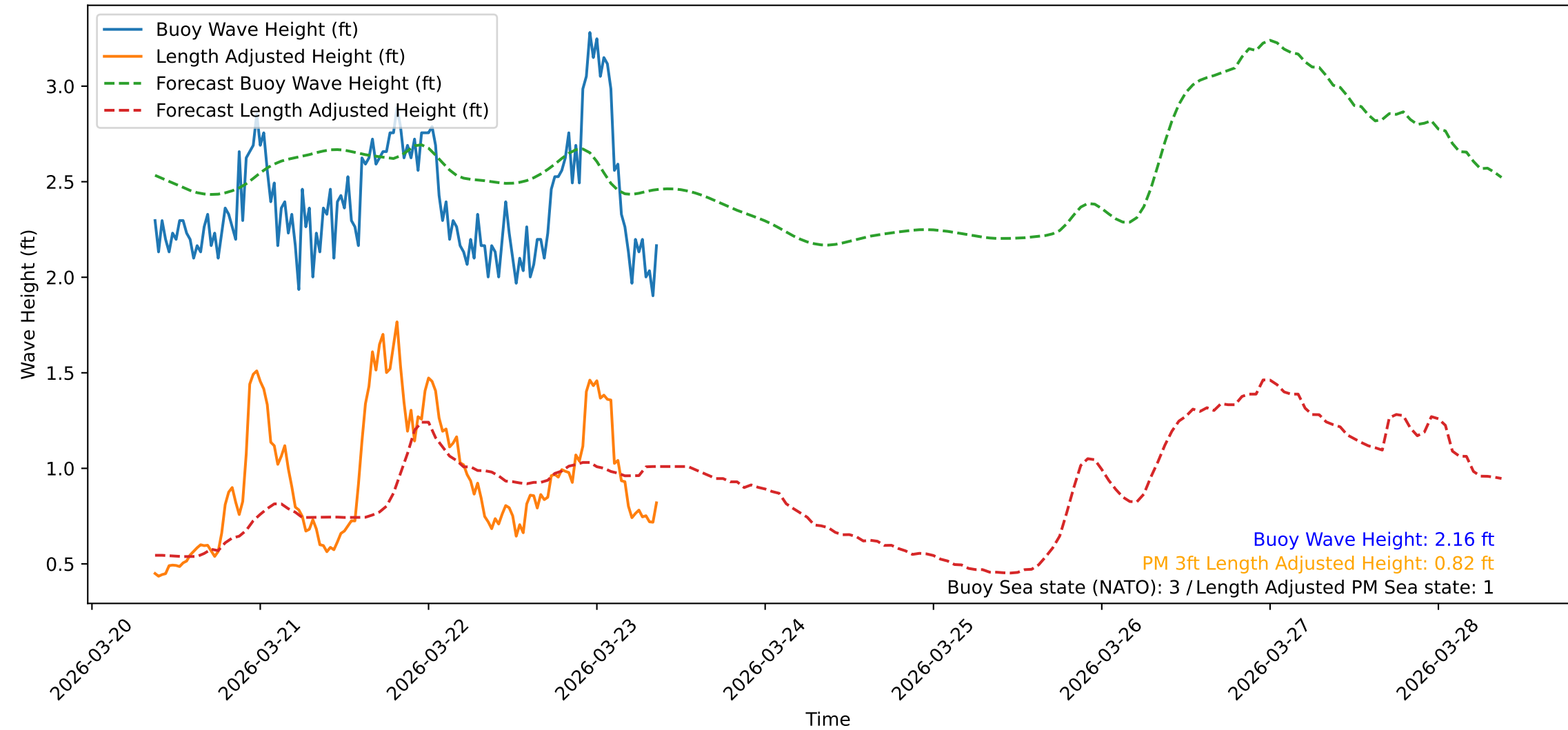
Wave Heights over Time for Green Beach at 2026-03-23 09:11:10
