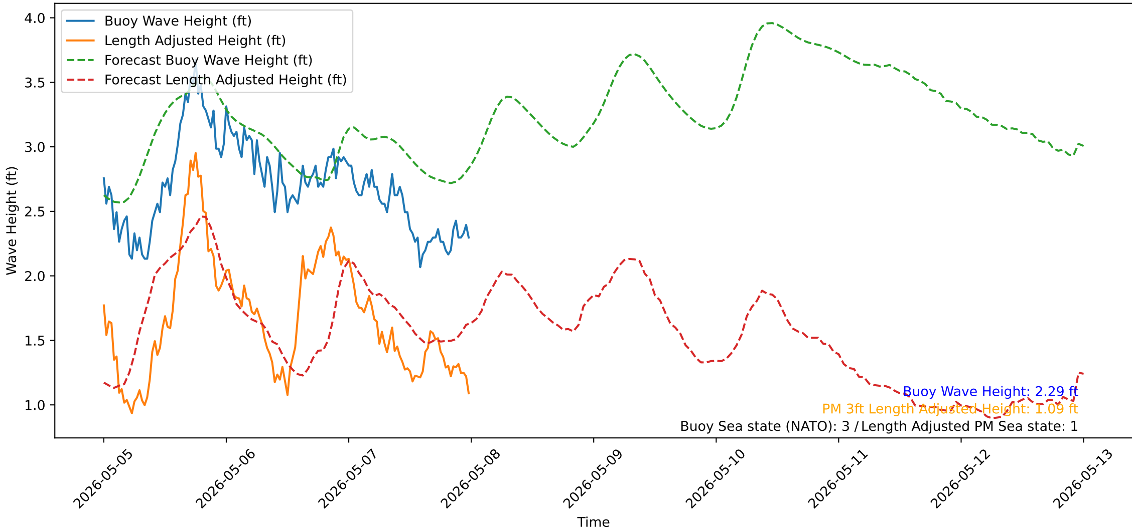
Wave Heights over Time for Green Beach at 2026-05-08 00:11:13
