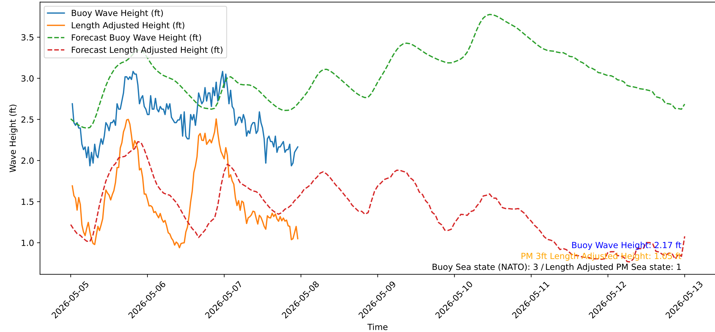
Wave Heights over Time for Red Beach at 2026-05-08 00:10:51
