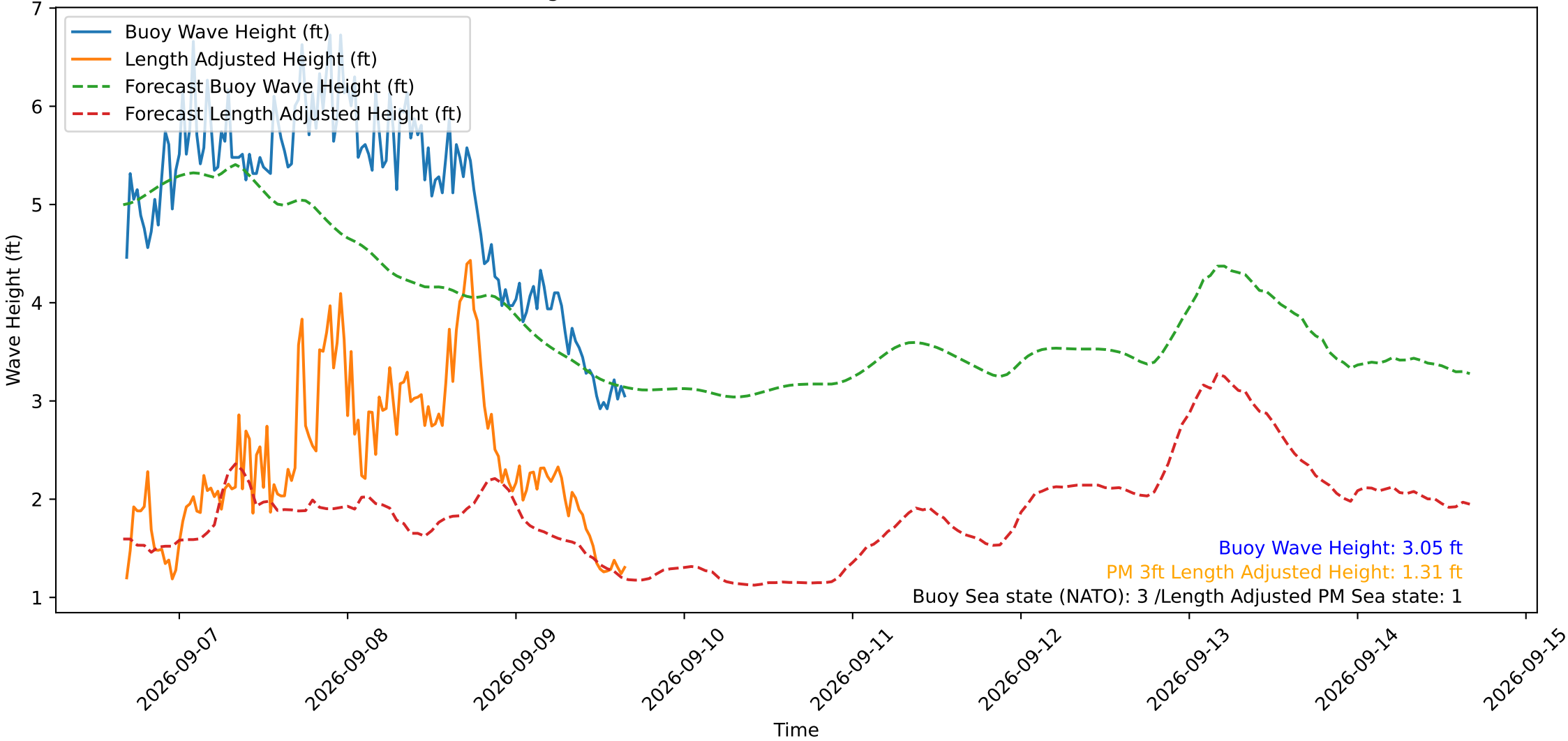
Wave Heights over Time for Red Beach at 2026-09-09 16:10:50
