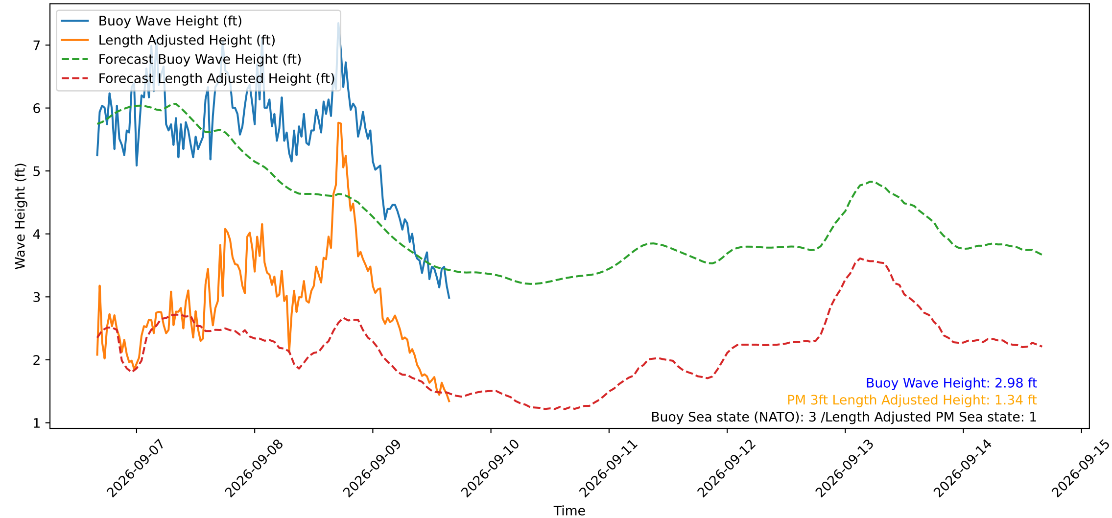
Wave Heights over Time for Oceanside Harbor at 2026-09-09 16:10:30
