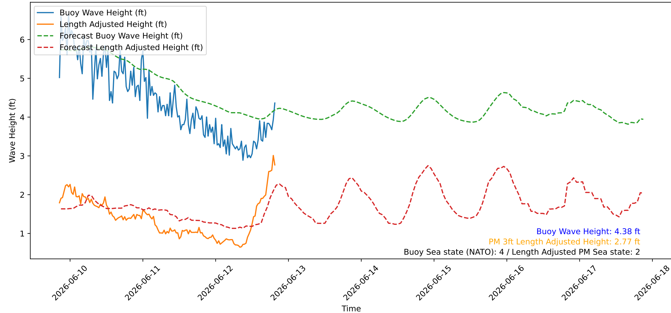
Wave Heights over Time for Green Beach at 2026-06-12 20:31:08
