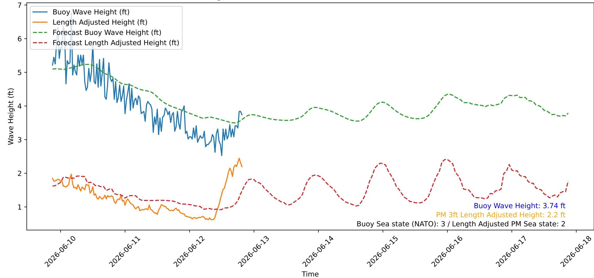
Wave Heights over Time for Red Beach at 2026-06-12 20:30:46
