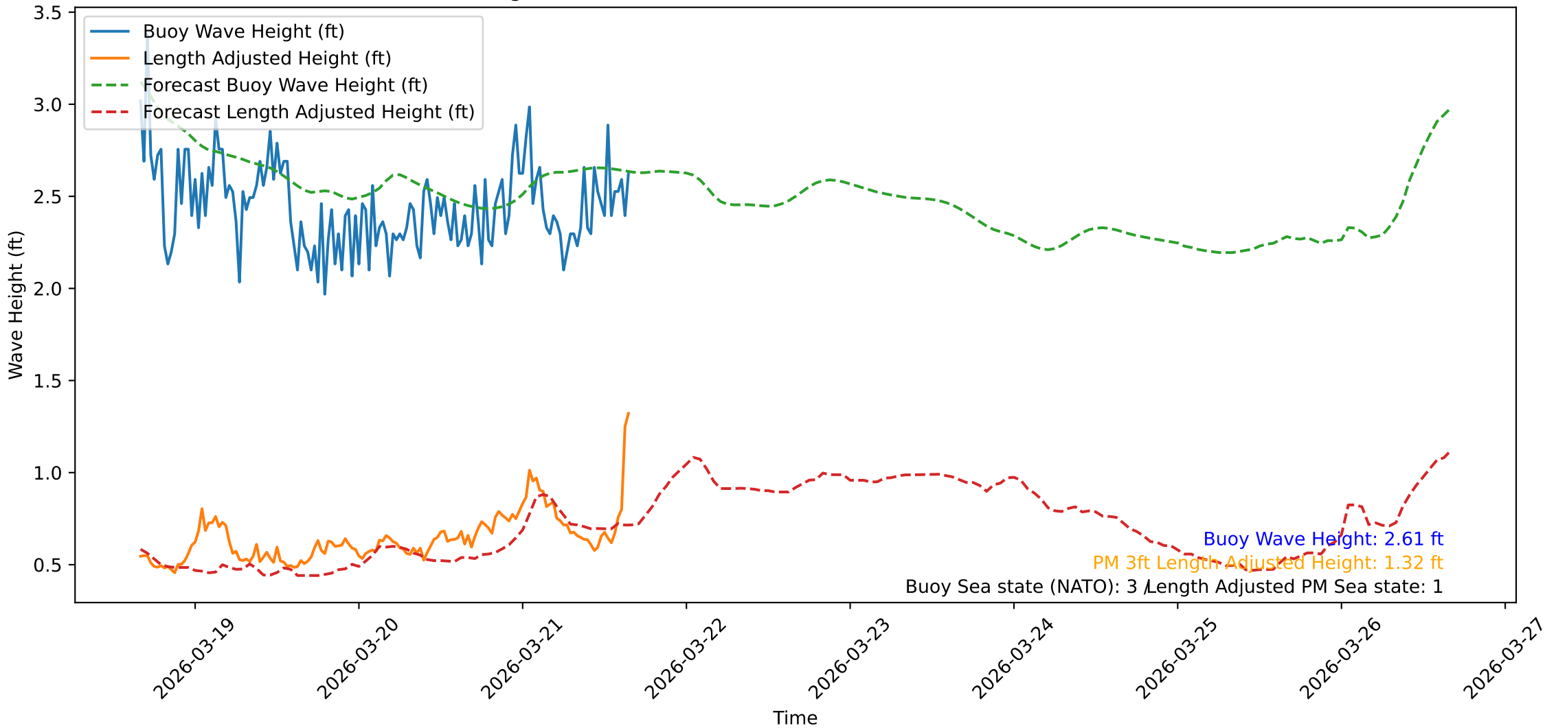
Wave Heights over Time for Oceanside Harbor at 2026-03-21 16:10:31
