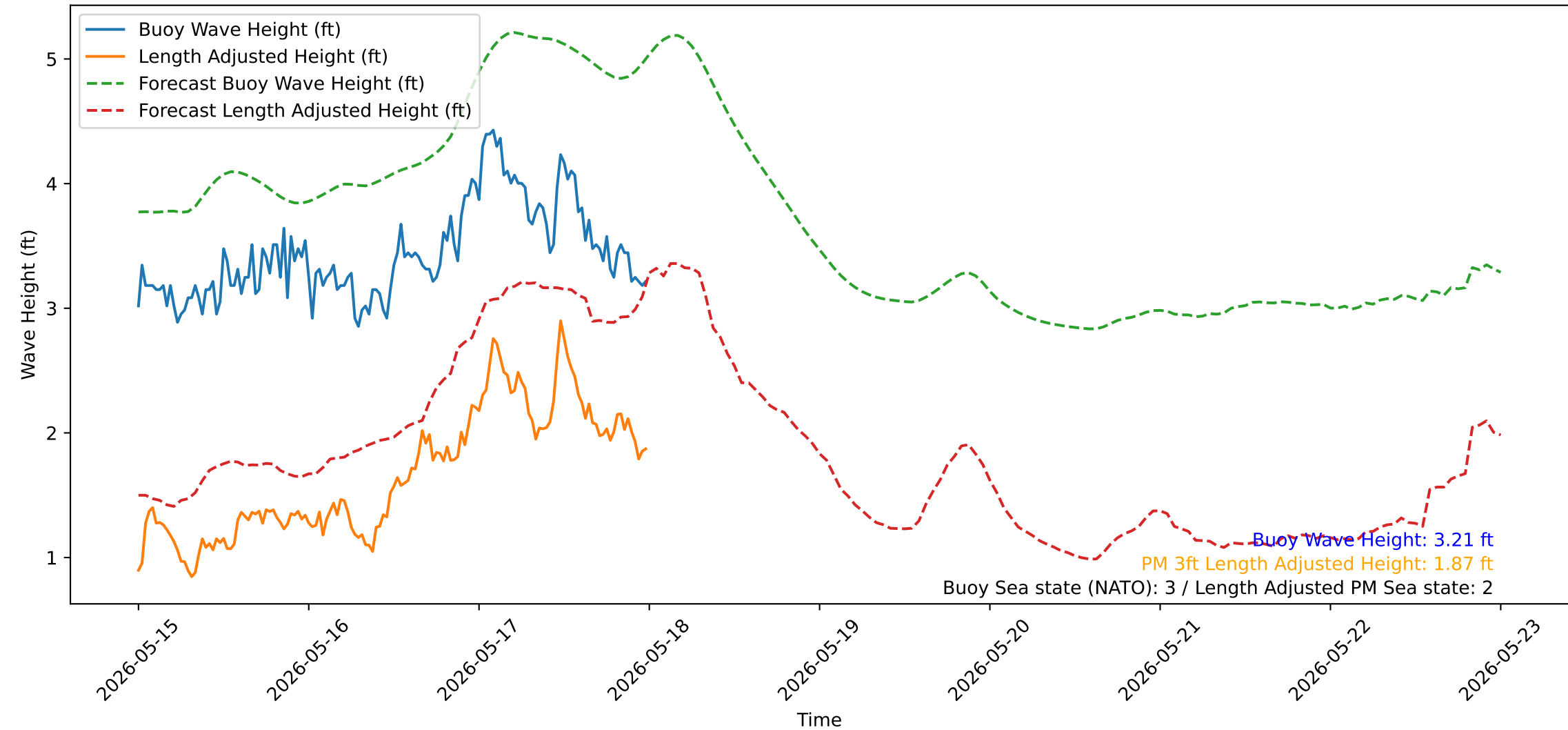
Wave Heights over Time for Green Beach at 2026-05-18 00:11:13
