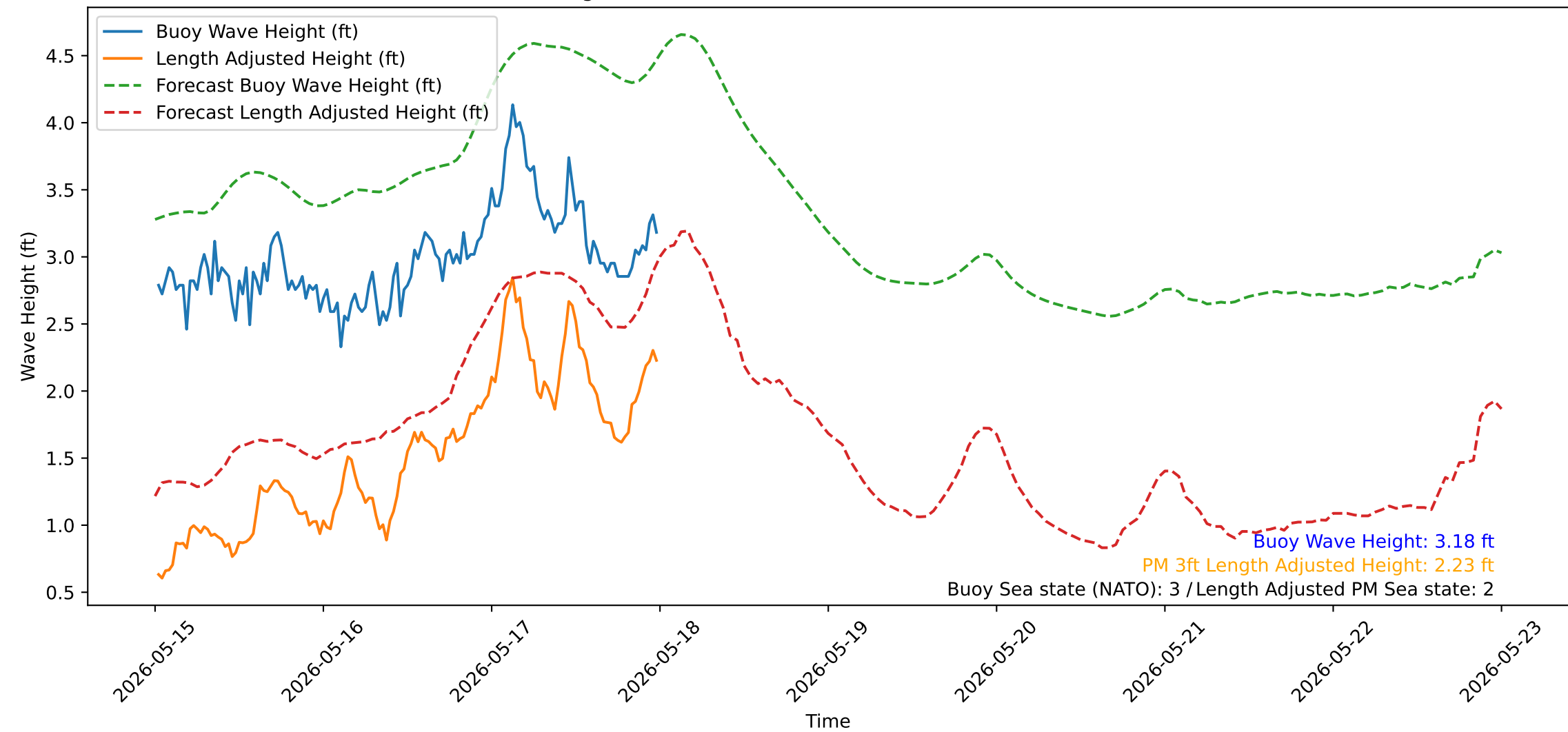
Wave Heights over Time for Red Beach at 2026-05-18 00:10:51
