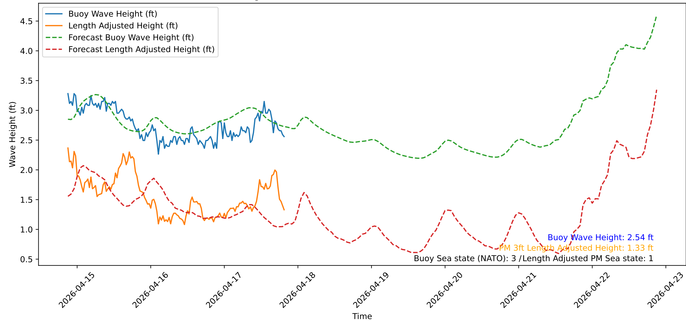
Wave Heights over Time for Red Beach at 2026-04-17 20:30:51
