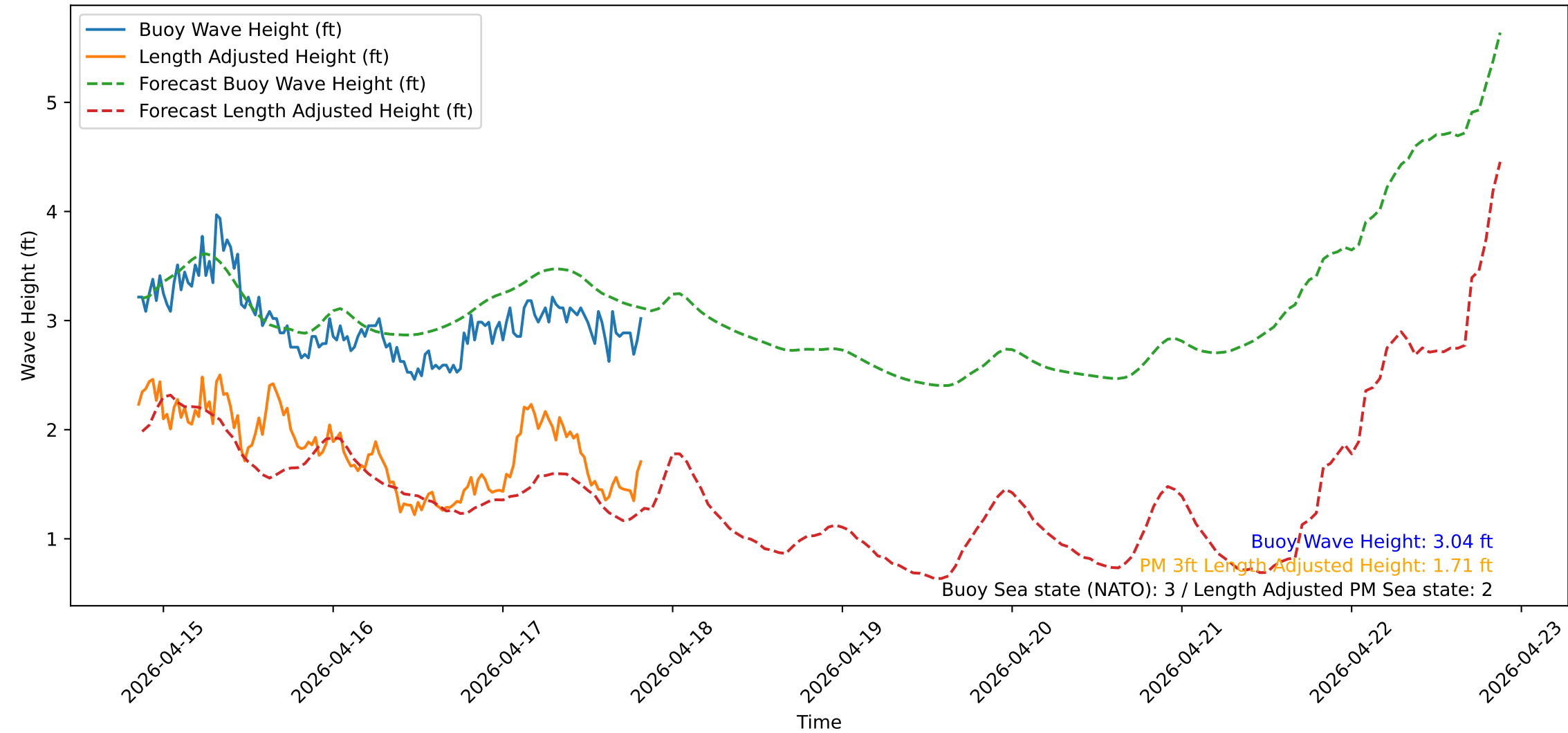
Wave Heights over Time for Green Beach at 2026-04-17 20:31:13
