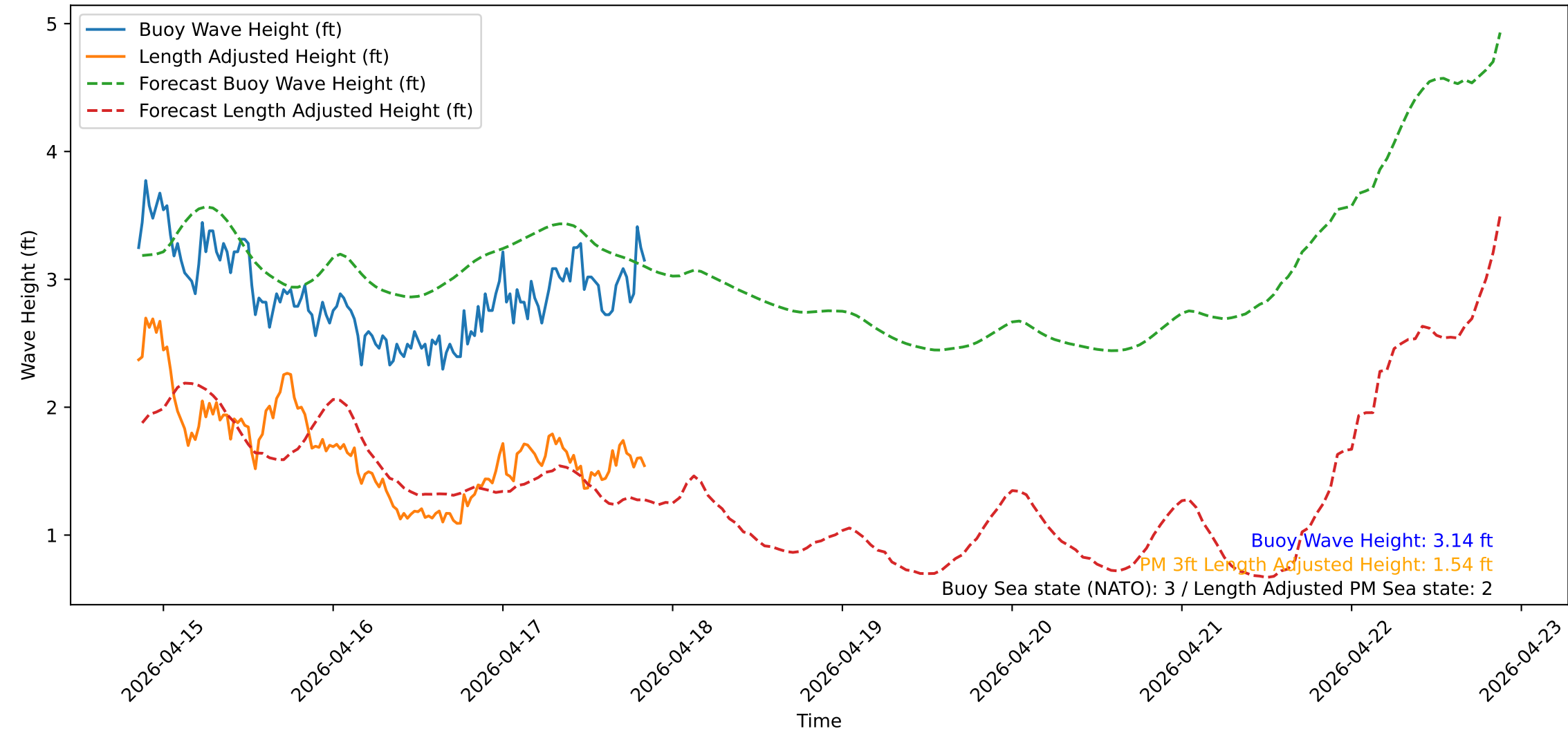
Wave Heights over Time for Oceanside Harbor at 2026-04-17 20:30:32
