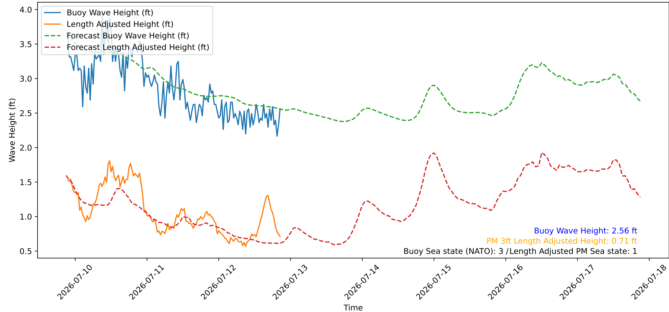
Wave Heights over Time for Red Beach at 2026-07-12 21:20:47
