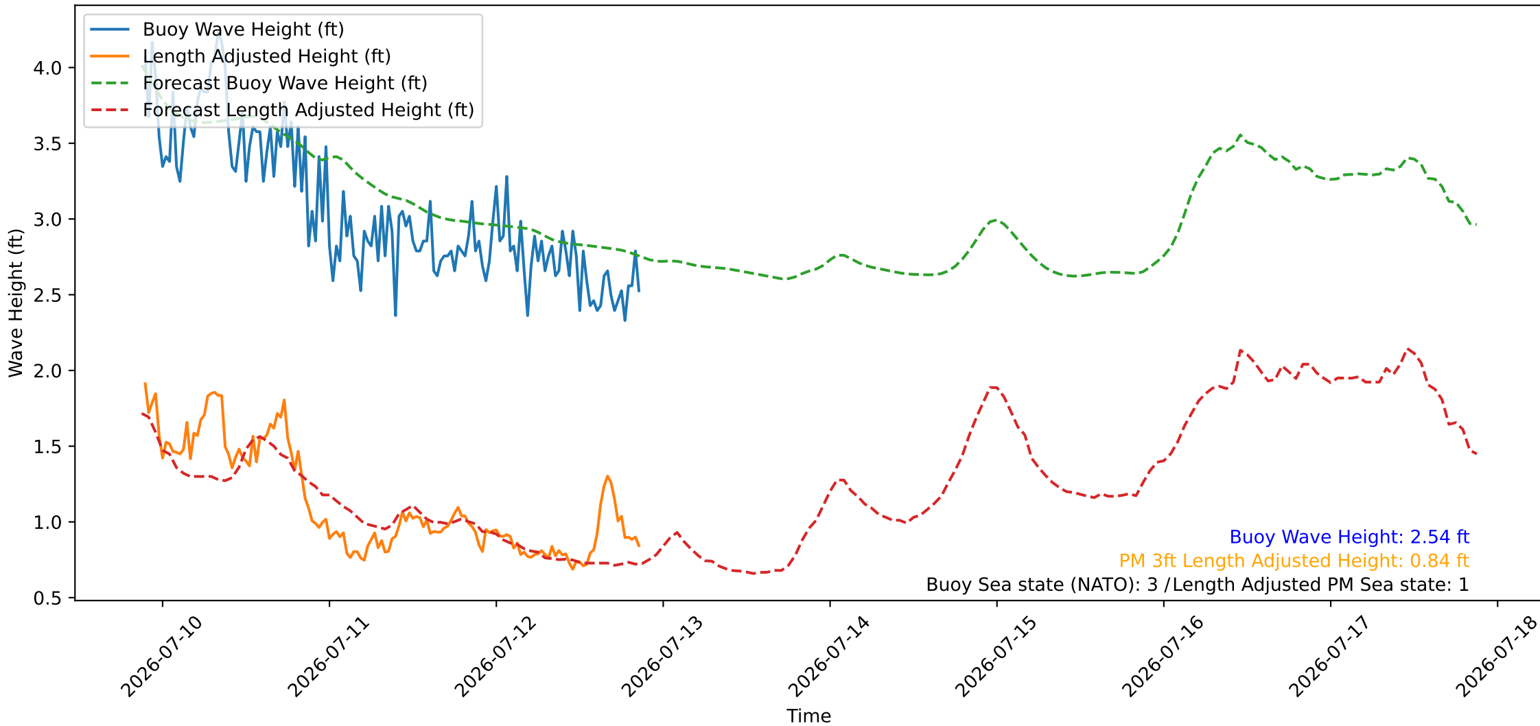
Wave Heights over Time for Oceanside Harbor at 2026-07-12 21:20:26
