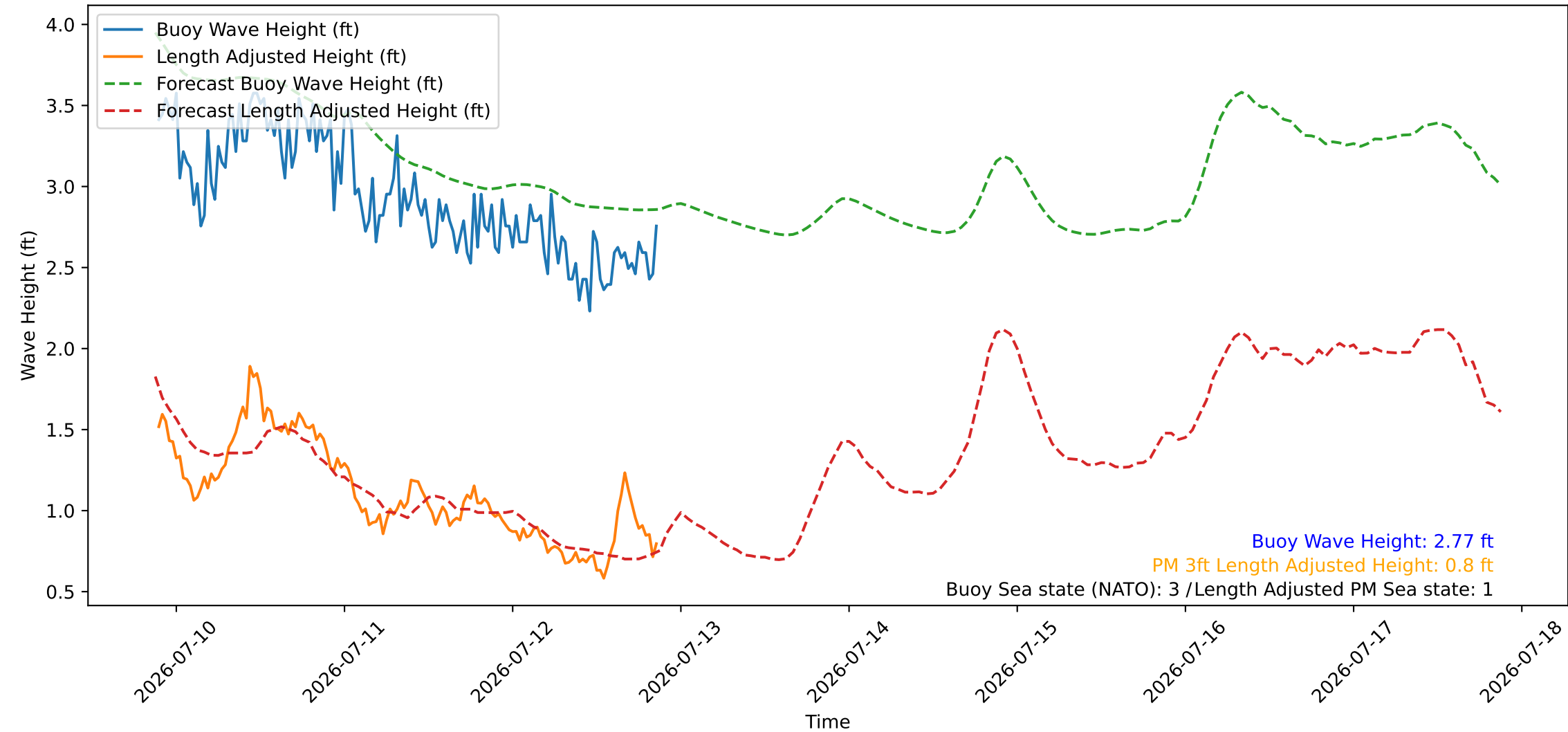
Wave Heights over Time for Green Beach at 2026-07-12 21:21:09
