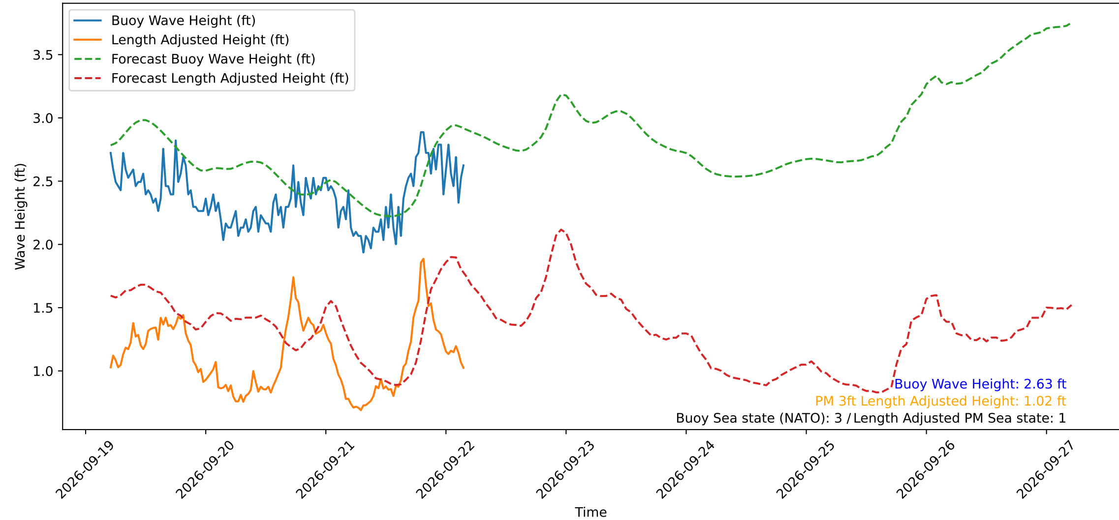
Wave Heights over Time for Red Beach at 2026-09-22 04:30:49
