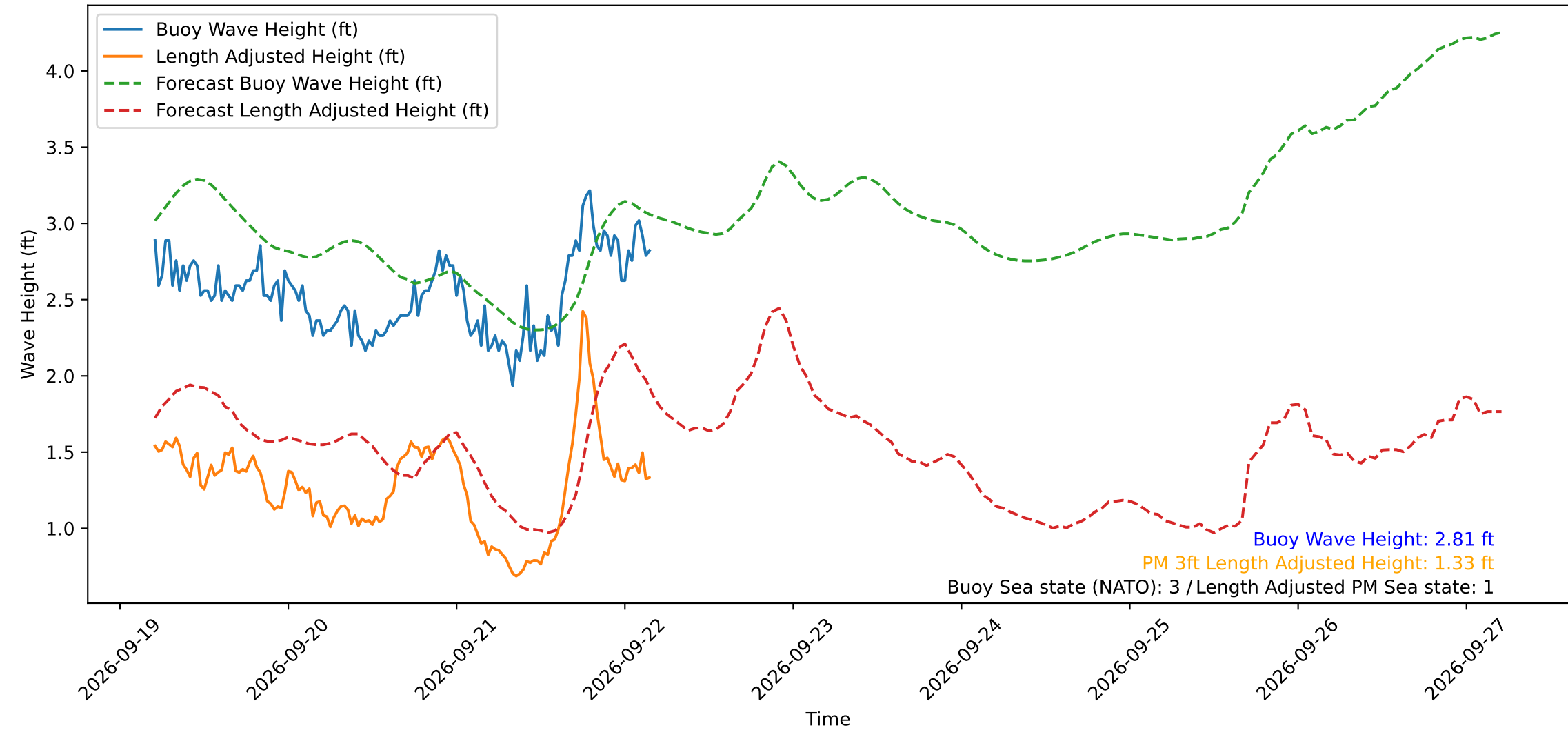
Wave Heights over Time for Green Beach at 2026-09-22 04:31:11
