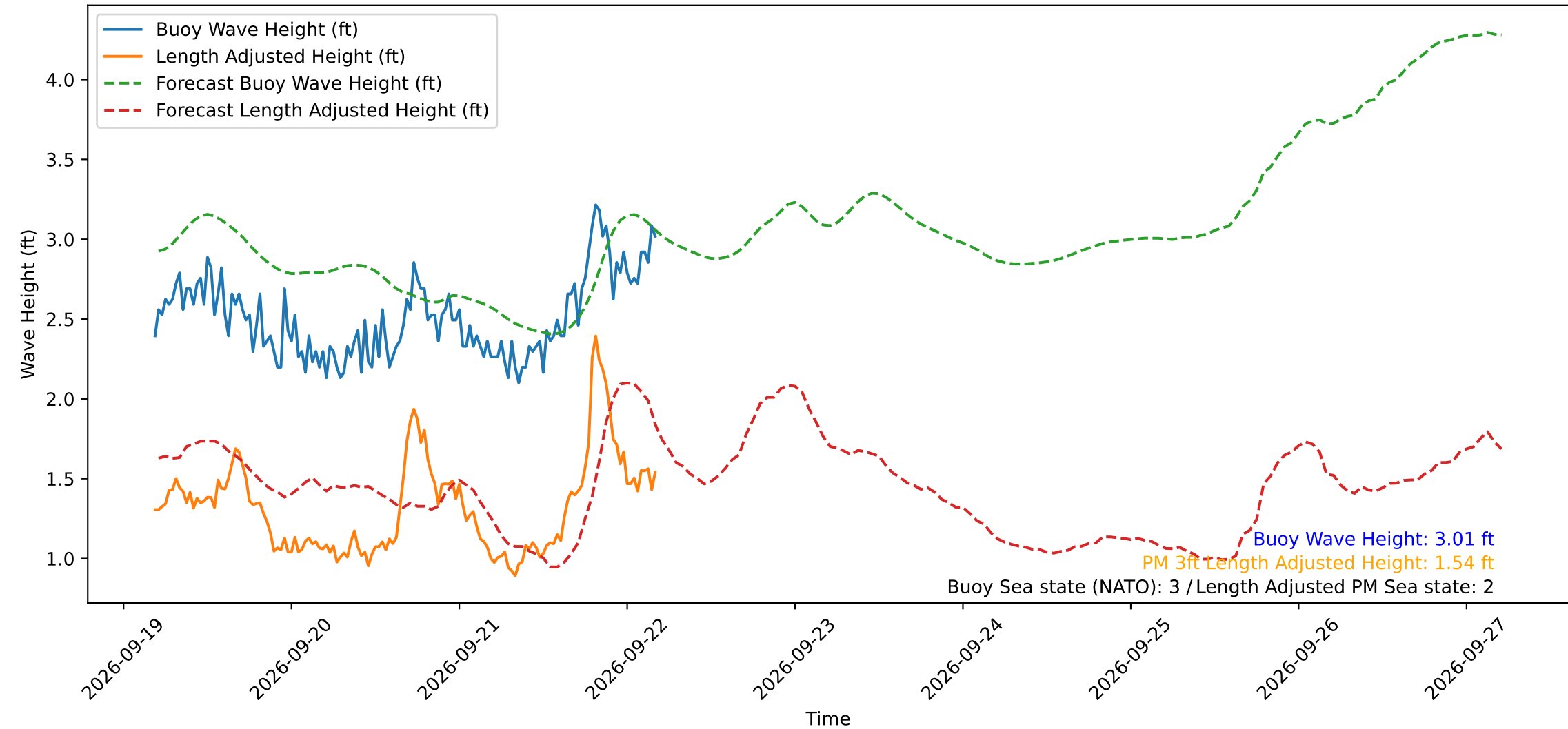
Wave Heights over Time for Oceanside Harbor at 2026-09-22 04:30:29
