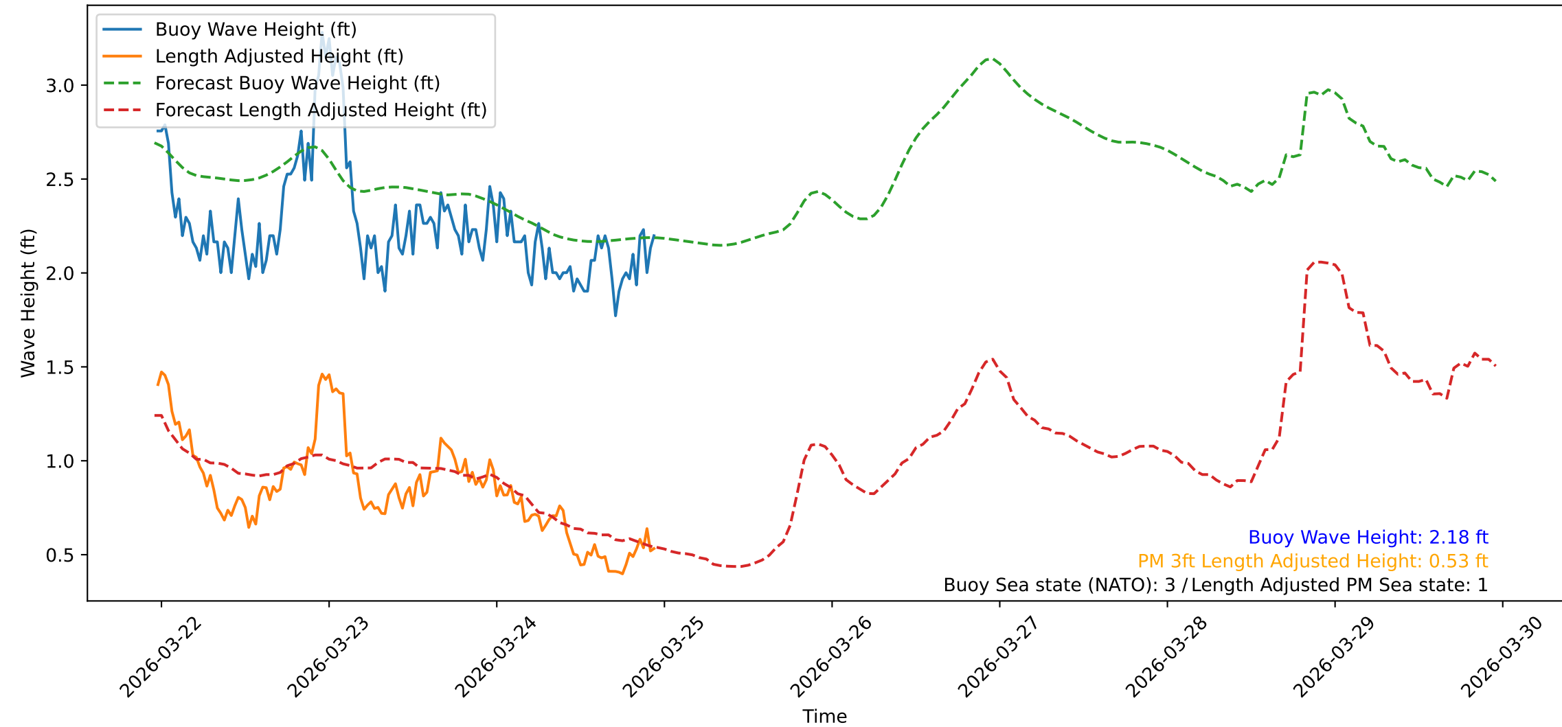
Wave Heights over Time for Green Beach at 2026-03-24 23:21:09
