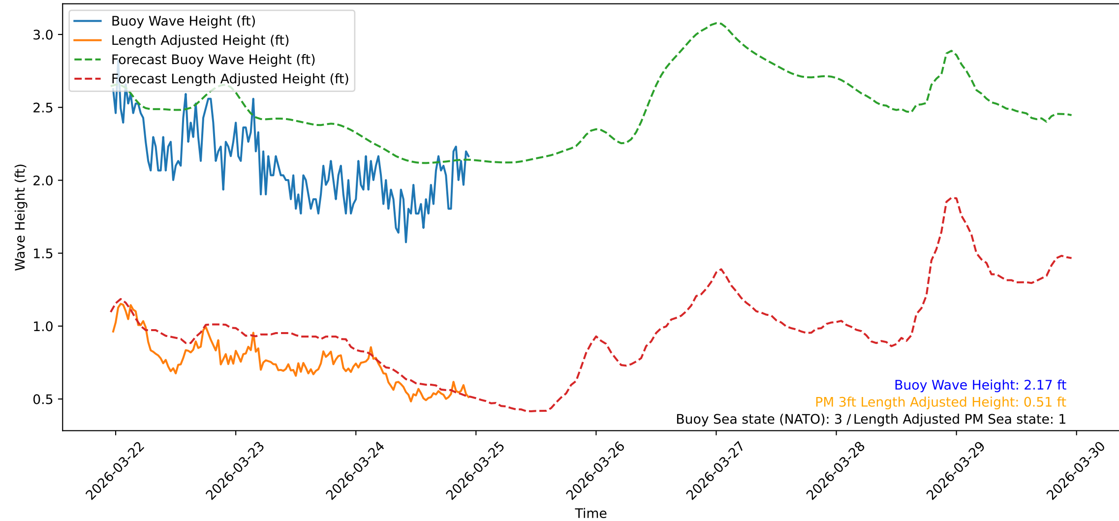
Wave Heights over Time for Oceanside Harbor at 2026-03-24 23:20:31
