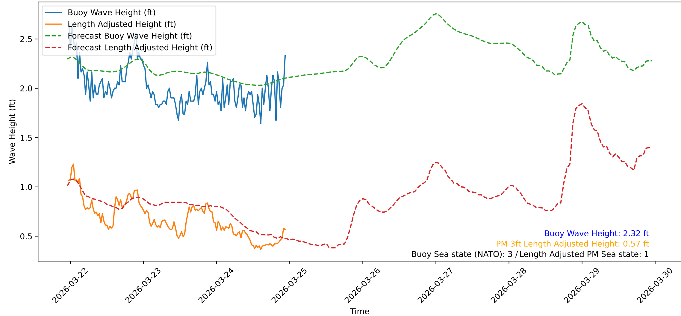
Wave Heights over Time for Red Beach at 2026-03-24 23:20:47
