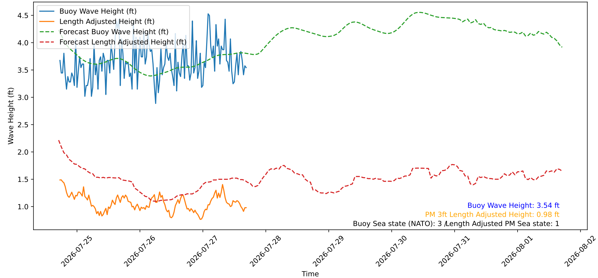
Wave Heights over Time for Red Beach at 2026-07-27 17:20:48
