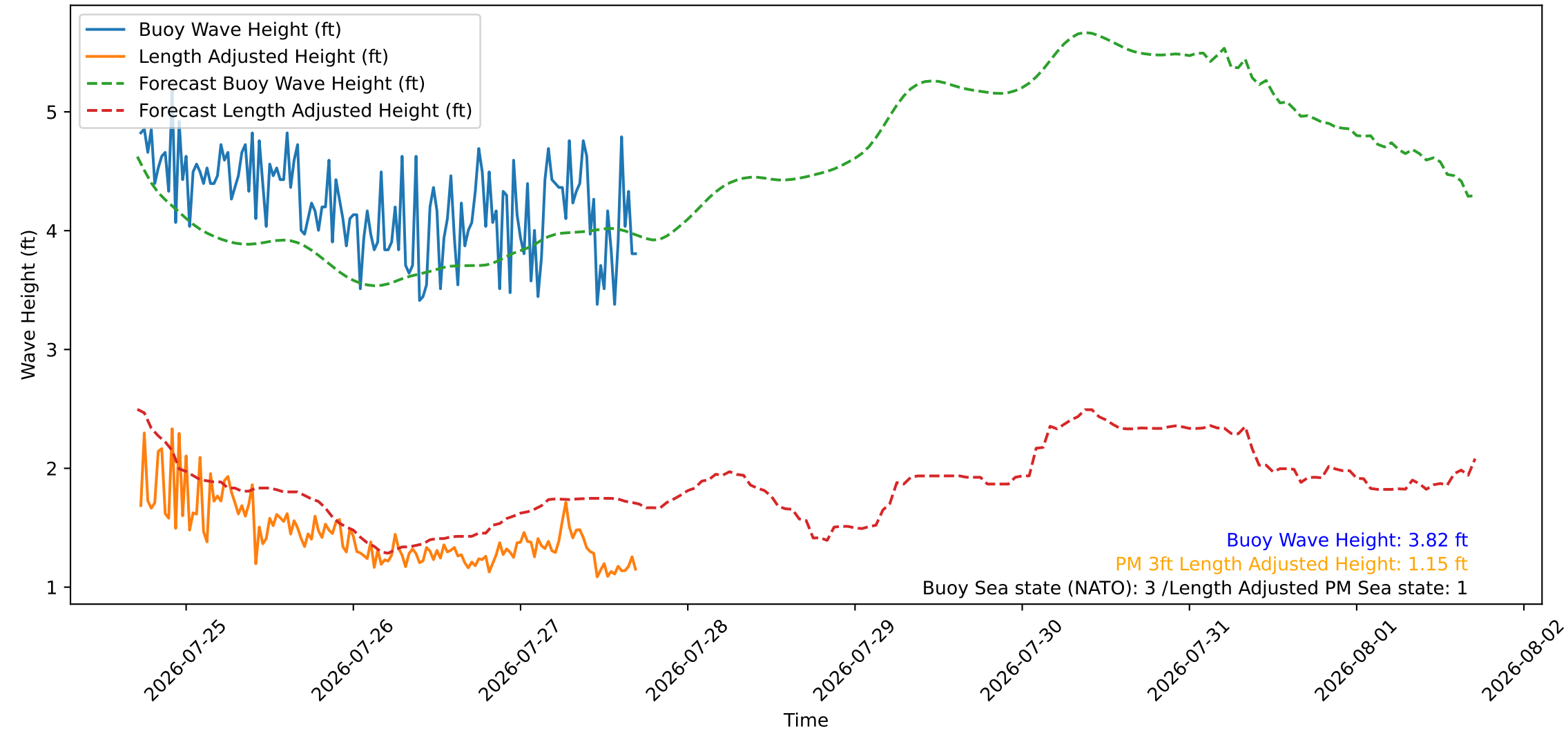
Wave Heights over Time for Green Beach at 2026-07-27 17:21:11
