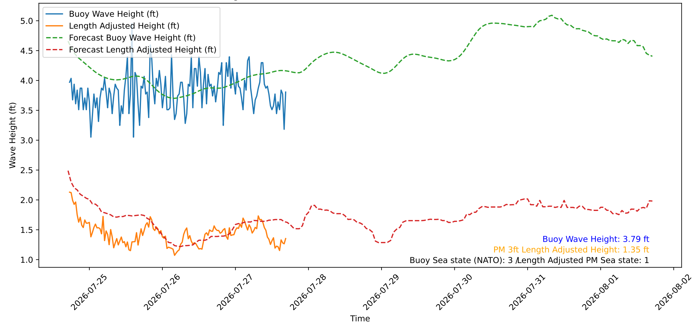
Wave Heights over Time for Oceanside Harbor at 2026-07-27 17:20:26
