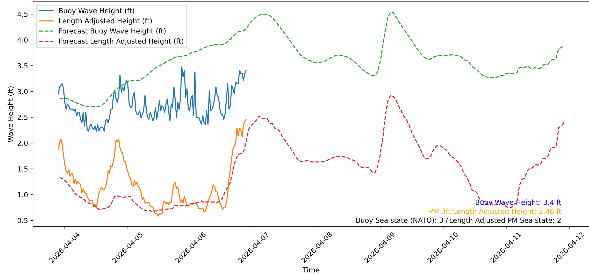
Wave Heights over Time for Green Beach at 2026-04-06 21:41:10
