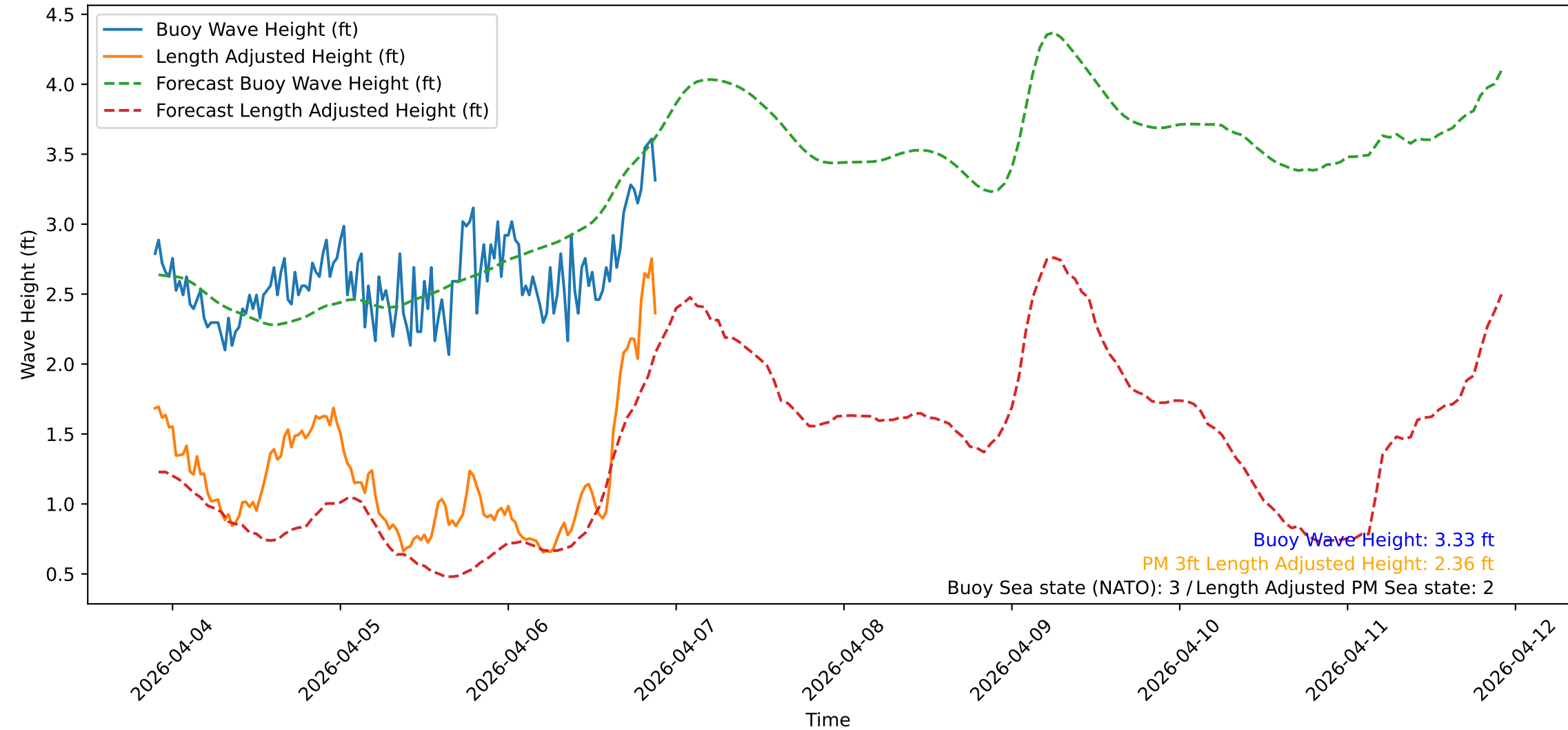
Wave Heights over Time for Oceanside Harbor at 2026-04-06 21:40:32
